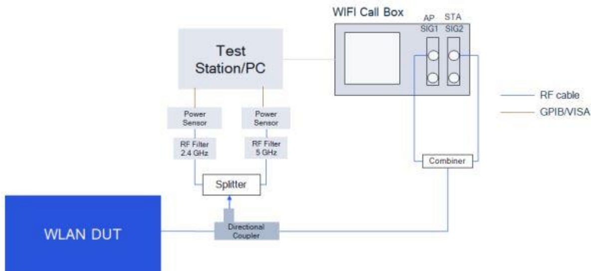
Figure 4-4 SISO (Simultaneous Transmission) – Validation test setup
