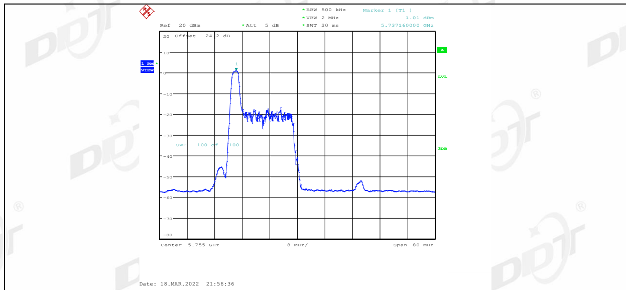
11AX40MIMO Ant2 5755 26Tone RU8
