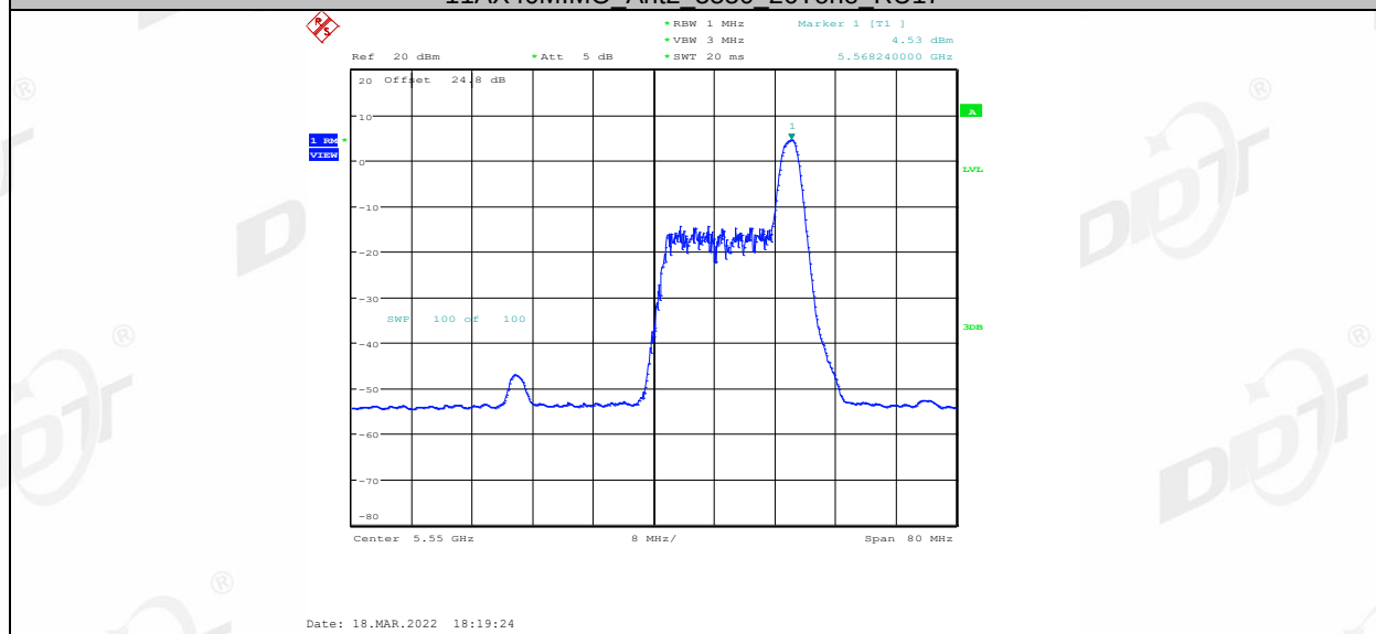
11AX40MIMO Ant2 5550 52Tone RU37
