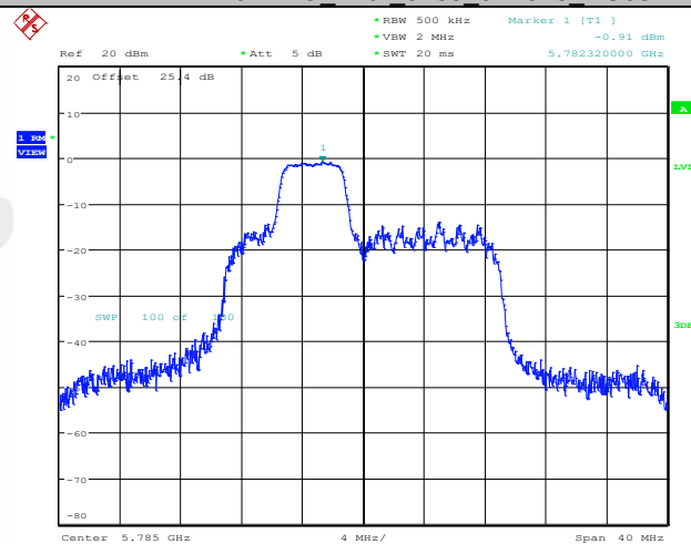
11AX20MIMO Ant2 5785 52Tone RU38
