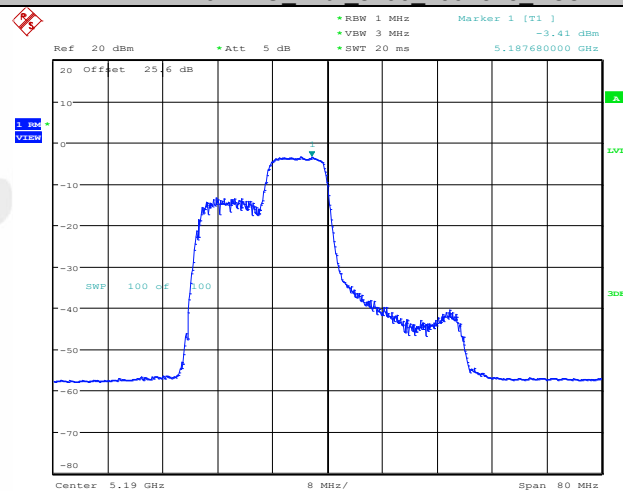
11AX40MIMO Ant2 5190 106Tone RU54
