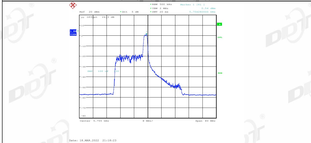
11AX40MIMO Ant1 5755 26Tone RU17
