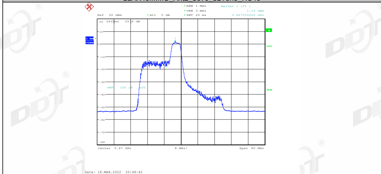
11AX40MIMO Ant2 5670 52Tone RU44
