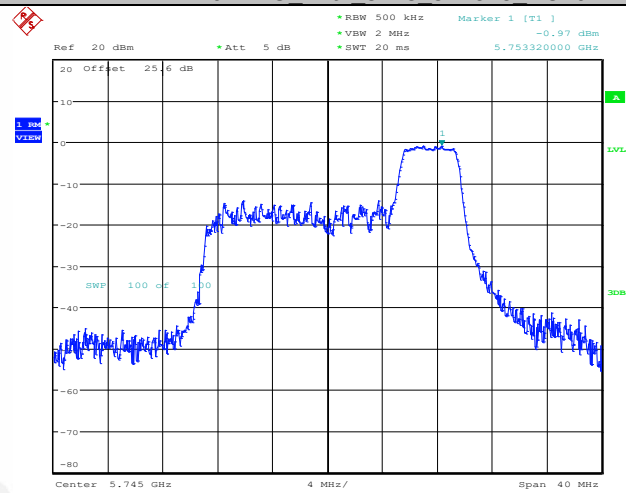
11AX20MIMO Ant2 5745 52Tone RU40
