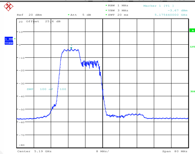
11AX40MIMO Ant2 5190 106Tone RU53
