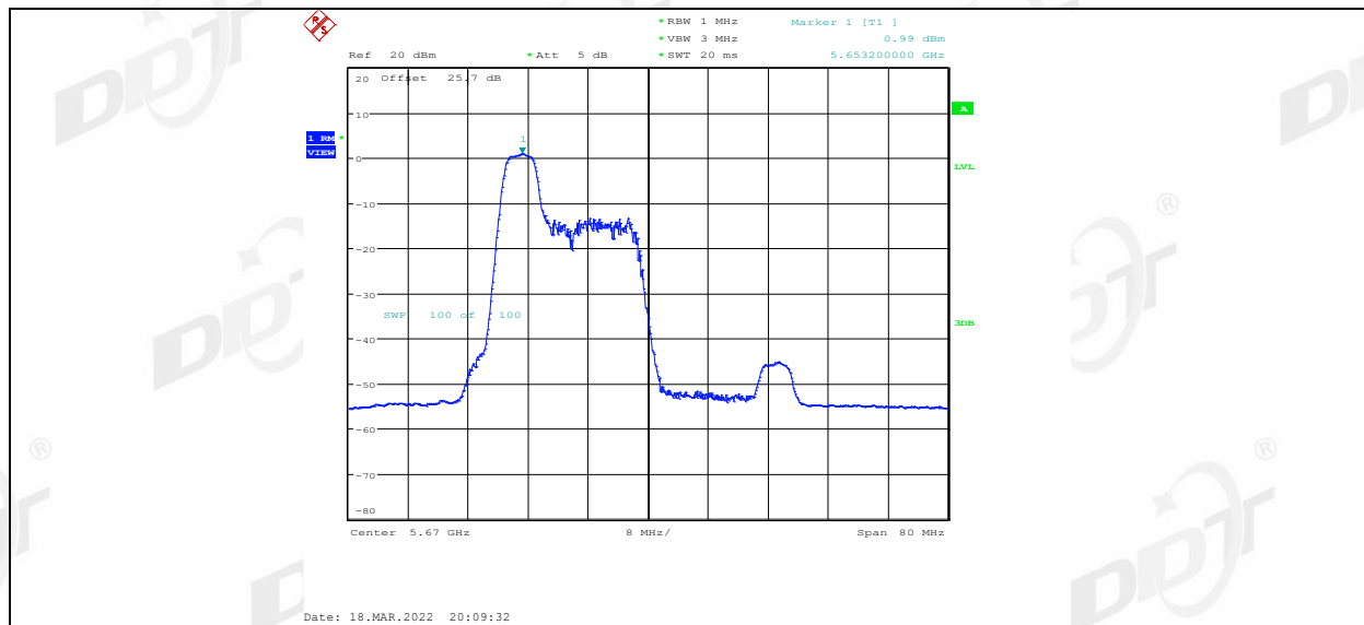
11AX40MIMO Ant1 5670 52Tone RU40
