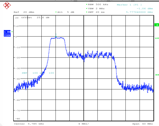
11AX20MIMO Ant2 5785 52Tone RU37
