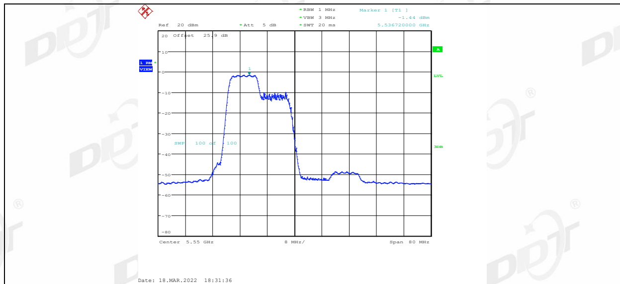
11AX40MIMO Ant2 5550 106Tone RU54
