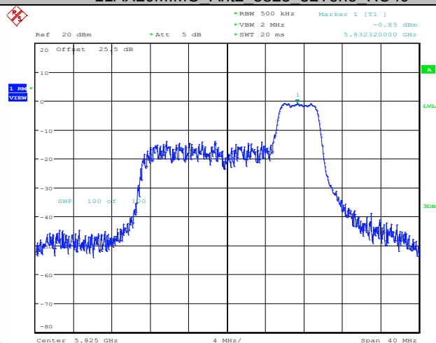
11AX20MIMO Ant2 5825 52Tone RU40
