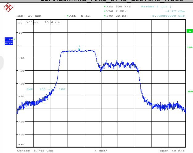
11AX20MIMO Ant2 5745 106Tone RU53
