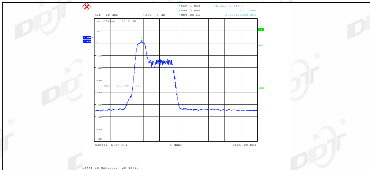
11AX40MIMO Ant2 5670 52Tone RU40
