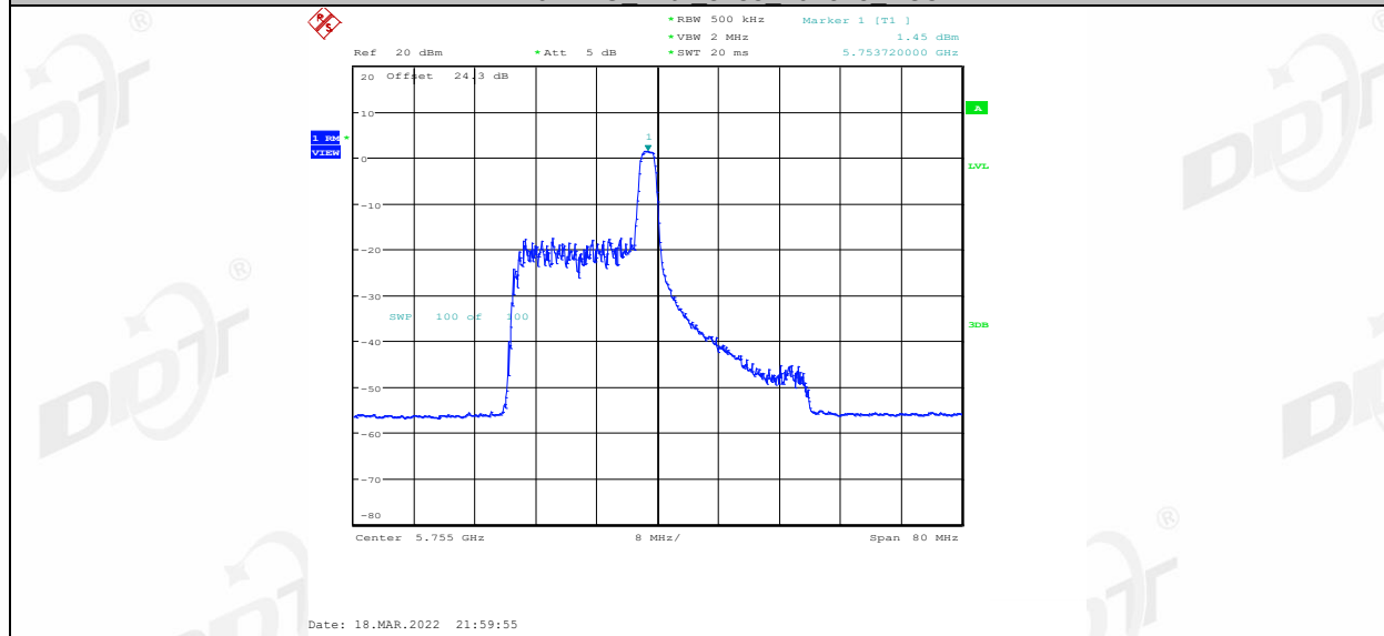
11AX40MIMO Ant2 5755 26Tone RU17
