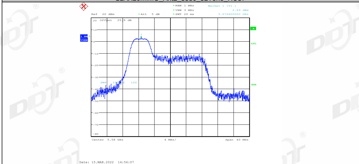
11AX20MIMO Ant2 5580 52Tone RU38
