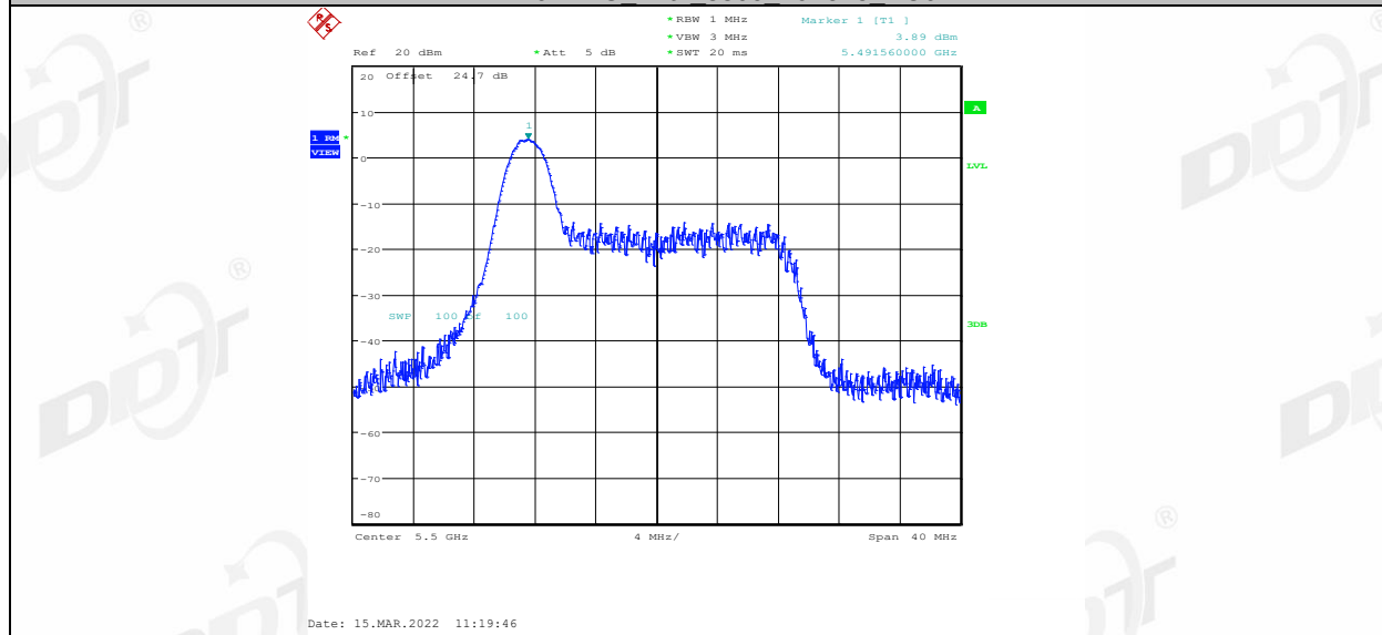
11AX20MIMO Ant2 5500 26Tone RU4
