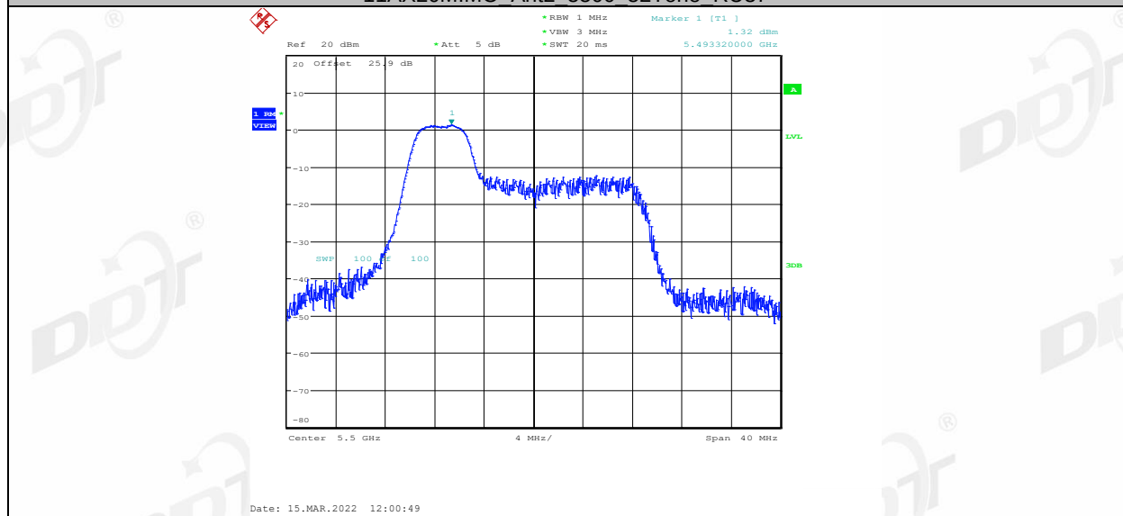
11AX20MIMO Ant2 5500 52Tone RU38
