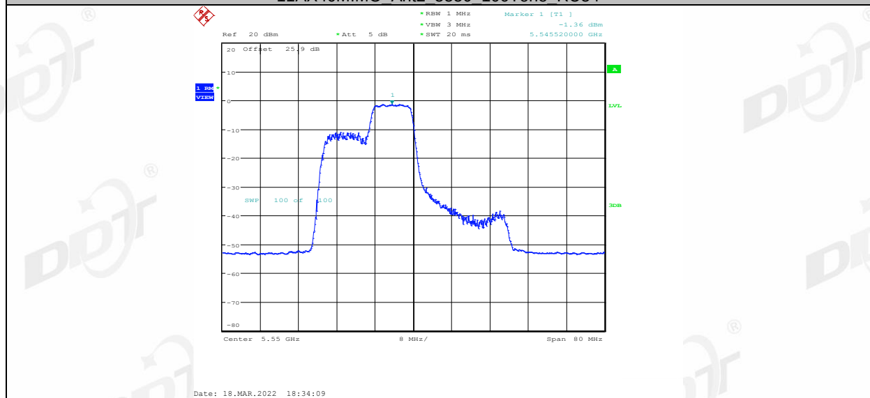
11AX40MIMO Ant2 5550 106Tone RU55
