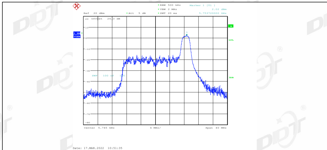
11AX20MIMO Ant2 5745 52Tone RU37
