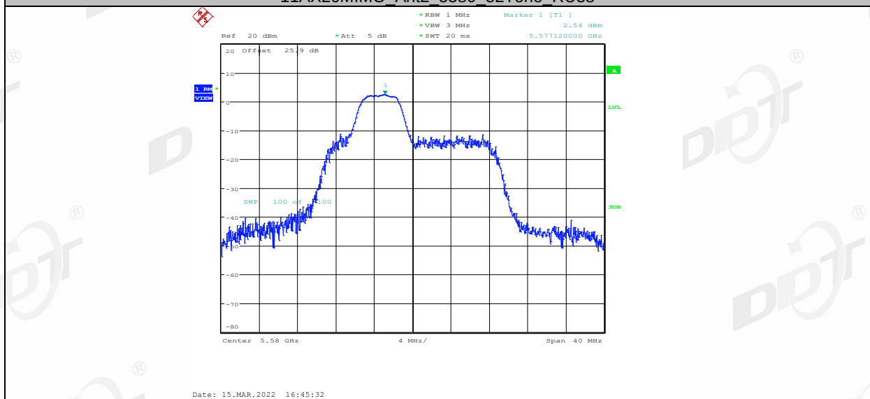
11AX20MIMO Ant2 5580 52Tone RU39
