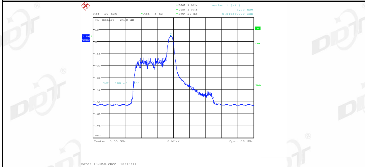
11AX40MIMO Ant2 5550 26Tone RU17
