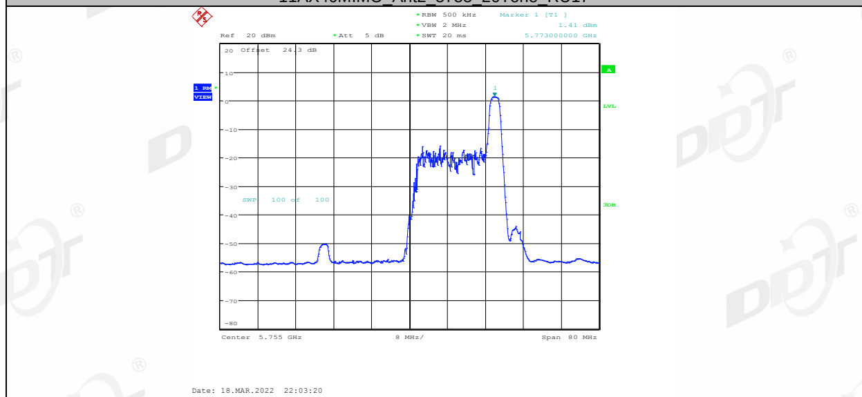
11AX40MIMO Ant2 5755 52Tone RU37
