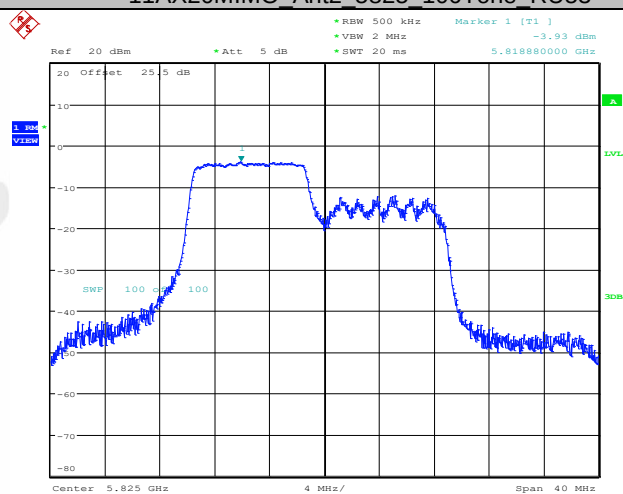
11AX20MIMO Ant2 5825 106Tone RU53
