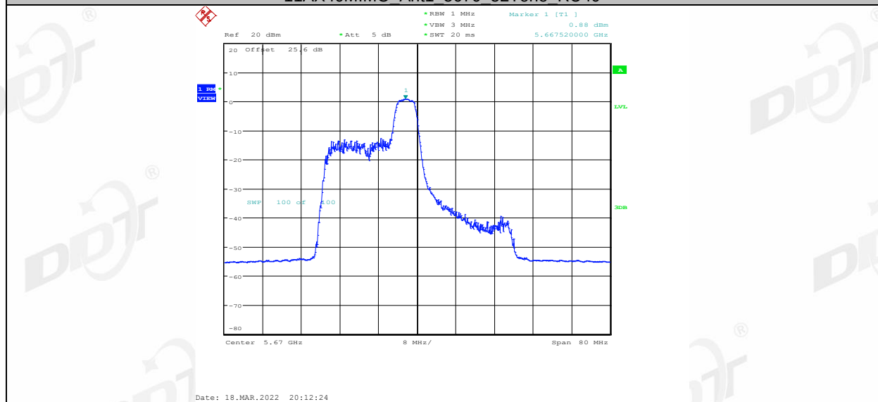
11AX40MIMO Ant1 5670 52Tone RU44
