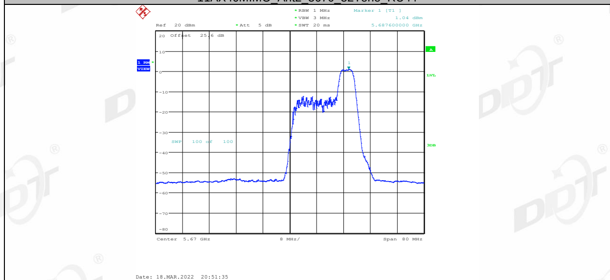
11AX40MIMO Ant2 5670 106Tone RU53
