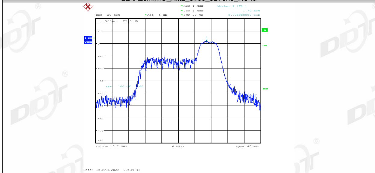
11AX20MIMO Ant2 5700 106Tone RU53
