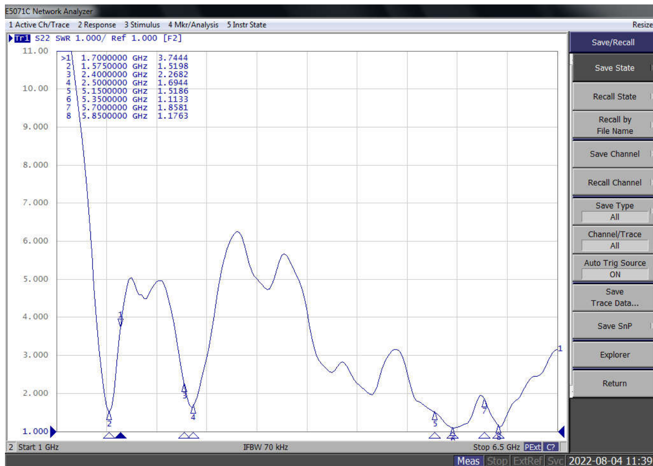
ANT22# VSWR
