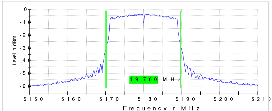
26 dB Bandwidth
