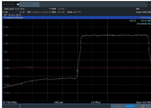
Plot 8-22. Band Edge Emission Plot (NR_n13_1C_5M_256QAM - Low Band Edge, Port 2)
