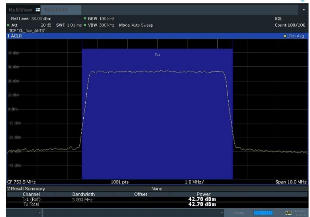
Plot 8-10. Conducted Average Output Power Plot (NR_n13_1C_5M_64QAM - High Channel, Port 3)
