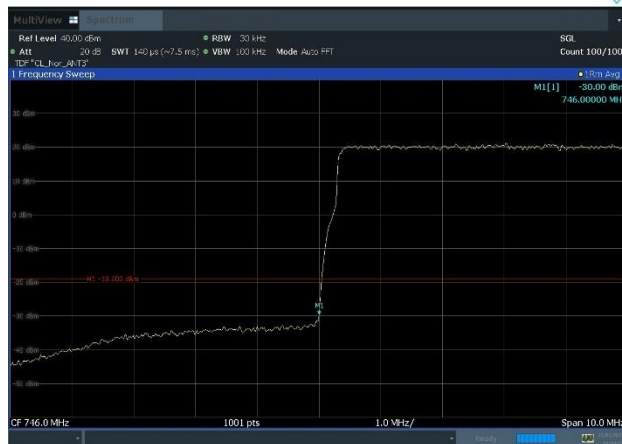
Plot 8-24. Band Edge Emission Plot (NR_n13_1C_10M_QPSK - Low Band Edge, Port 3)
