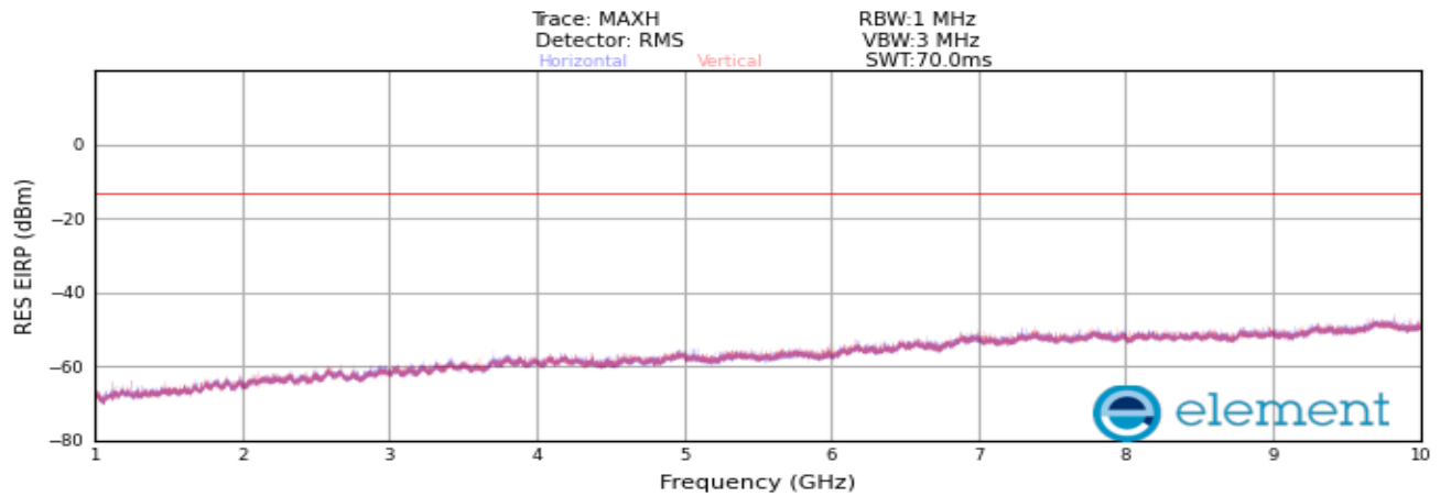
Plot 8-68. Radiated spurious emission_1 GHz to 10 GHz (Multi band_NR_n13_1C_10M+LTE B5_1C_20M_Mid Channel)
