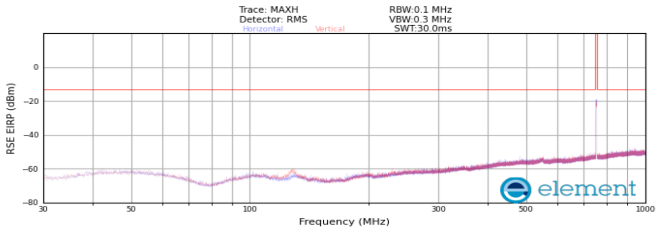
Plot 8-61. Radiated spurious emission 30 MHz to 1000 MHz (NR_n13_1C_5M_High Channel)
