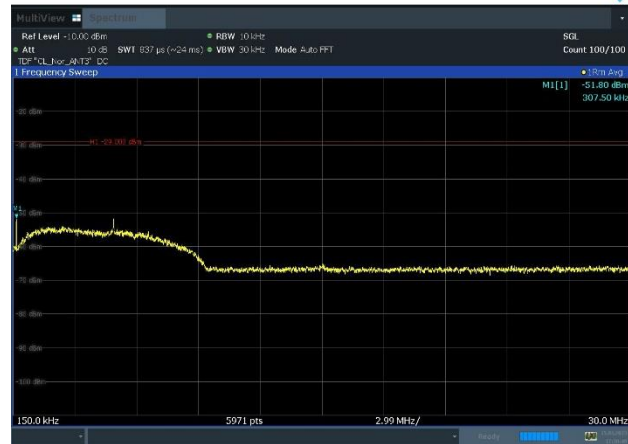
Plot 8-43. Conducted Spurious Emission Plot 150 kHz to 30 MHz (NR_n13_2C_5M+5M_QPSK - Mid Channel, Port 3)
