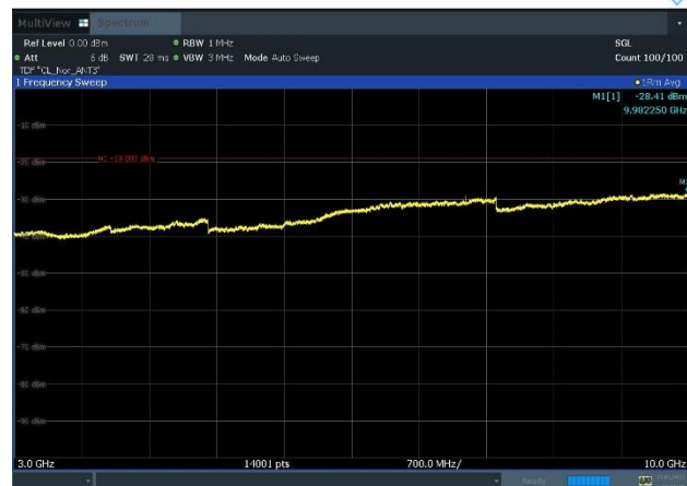
Plot 8-41. Conducted Spurious Emission Plot 3 GHz to 10 GHz (NR_n13_1C_10M_64QAM - Mid Channel, Port 3)
