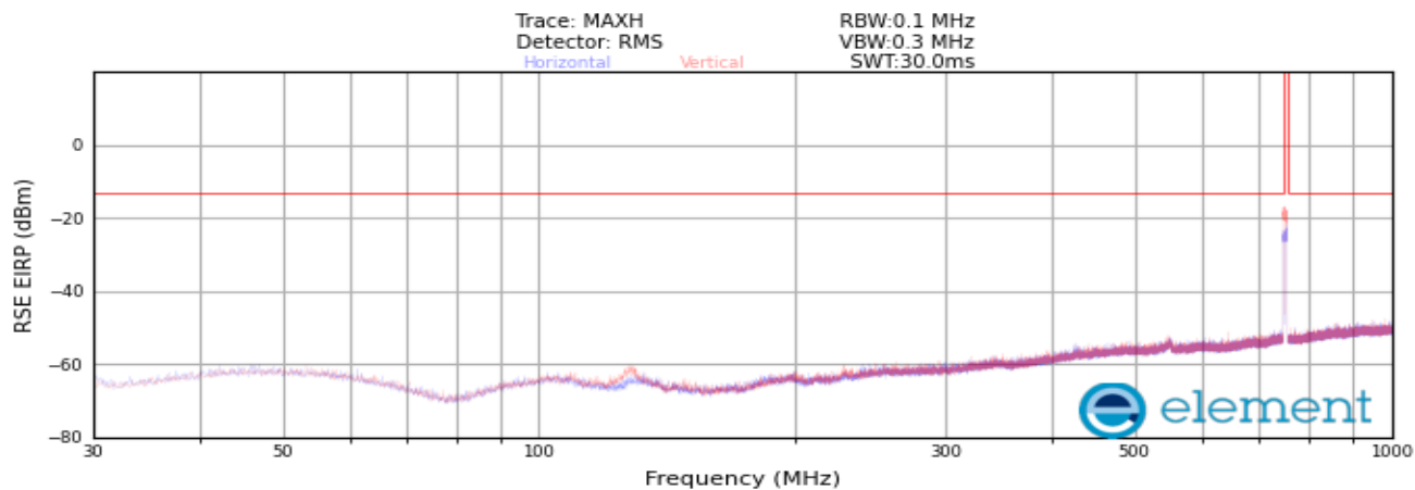
Plot 8-65. Radiated spurious emission_30 MHz to 1000 MHz (NR_n13_2C_5M+5M_Mid Channel)
