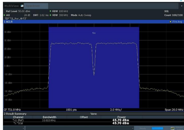
Plot 8-18. Conducted Average Output Power Plot (NR_n13_2C_5M+5M_16QAM - Mid Channel, Port 3)
