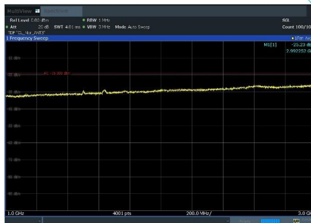
Plot 8-53. Conducted Spurious Emission Plot 1 GHz to 3 GHz (Multi band_NR_n13_1C_10M+LTE B5_1C_20M_QPSK - Mid Channel, Port 3)
