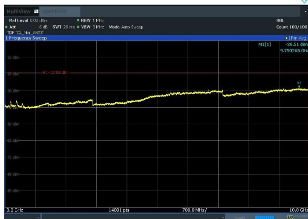
Plot 8-54. Conducted Spurious Emission Plot 3 GHz to 10 GHz (Multi band_NR_n13_1C_10M+LTE B5_1C_20M_QPSK - Mid Channel, Port 3)
