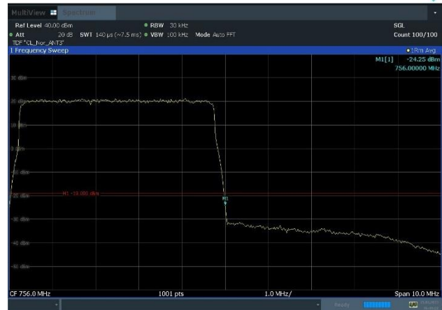
Plot 8-23. Band Edge Emission Plot (n13_1C_5M_16QAM - High Band Edge, Port 3)
