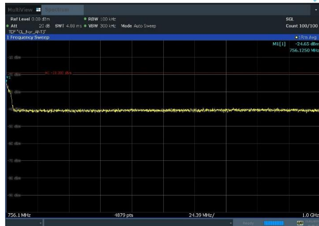
Plot 8-33. Conducted Spurious Emission Plot 756.1 MHz to 1 GHz (NR_n13_1C_5M_16QAM - High Channel, Port 3)
