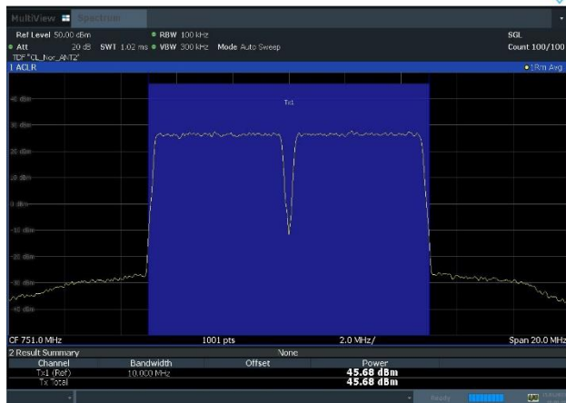
Plot 8-17. Conducted Average Output Power Plot (NR_n13_2C_5M+5M_16QAM - Mid Channel, Port 2)
