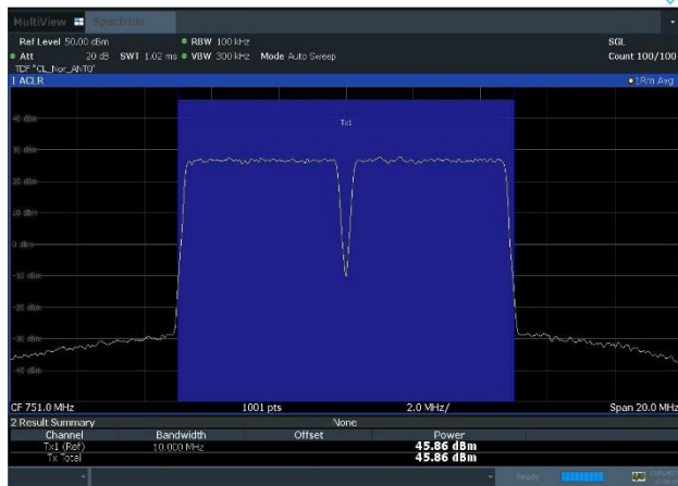
Plot 8-15. Conducted Average Output Power Plot (NR_n13_2C_5M+5M_16QAM - Mid Channel, Port 0)
