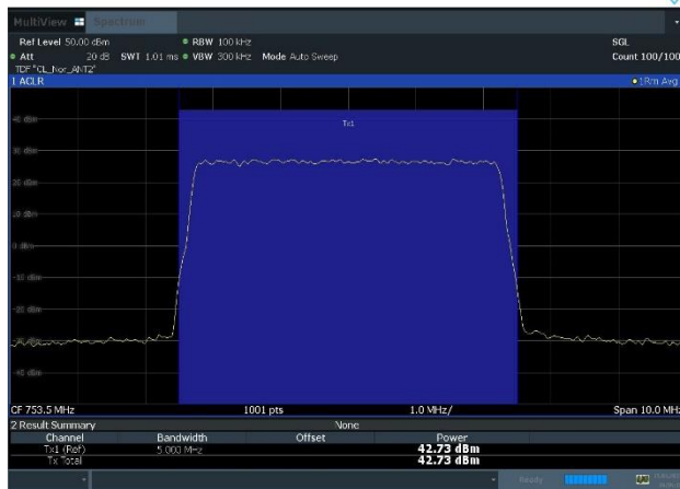
Plot 8-9. Conducted Average Output Power Plot (NR_n13_1C_5M_64QAM - High Channel, Port 2)
