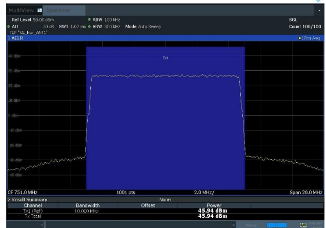
Plot 8-12. Conducted Average Output Power Plot (NR_n13_1C_10M_256QAM - Mid Channel, Port 1)
