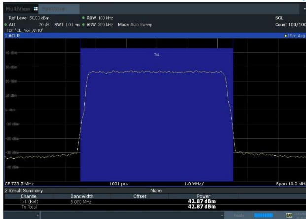
Plot 8-7. Conducted Average Output Power Plot (NR_n13_1C_5M_64QAM - High Channel, Port 0)
