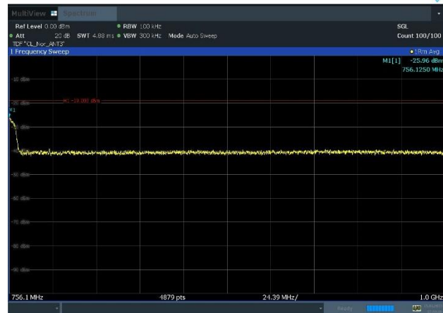
Plot 8-45. Conducted Spurious Emission Plot 756.1 MHz to 1 GHz (NR_n13_2C_5M+5M_QPSK - Mid Channel, Port 3)
