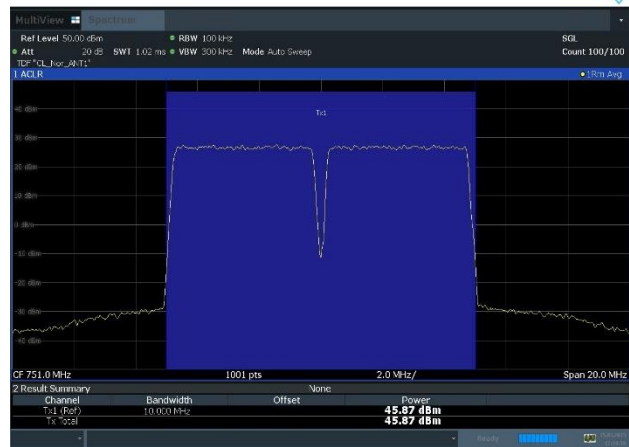
Plot 8-16. Conducted Average Output Power Plot (NR_n13_2C_5M+5M_16QAM - Mid Channel, Port 1)
