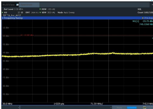
Plot 8-38. Conducted Spurious Emission Plot 30 MHz to 745.9 MHz (NR_n13_1C_10M_64QAM - Mid Channel, Port 3)
