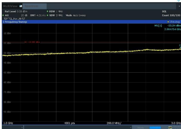
Plot 8-34. Conducted Spurious Emission Plot 1 GHz to 3 GHz (NR_n13_1C_5M_16QAM - High Channel, Port 3)
