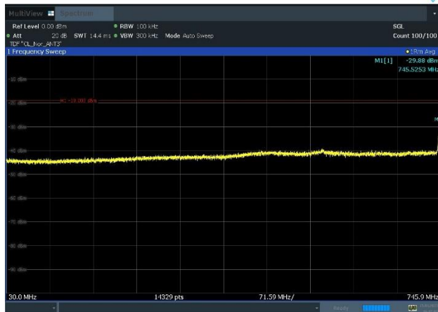
Plot 8-32. Conducted Spurious Emission Plot 30 MHz to 745.9 MHz (NR_n13_1C_5M_16QAM - High Channel, Port 3)
