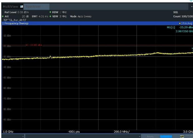
Plot 8-40. Conducted Spurious Emission Plot 1 GHz to 3 GHz (NR_n13_1C_10M_64QAM - Mid Channel, Port 3)
