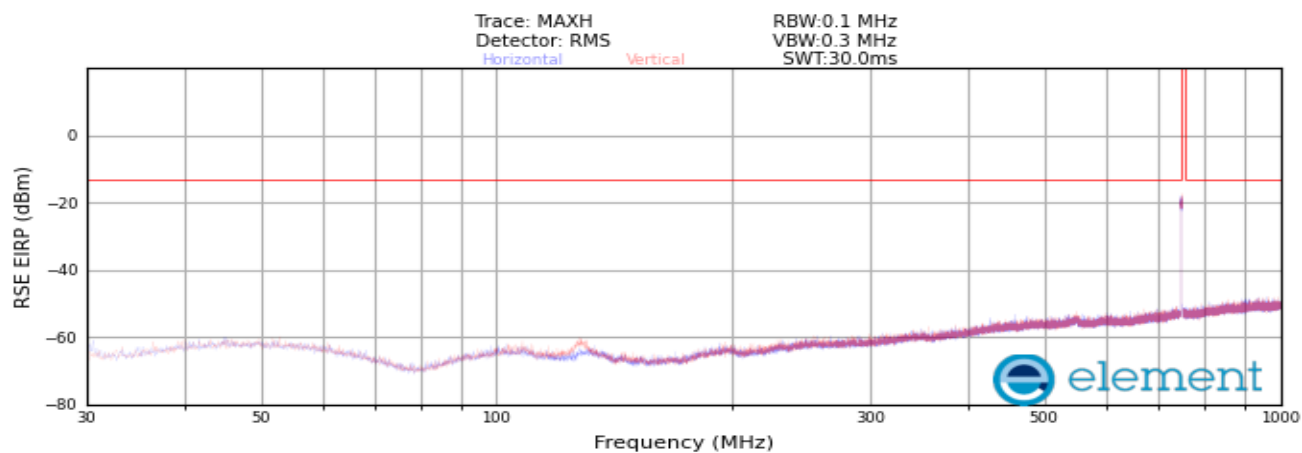
Plot 8-59. Radiated spurious emission_30 MHz to 1000 MHz (NR_n13_1C_5M_Low Channel)
