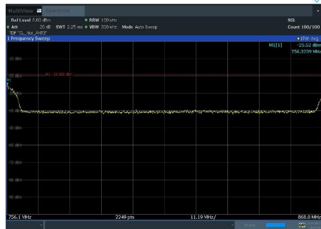
Plot 8-51. Conducted Spurious Emission Plot 756.1 MHz to 868 MHz (Multi band_NR_n13_1C_10M+LTE B5_1C_20M_QPSK - Mid Channel, Port 3)
