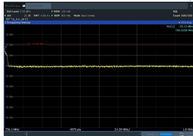
Plot 8-39. Conducted Spurious Emission Plot 756.1 MHz to 1 GHz (NR_n13_1C_10M_64QAM - Mid Channel, Port 3)
