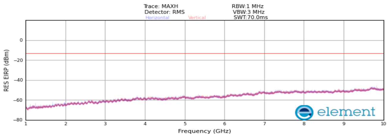
Plot 8-62. Radiated spurious emission_1 GHz to 10 GHz (NR_n13_1C_5M_High Channel)
