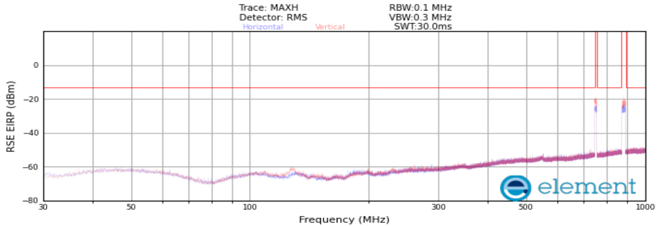
Plot 8-67. Radiated spurious emission_30 MHz to 1000 MHz (Multi band_NR_n13_1C_10M+LTE B5_1C_20M_Mid Channel)
