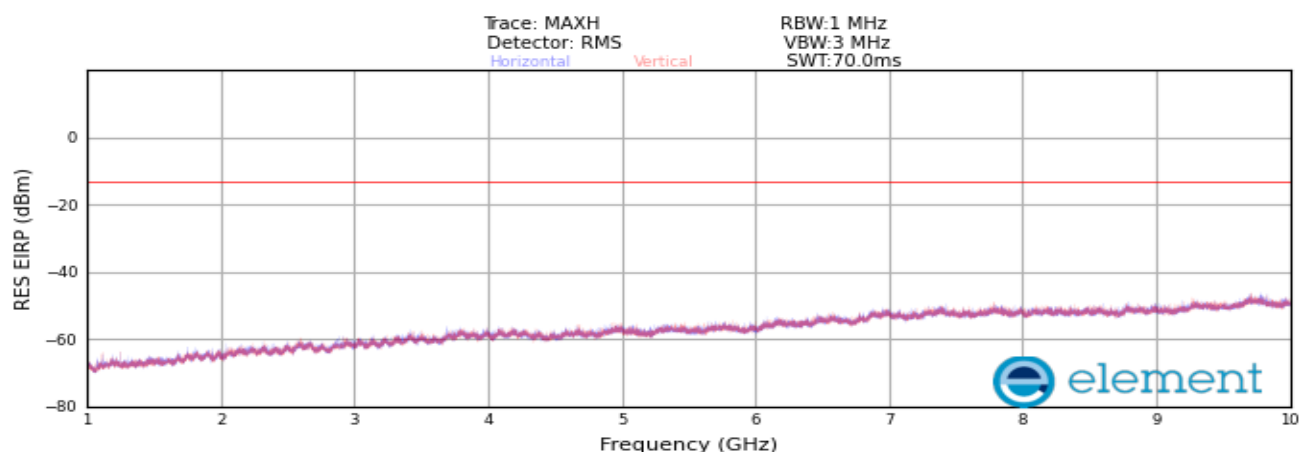
Plot 8-60. Radiated spurious emission_1 GHz to 10 GHz (NR_n13_1C_5M_Low Channel)
