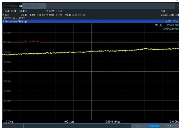
Plot 8-46. Conducted Spurious Emission Plot 1 GHz to 3 GHz (NR_n13_2C_5M+5M_QPSK - Mid Channel, Port 3)
