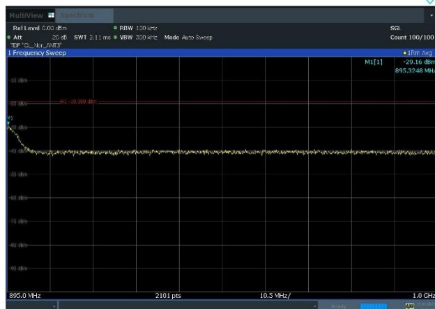
Plot 8-52. Conducted Spurious Emission Plot 895 MHz to 1 GHz (Multi band_NR_n13_1C_10M+LTE B5_1C_20M_QPSK - Mid Channel, Port 3)
