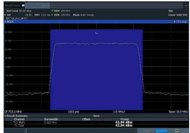
Plot 8-8. Conducted Average Output Power Plot (NR_n13_1C_5M_64QAM - High Channel, Port 1)
