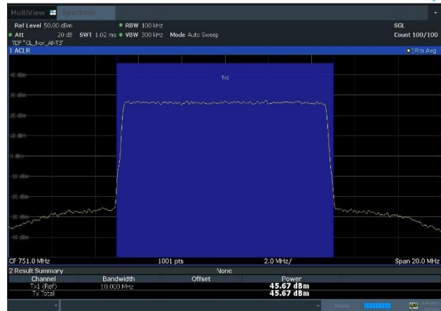
Plot 8-14. Conducted Average Output Power Plot (NR_n13_1C_10M_256QAM - Mid Channel, Port 3)
