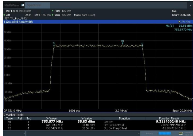
Plot 8-4. Occupied Bandwidth Plot (NR_n13_1C_10M_16QAM - Mid Channel, Port 2)
