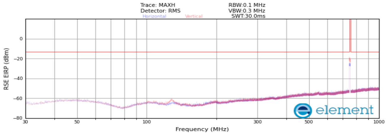
Plot 8-63. Radiated spurious emission 30 MHz to 1000 MHz (NR_n13_1C_10M_Mid Channel)
