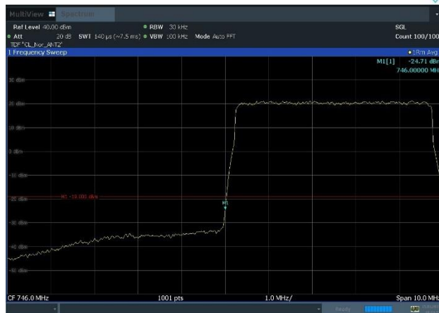
Plot 8-26. Band Edge Emission Plot (NR_n13_2C_5M+5M_QPSK - Low Band Edge, Port 2)
