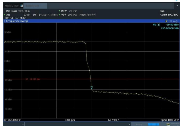
Plot 8-25. Band Edge Emission Plot (NR_n13_1C_10M_64QAM - High Band Edge, Port 3)
