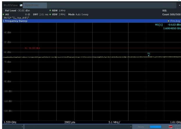
Plot 8-55. Conducted Spurious Emission Plot 1.559 GHz to 1.61 GHz (NR_n13_1C_5M_QPSK - High Channel, Port 0)
