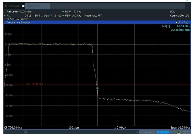
Plot 8-27. Band Edge Emission Plot (NR_n13_2C_5M+5M_QPSK - High Band Edge, Port 2)
