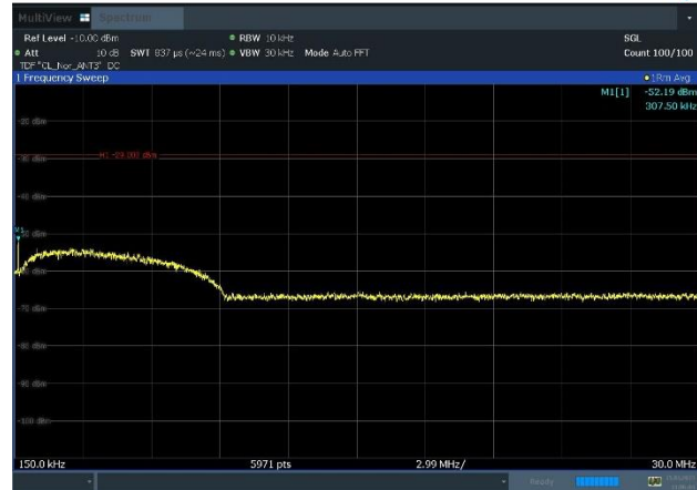
Plot 8-37. Conducted Spurious Emission Plot 150 kHz to 30 MHz (NR_n13_1C_10M_64QAM - Mid Channel, Port 3)
