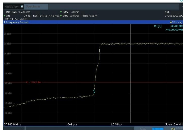
Plot 8-28. Band Edge Emission Plot (Multi band_NR_n13_1C_10M+LTE B5_1C_20M_QPSK - Low Band Edge, Port 3)
