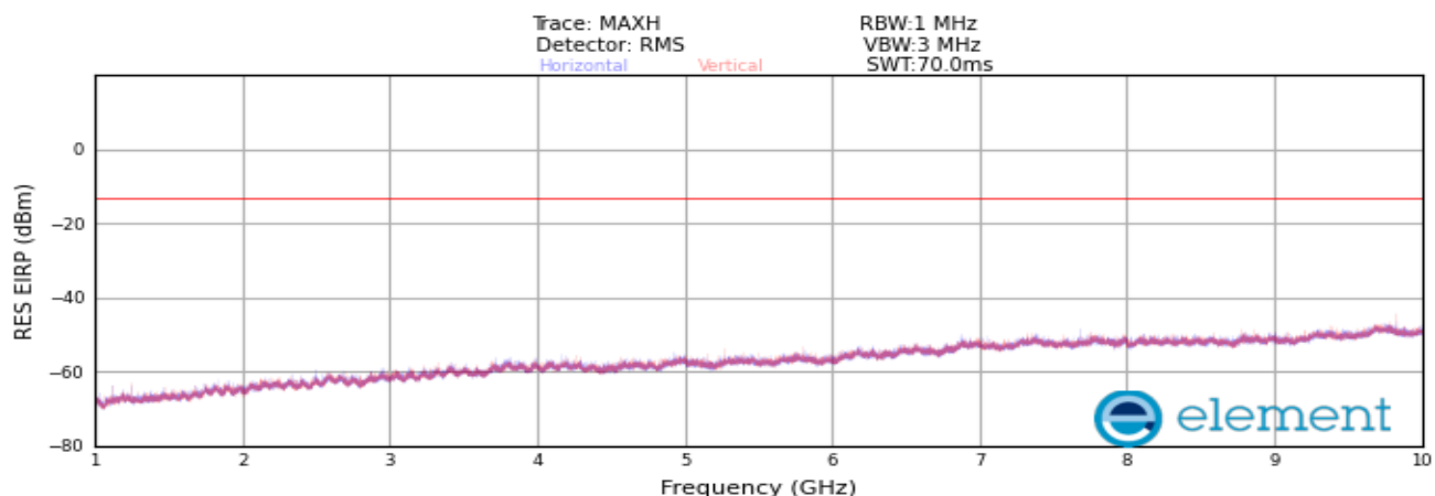
Plot 8-66. Radiated spurious emission_1 GHz to 10 GHz (NR_n13_2C_5M+5M_Mid Channel)
