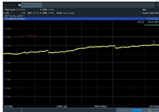
Plot 8-47. Conducted Spurious Emission Plot 3 GHz to 10 GHz (NR_n13_2C_5M+5M_QPSK - Mid Channel, Port 3)
