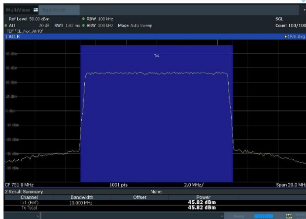
Plot 8-11. Conducted Average Output Power Plot (NR_n13_1C_10M_256QAM - Mid Channel, Port 0)
