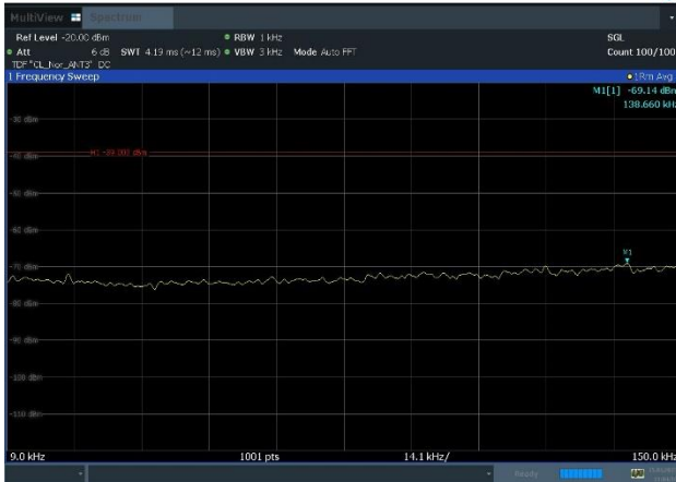
Plot 8-36. Conducted Spurious Emission Plot 9 kHz to 150 kHz (NR_n13_1C_10M_64QAM - Mid Channel, Port 3)
