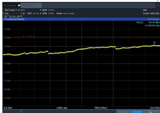
Plot 8-35. Conducted Spurious Emission Plot 3 GHz to 10 GHz (NR_n13_1C_5M_16QAM - High Channel, Port 3)
