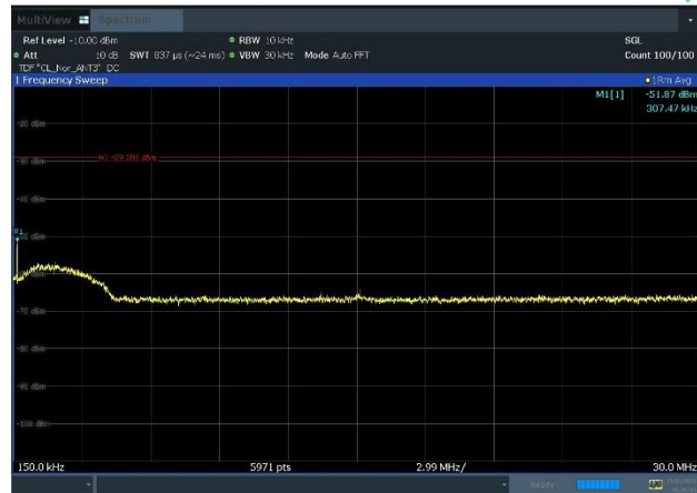
Plot 8-31. Conducted Spurious Emission Plot 150 kHz to 30 MHz (NR_n13_1C_5M_16QAM - High Channel, Port 3)
