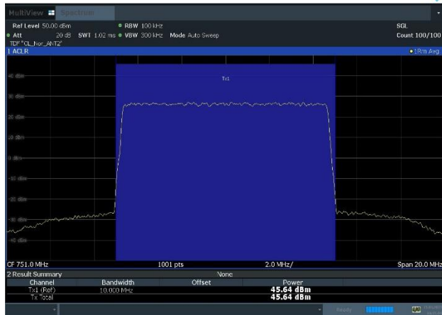
Plot 8-13. Conducted Average Output Power Plot (NR_n13_1C_10M_256QAM - Mid Channel, Port 2)
