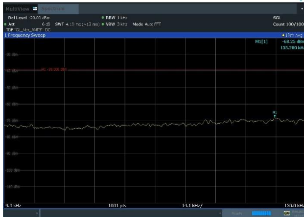
Plot 8-48. Conducted Spurious Emission Plot 9 kHz to 150 kHz (Multi band_NR_n13_1C_10M+LTE B5_1C_20M_QPSK - Mid Channel, Port 3)
