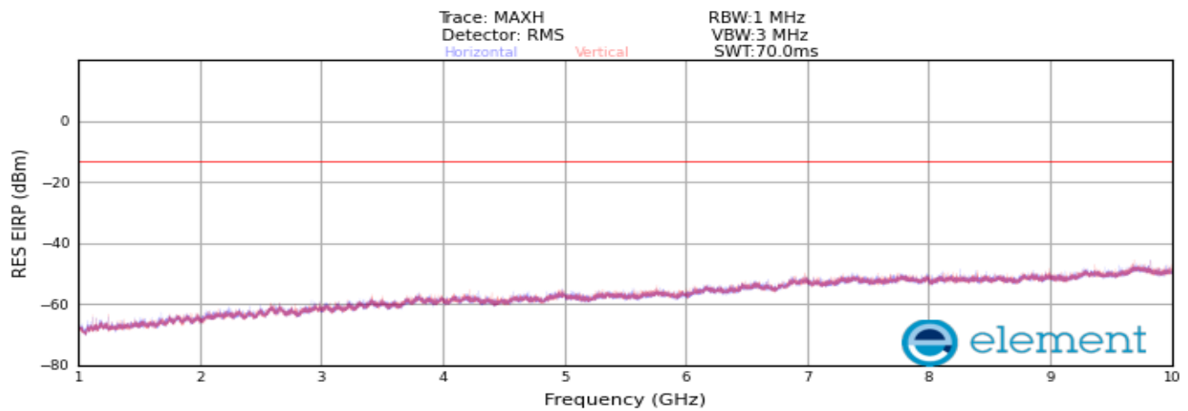
Plot 8-64. Radiated spurious emission 1 GHz to 10 GHz (NR_n13_1C_10M_Mid Channel)
