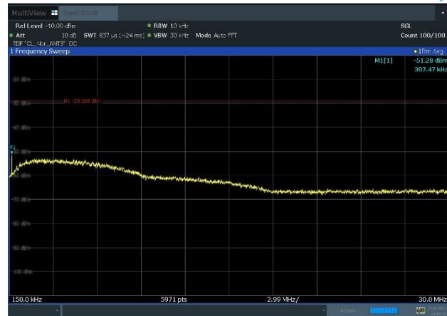
Plot 8-49. Conducted Spurious Emission Plot 150 kHz to 30 MHz (Multi band_NR_n13_1C_10M+LTE B5_1C_20M_QPSK - Mid Channel, Port 3)
