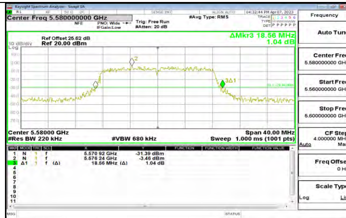
11A-CDD Ant2 5580
