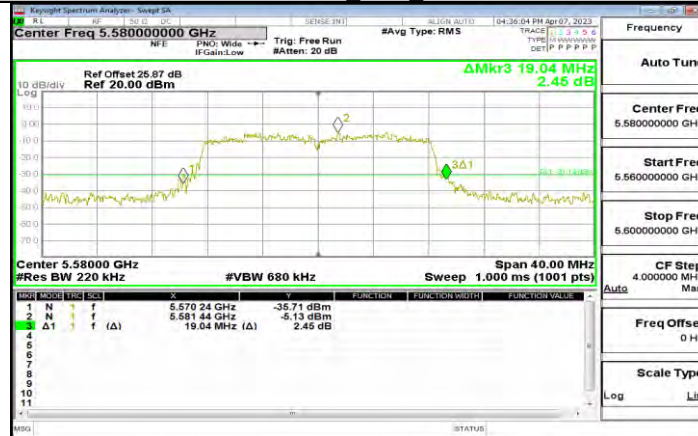
11A-CDD Ant4 5580
