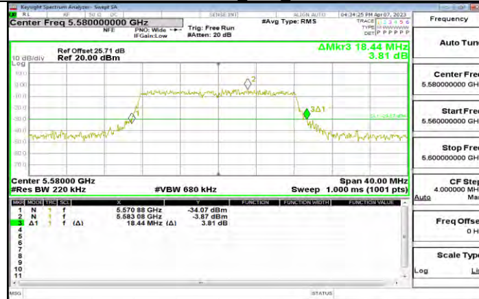
11A-CDD Ant3 5580
