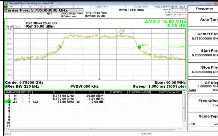
11A-CDD Ant2 5785
