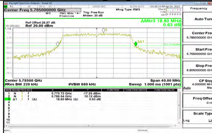
11A-CDD Ant15 5785
