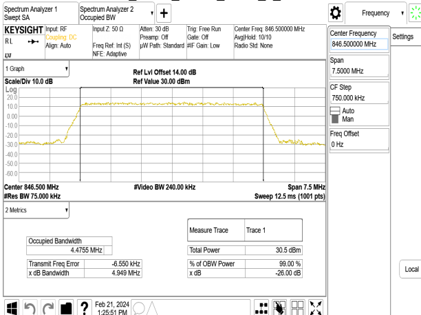
Band5_5MHz_QPSK_RB25_0_CH20625
