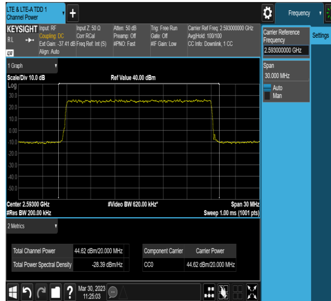
Band41-20MHz-64QAM-Highest-E-TM3.1-20
