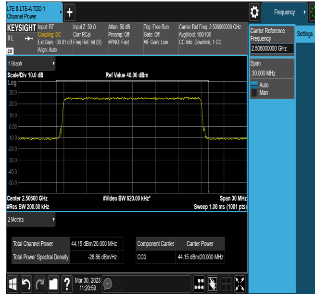
Band41-20MHz-64QAM-Middle-E-TM3.1-20
