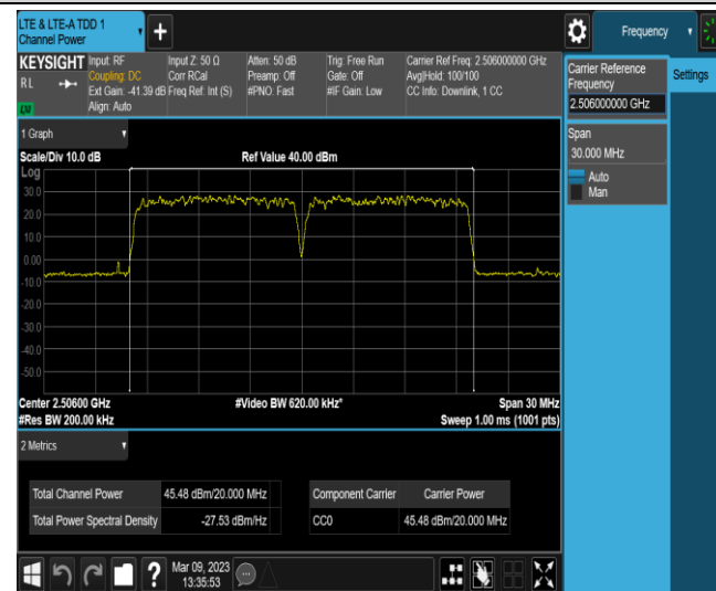
Band41-20MHz-256QAM-Middle-E-TM3.1A-20
