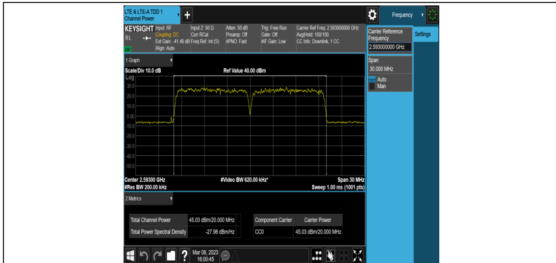
Band41-20MHz-QPSK-Highest-E-TM1.1-20
