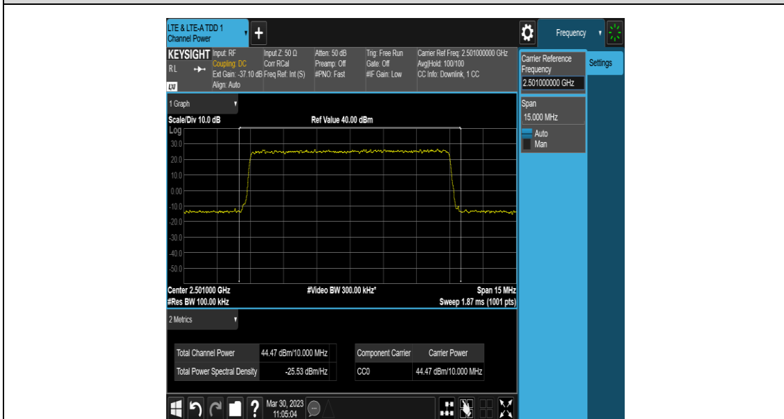
Band41-10MHz-64QAM-Lowest-E-TM3.1-10
