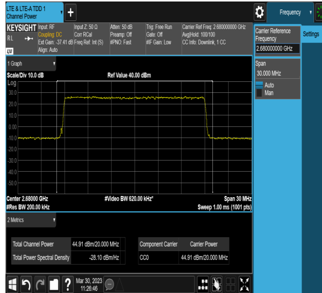
Band41-20MHz-QPSK-Highest-E-TM1.1-20
