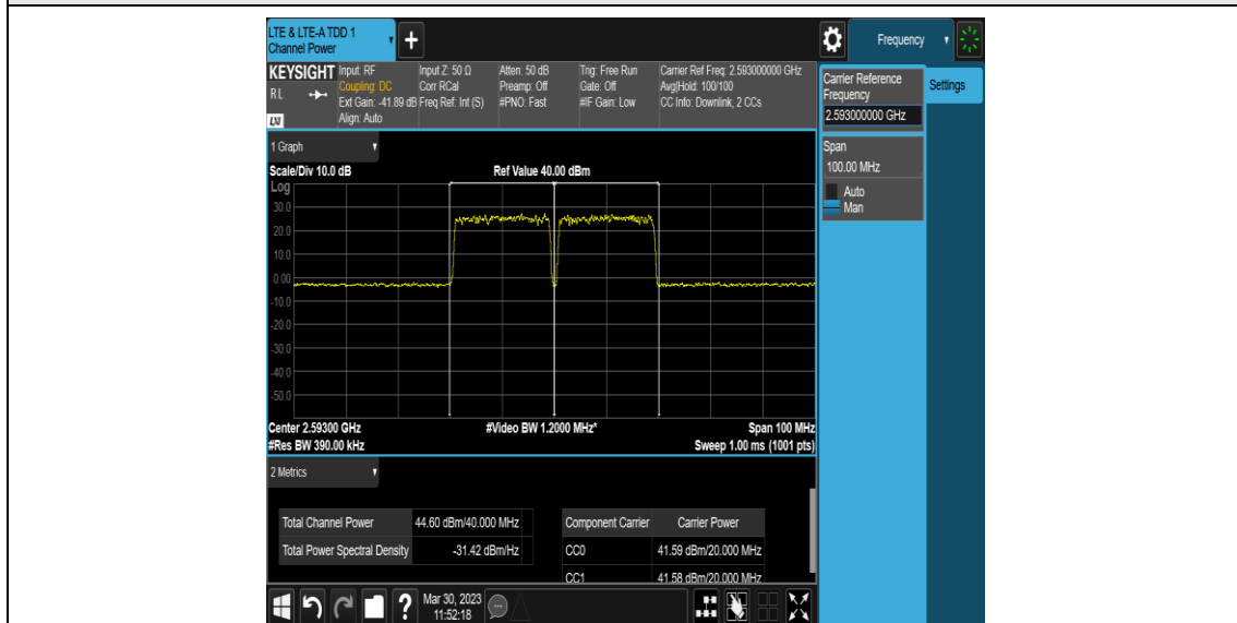
Band41-40MHz-64QAM-Highest-E-TM3.1-40
