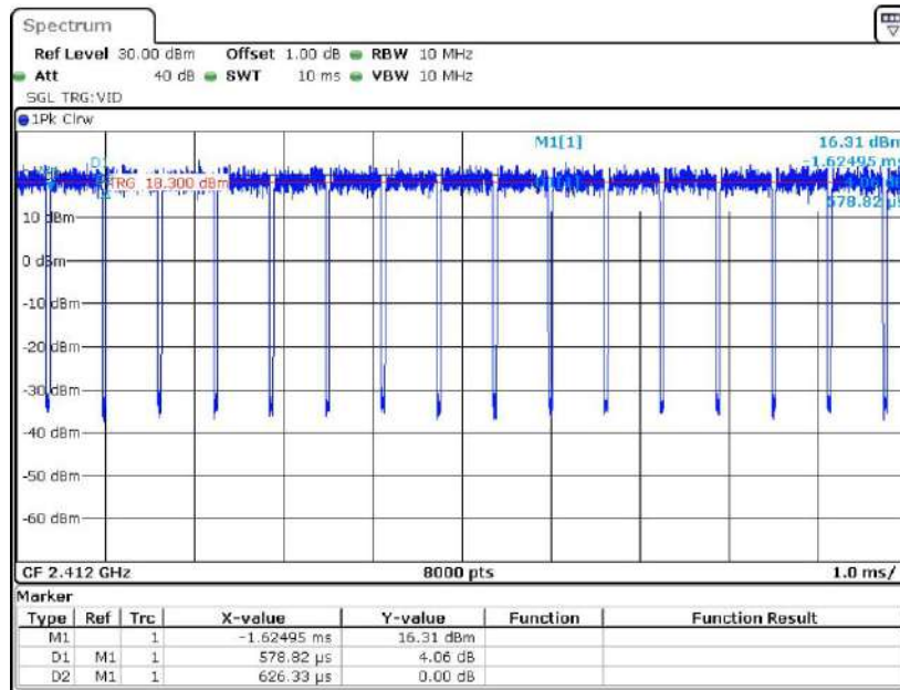
11AX20SISO-242T_Ant1_2412
