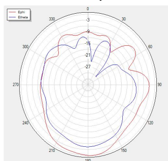
H Theta=90 freq=2450MHz
