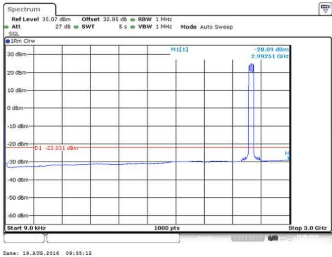
Figure 185 Spurious Emissions (9kHz – 3GHz) – 64QAM (2573/ 2593/ 2613 MHz) (3 X 20 MHz Channel BW)
