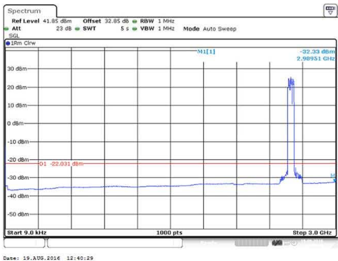
Figure 213 Spurious Emissions (9kHz – 3GHz) – 16QAM (2573/ 2593/ 2613 MHz) (3 X 20 MHz Channel BW)
