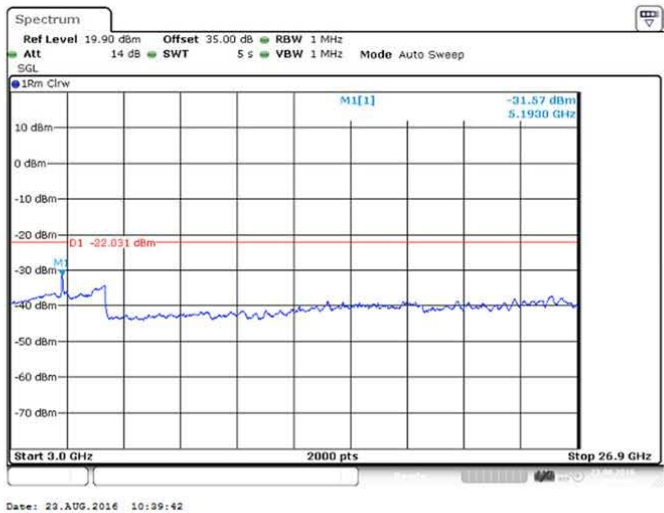
Figure 214 Spurious Emissions (3GHz – 26.900GHz) – 16QAM (2573/ 2593/ 2613 MHz) (3 X 20 MHz Channel BW)
