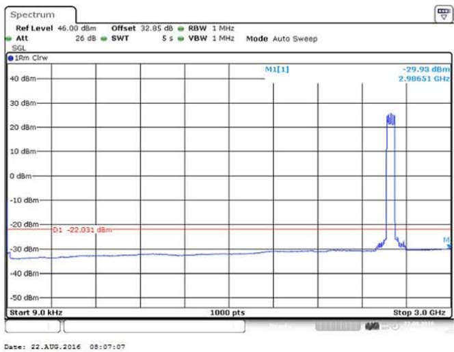
Figure 229 Spurious Emissions (9kHz – 3GHz) – QPSK (2573/ 2593/ 2613 MHz) (3 X 20 MHz Channel BW)
