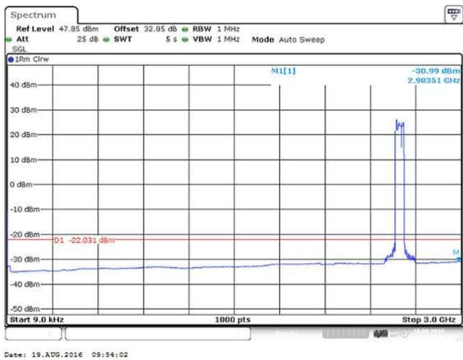
Figure 189 Spurious Emissions (9kHz – 3GHz) – 16QAM (2573/ 2593/ 2613 MHz) (3 X 20 MHz Channel BW)
