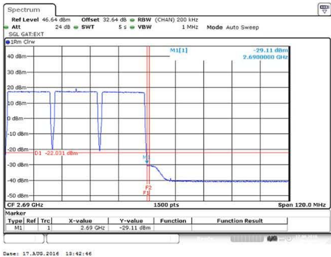
Figure 208 Spurious Emissions (Upper Band Edge) – 64QAM (2640/ 2660/ 2680 MHz) (3 X 20 MHz Channel BW)
