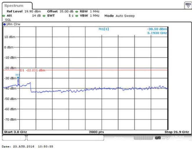
Figure 222 Spurious Emissions (3GHz – 26.900GHz) – 64QAM (2573/ 2593/ 2613 MHz) (3 X 20 MHz Channel BW)
