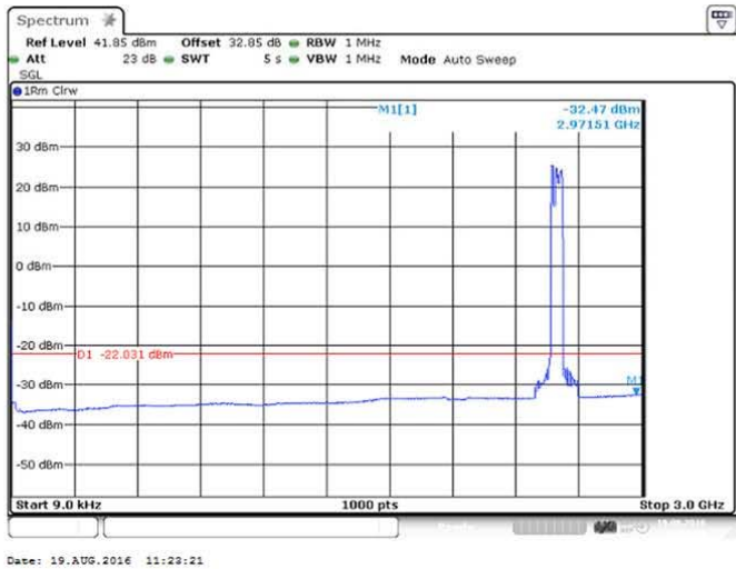
Figure 205 Spurious Emissions (9kHz – 3GHz) – QPSK (2573/ 2593/ 2613 MHz) (3 X 20 MHz Channel BW)
