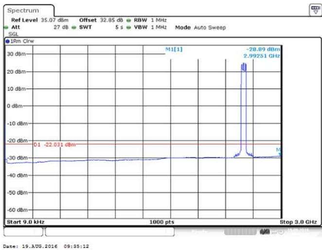
Figure 173 Spurious Emissions (9kHz – 3GHz) – 64QAM (2573/ 2593/ 2613 MHz) (3 X 20 MHz Channel BW)
