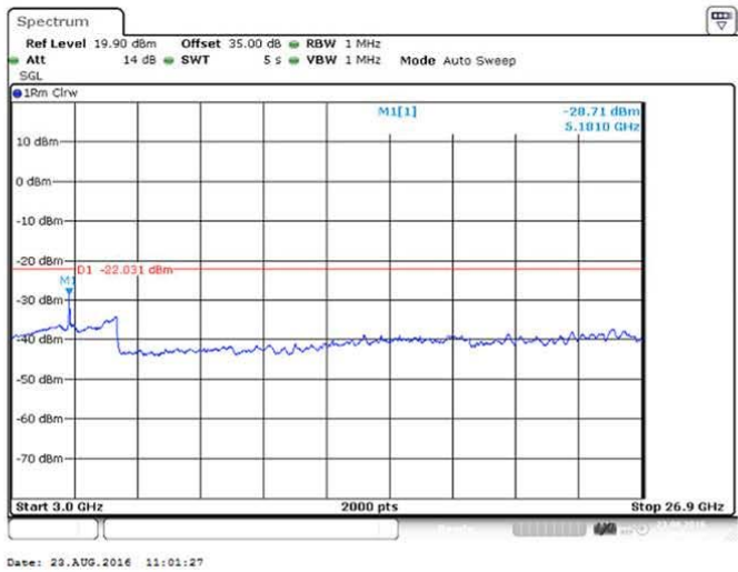
Figure 230 Spurious Emissions (3GHz – 26.900GHz) – QPSK (2573.0/2593/2613.0 MHz) (3 X 20 MHz Channel BW)
