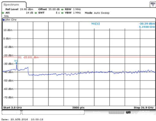
Figure 186 Spurious Emissions (3GHz – 26.900GHz) – 64QAM (2573/ 2593/ 2613 MHz) (3 X 20 MHz Channel BW)
