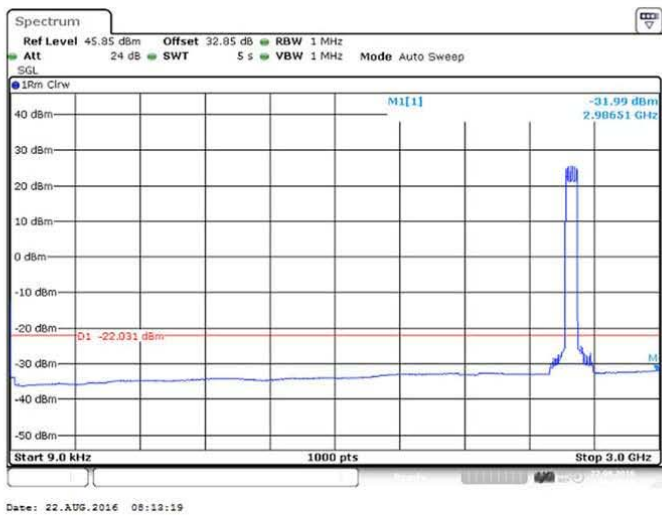
Figure 233 Spurious Emissions (9kHz – 3GHz) – 64QAM (2573/ 2593/ 2613 MHz) (3 X 20 MHz Channel BW)
