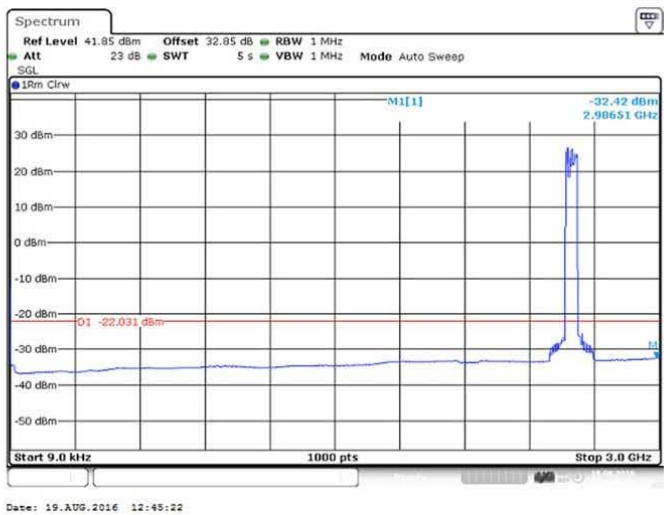
Figure 225 Spurious Emissions (9kHz – 3GHz) – 16QAM (2573/ 2593/ 2613 MHz) (3 X 20 MHz Channel BW)
