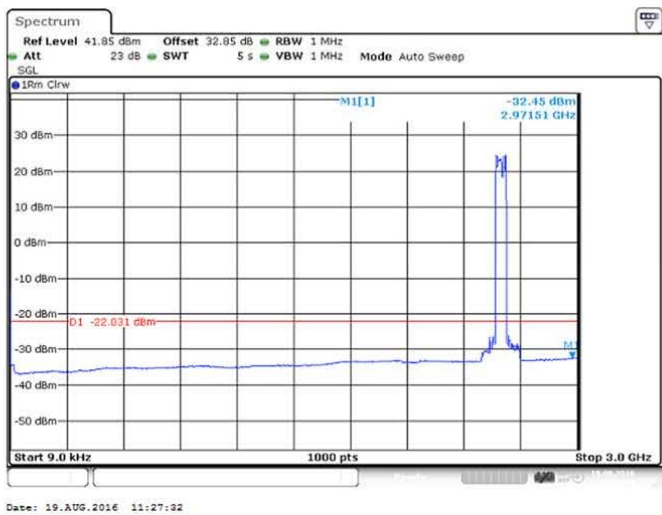
Figure 209 Spurious Emissions (9kHz – 3GHz) – 64QAM (2573/ 2593/ 2613 MHz) (3 X 20 MHz Channel BW)
