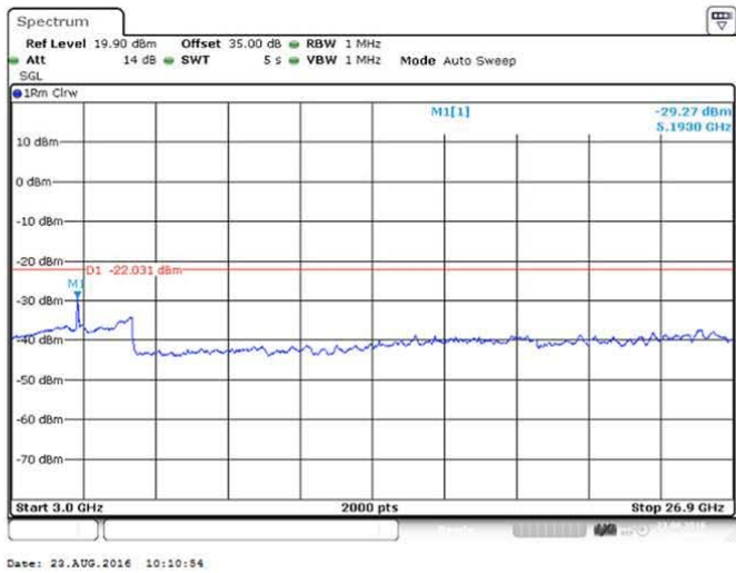
Figure 190 Spurious Emissions (3GHz – 26.900GHz) – 16QAM (2573/ 2593/ 2613 MHz) (3 X 20 MHz Channel BW)
