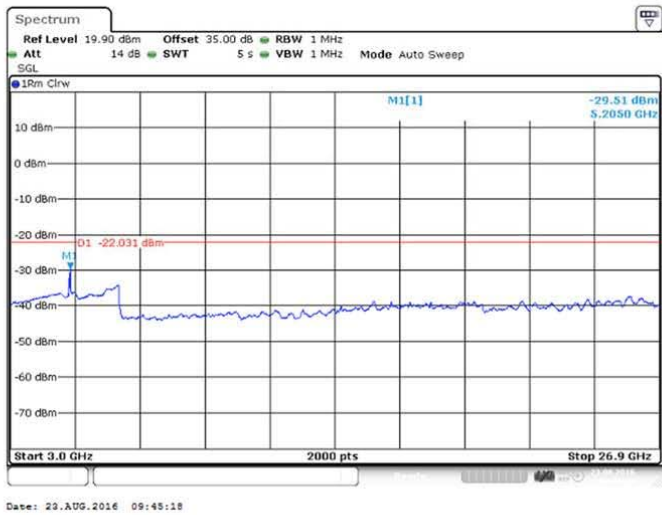
Figure 174 Spurious Emissions (3GHz – 26.900GHz) – 64QAM (2573/ 2593/ 2613 MHz) (3 X 20 MHz Channel BW)
