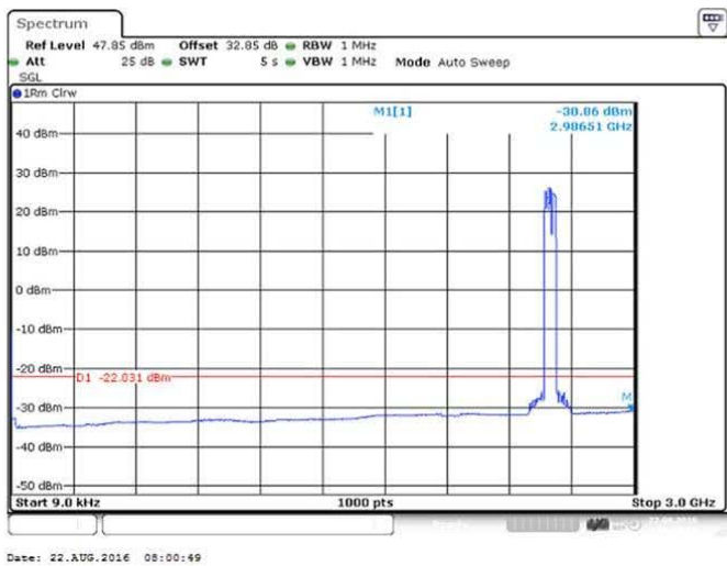
Figure 221 Spurious Emissions (9kHz – 3GHz) – 64QAM (2573/ 2593/ 2613 MHz) (3 X 20 MHz Channel BW)
