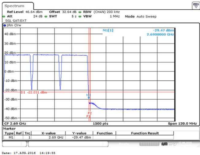
Figure 220 Spurious Emissions (Upper Band Edge) – 64QAM (2640/ 2660/ 2680 MHz) (3 X 20 MHz Channel BW)
