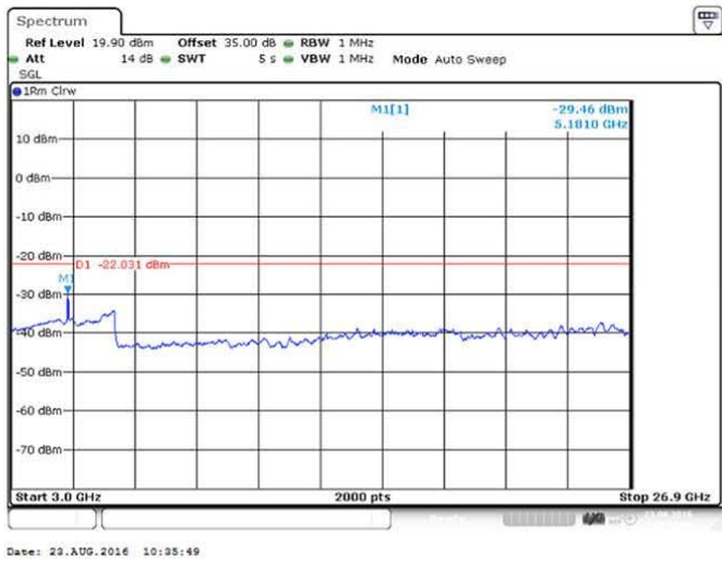
Figure 210 Spurious Emissions (3GHz – 26.900GHz) – 64QAM (2573/ 2593/ 2613 MHz) (3 X 20 MHz Channel BW)
