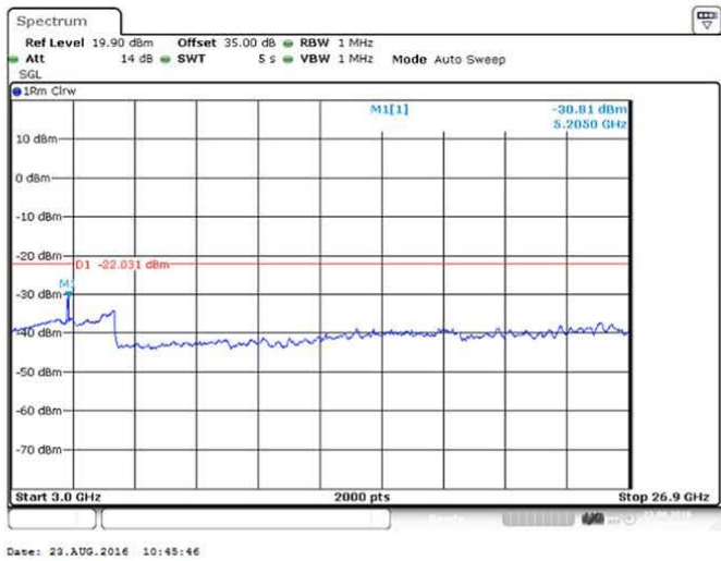
Figure 218 Spurious Emissions (3GHz – 26.900GHz) – QPSK (2573/ 2593/ 2613 MHz) (3 X 20 MHz Channel BW)
