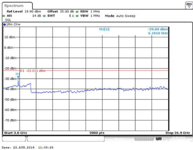
Figure 234 Spurious Emissions (3GHz – 26.900GHz) – 64QAM (2573/ 2593/ 2613 MHz) (3 X 20 MHz Channel BW)
