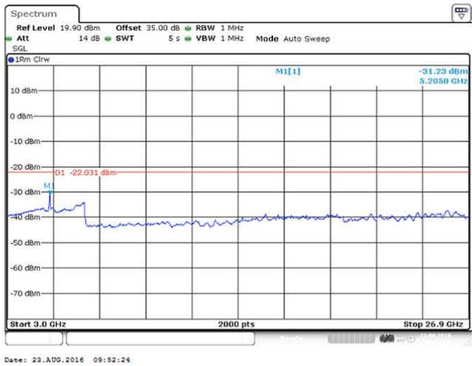
Figure 178 Spurious Emissions (3GHz – 26.900GHz) – 16QAM (2573/ 2593/ 2613 MHz) (3 X 20 MHz Channel BW)
