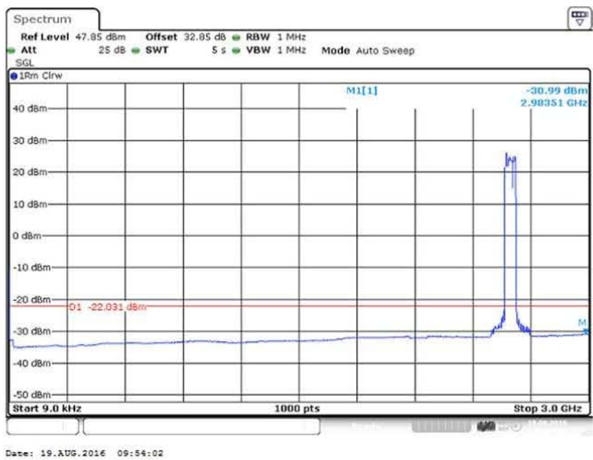
Figure 177 Spurious Emissions (9kHz – 3GHz) – 16QAM (2573/ 2593/ 2613 MHz) (3 X 20 MHz Channel BW)
