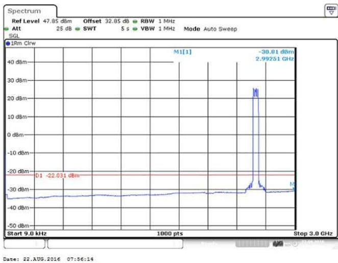
Figure 217 Spurious Emissions (9kHz – 3GHz) – QPSK (2573/ 2593/ 2613 MHz) (3 X 20 MHz Channel BW)
