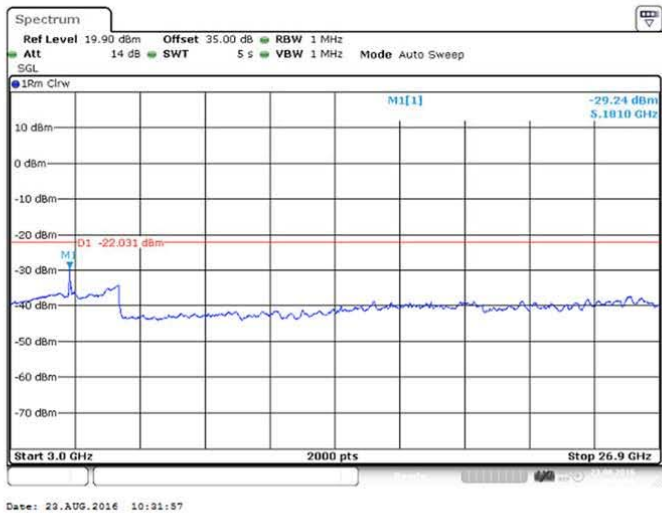
Figure 206 Spurious Emissions (3GHz – 26.900GHz) – QPSK (2573.0/2593/2613.0 MHz) (3 X 20 MHz Channel BW)
