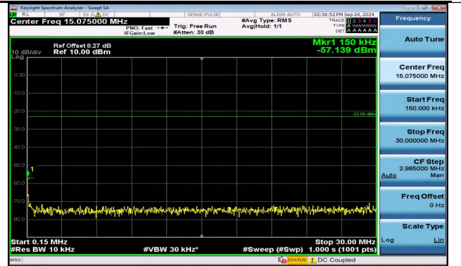
Band5_1.4MHz_QPSK_20643_1RB#0_0.15~30_0.15~30
