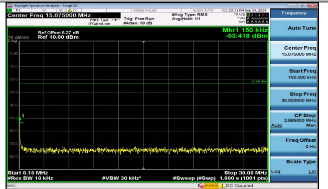
Band5_1.4MHz_QPSK_20643_1RB#5_0.15~30_0.15~30
