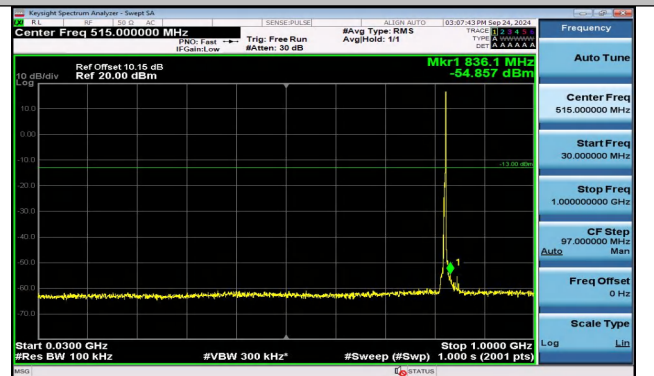
Band5_3MHz_16QAM_20415_1RB#14_30~1000_30~1000 0
