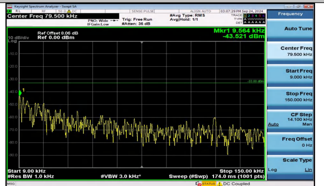
Band5_3MHz_16QAM_20415_1RB#14_0.009~0.15_0.009 ~0.15
