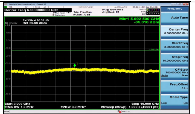
Band5_3MHz_16QAM_20415_1RB#14_3000~10000_3000 ~10000
