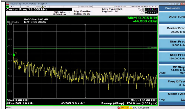
Band5_3MHz_QPSK_20415_1RB#0_0.009~0.15_0.009~0.15
