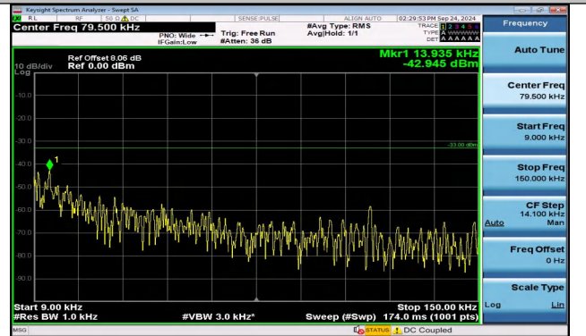
Band5_1.4MHz_16QAM_20525_6RB#0_0.009~0.15_0.009~0.15 ~0.15
