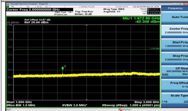
Band5_1.4MHz_16QAM_20525_6RB#0_1000~3000_1000~3000 0~3000
