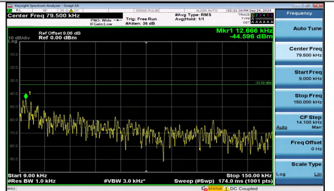
Band5_1.4MHz_16QAM_20643_1RB#0_0.009~0.15_0.009 ~0.15
