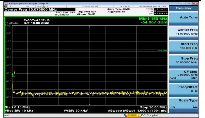
Band5_3MHz_QPSK_20415_1RB#14_0.15~30_0.15~30
