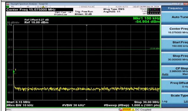
Band5_3MHz_16QAM_20415_1RB#14_0.15~30_0.15~3 0
