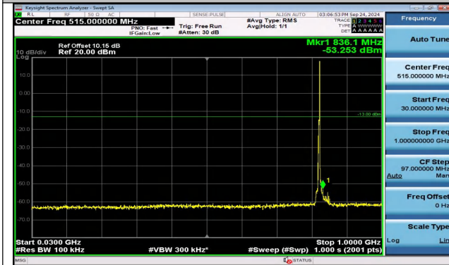
Band5_3MHz_QPSK_20415_1RB#14_30~1000_30~1000
