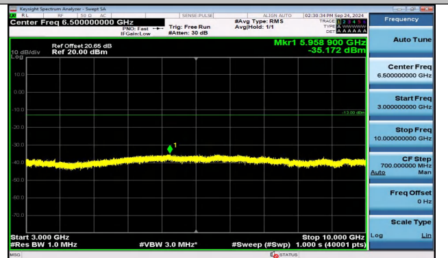
Band5_1.4MHz_16QAM_20525_6RB#0_3000~10000_3000~10000 0~10000
