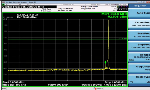
Band5_1.4MHz_QPSK_20643_1RB#0_30~1000_30~100 0
