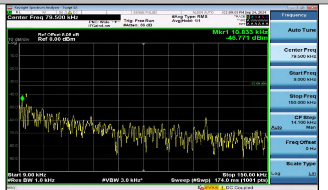
Band5_3MHz_16QAM_20415_15RB#0_0.009~0.15_0.009 ~0.15
