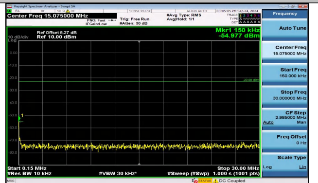
Band5_3MHz_QPSK_20415_1RB#0_0.15~30_0.15~30
