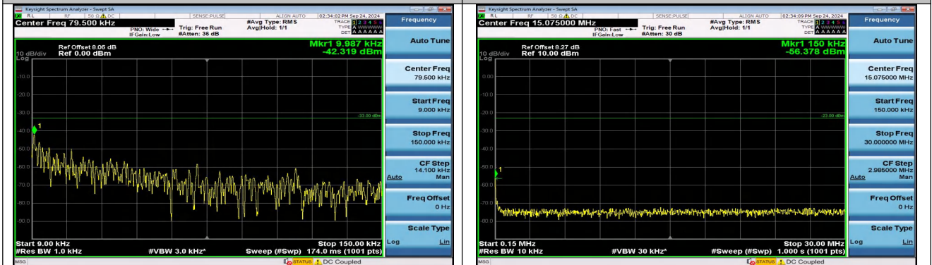
Band5_1.4MHz_QPSK_20643_6RB#0_0.009~0.15_0.009
