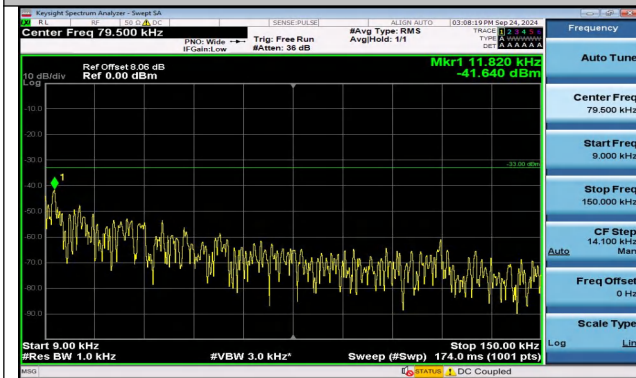
Band5_3MHz_QPSK_20415_15RB#0_0.009~0.15_0.009 ~0.15
