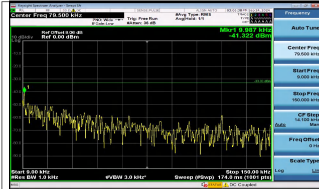
Band5_3MHz_QPSK_20415_1RB#14_0.009~0.15_0.009 ~0.15
