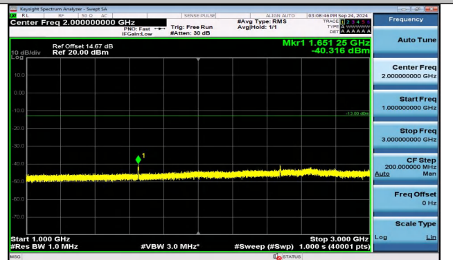
Band5_3MHz_QPSK_20415_15RB#0_1000~3000_1000~3000
