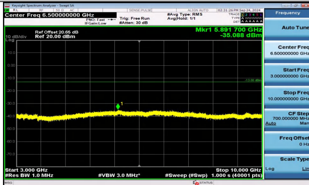
Band5_1.4MHz_QPSK_20643_1RB#0_3000~10000_3000~10000
