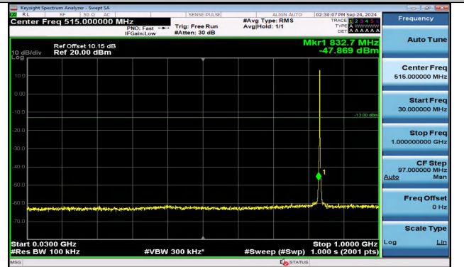
Band5_1.4MHz_16QAM_20525_6RB#0_30~1000_30~1000 0
