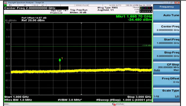
Band5_1.4MHz_QPSK_20643_1RB#0_1000~3000_1000~3000
