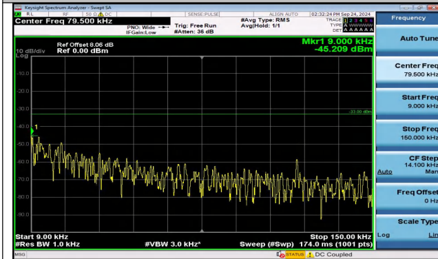
Band5_1.4MHz_QPSK_20643_1RB#5_0.009~0.15_0.009 ~0.15
