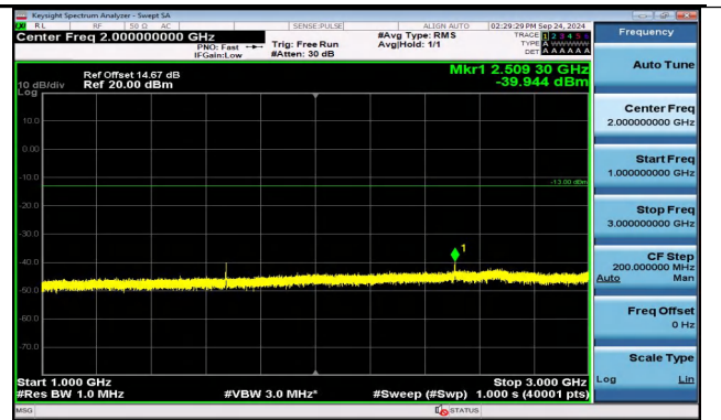
Band5_1.4MHz_QPSK_20525_6RB#0_1000~3000_1000~3000 3000
