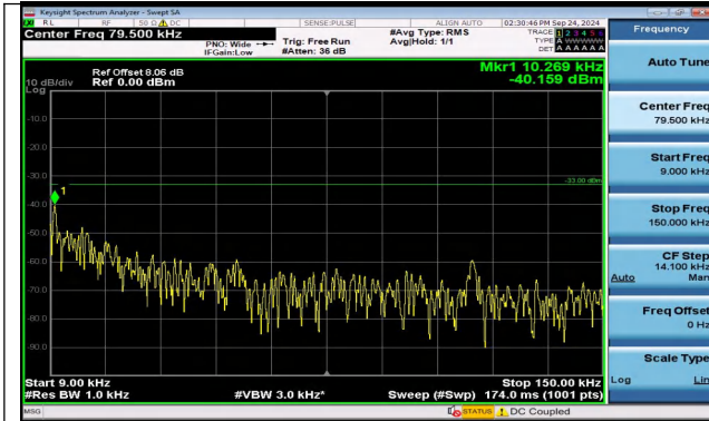
Band5_1.4MHz_QPSK_20643_1RB#0_0.009~0.15_0.009 ~0.15
