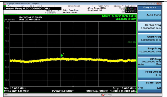
Band5_1.4MHz_16QAM_20643_1RB#0_3000~10000_300 0~10000
