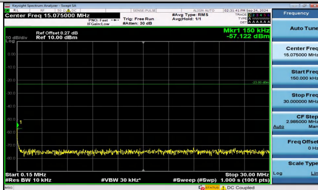
Band5_1.4MHz_16QAM_20643_1RB#0_0.15~30_0.15~30 0
