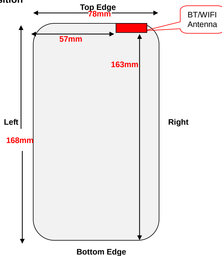
< EUT Front Side View >
