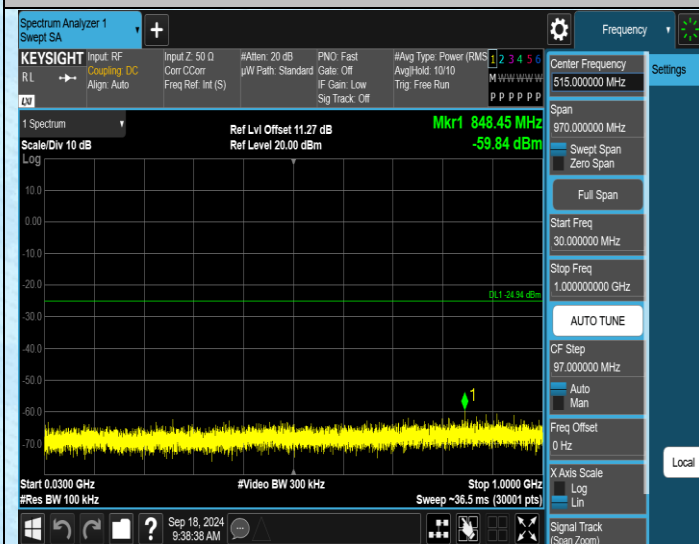
11G-Ant2-2437-30~1000-PASS
