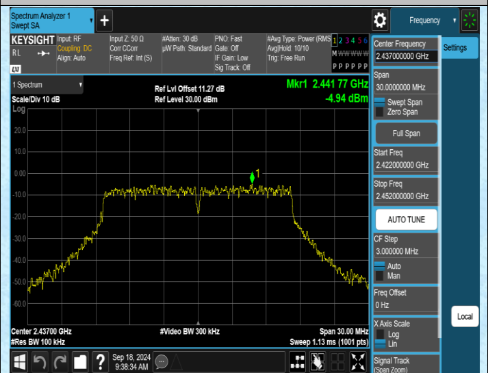
11G-Ant2-2437-0~Reference-PASS
