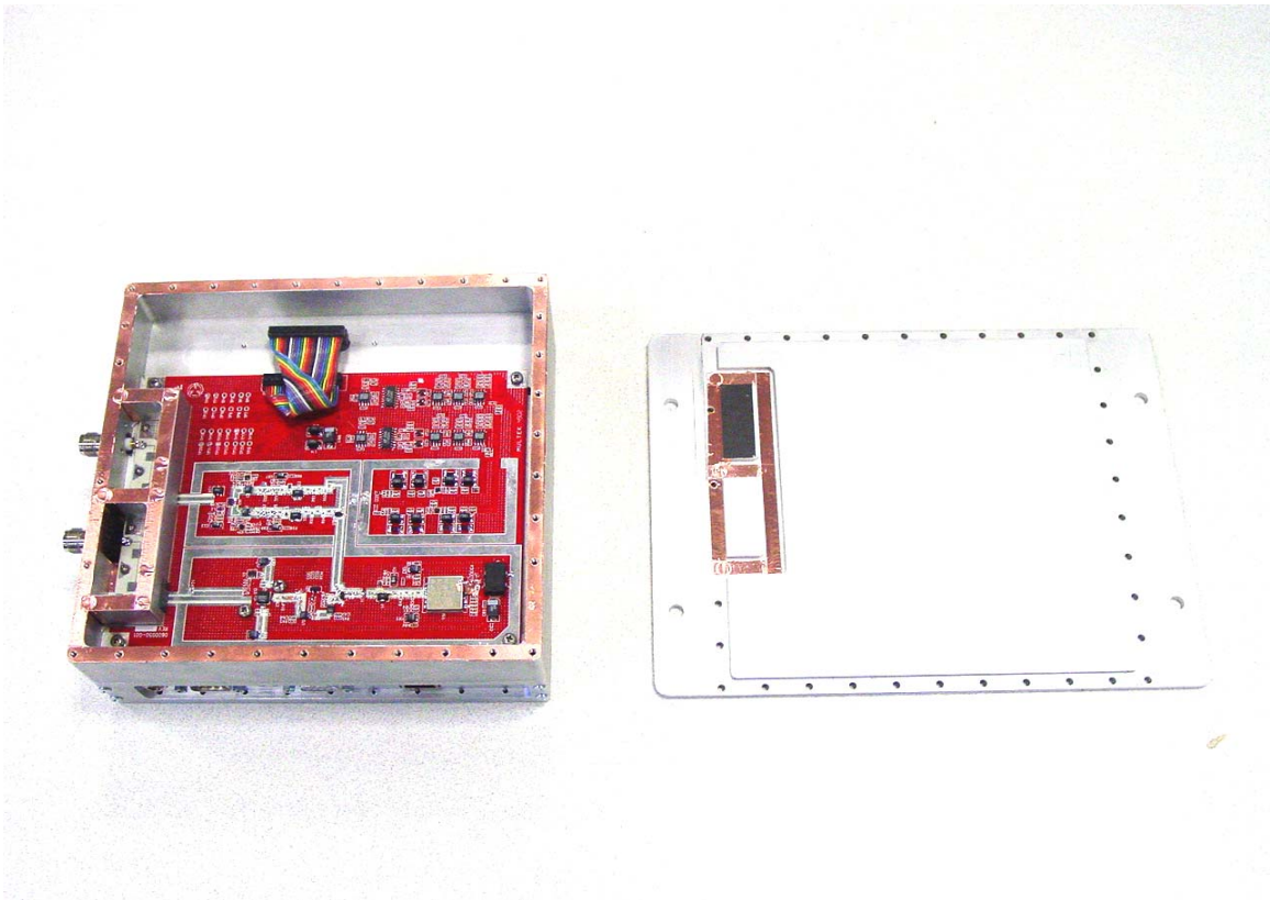
B2450R01 Assembly RF
