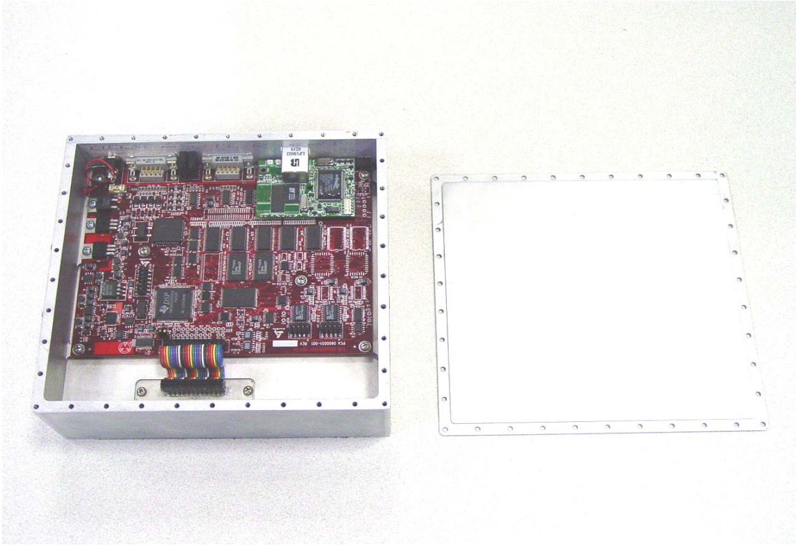
B2450R01 Assembly Digital
