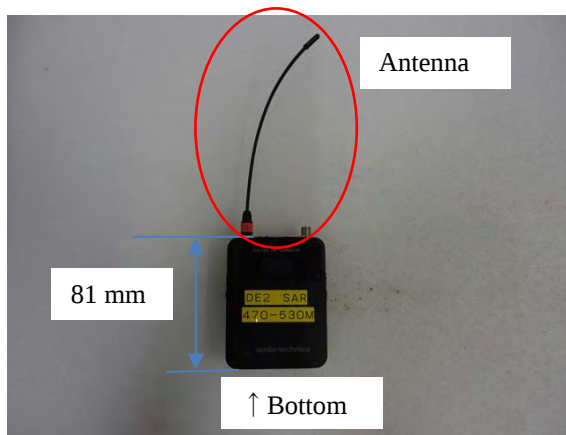
Photograph C1: Antenna position
