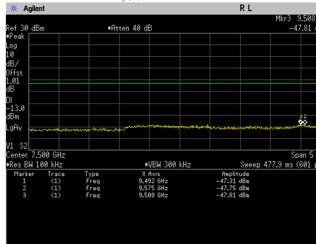
Conducted Emissions. Bluetooth LE, Frequency 2440 MHz Emission Level, 5 GHz -> 10 GHz
