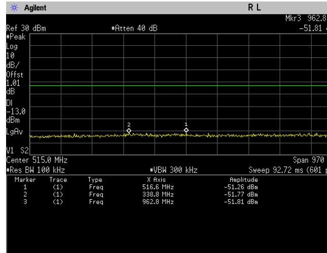
Conducted Emissions. Bluetooth LE, Frequency 2440 MHz Emission Level, 30 MHz -> 1 GHz
