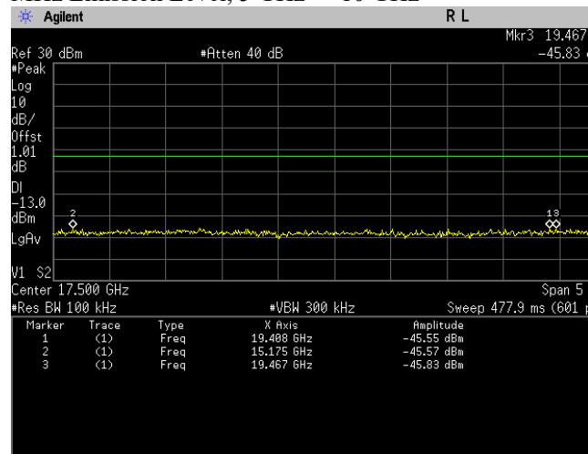
Conducted Emissions. Bluetooth LE, Frequency 2440 MHz Emission Level, 15 GHz -> 20 GHz
