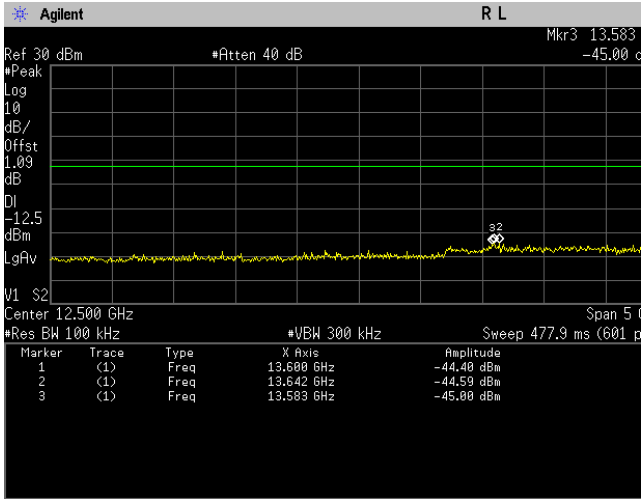
Conducted Emissions. Bluetooth LE, Frequency 2402 Emission Level, 10 GHz -> 15 GHz
