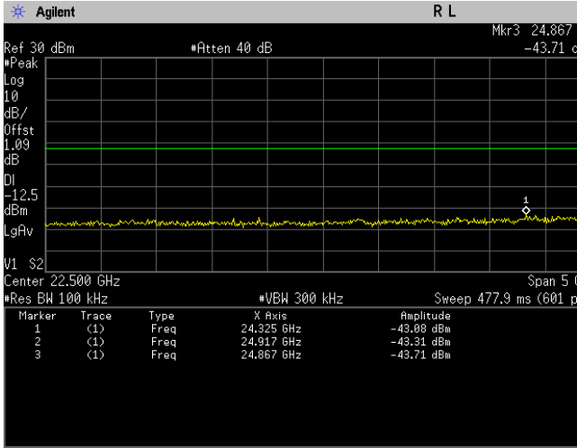
Conducted Emissions. Bluetooth LE, Frequency 2402 MHz Emission Level, 20 GHz -> 25 GHz
