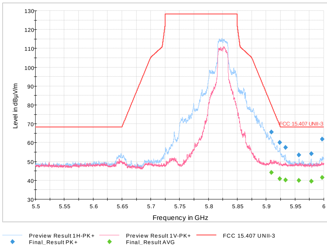
Figure 24: High Band Edge 802.11n HT Mode 20 MHz, High Channel
