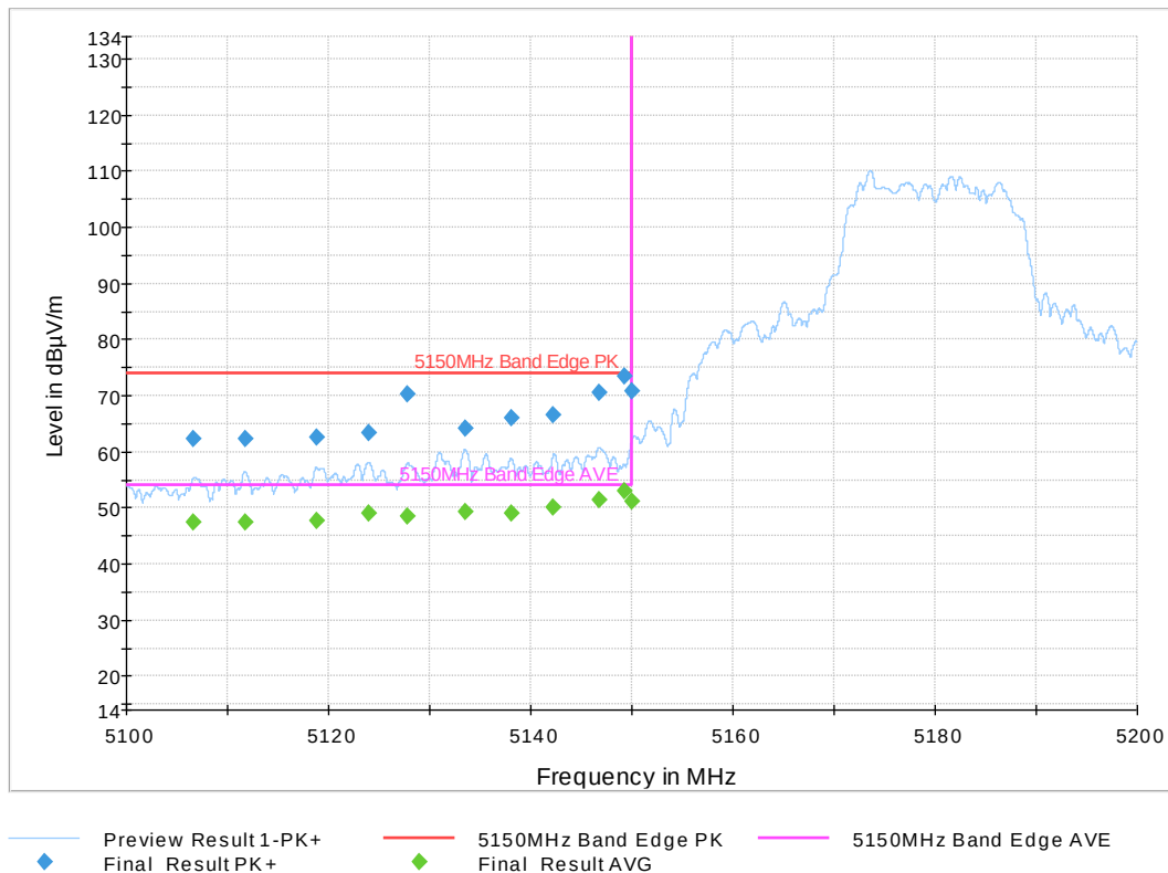
Figure 8: Low Band Edge 802.11ac VHT Mode 20 MHz, Low Channel
