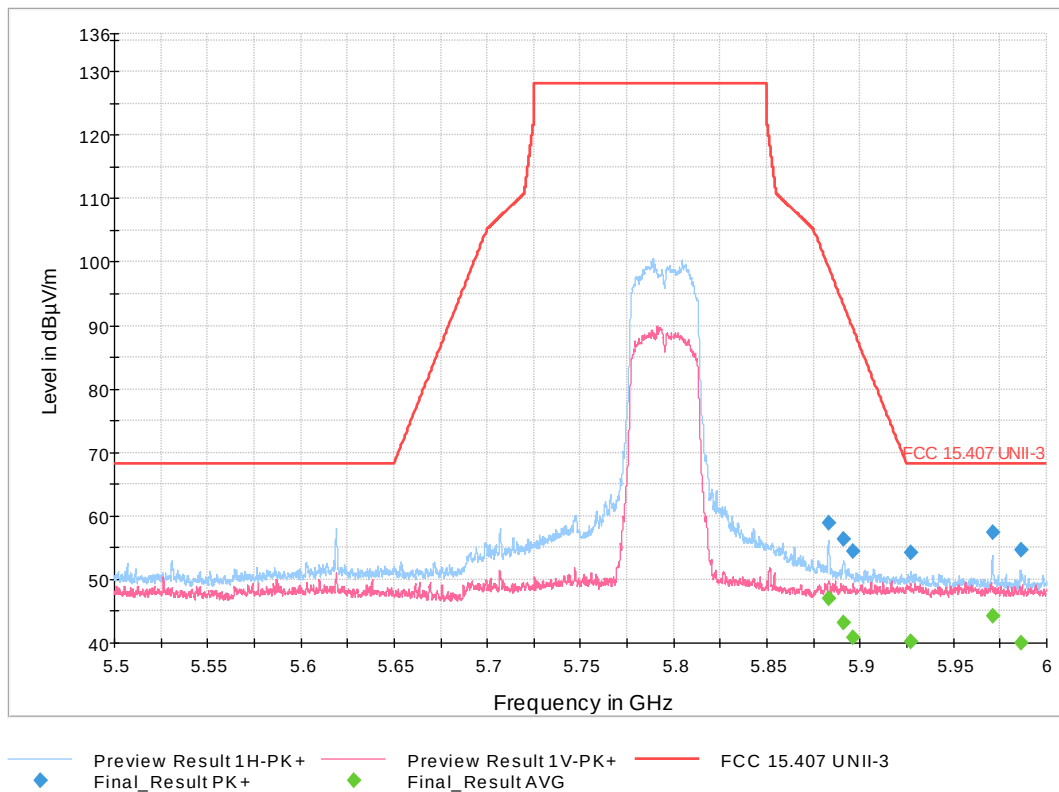
Figure 27: High Band Edge 802.11ac VHT Mode 40 MHz, High Channel
