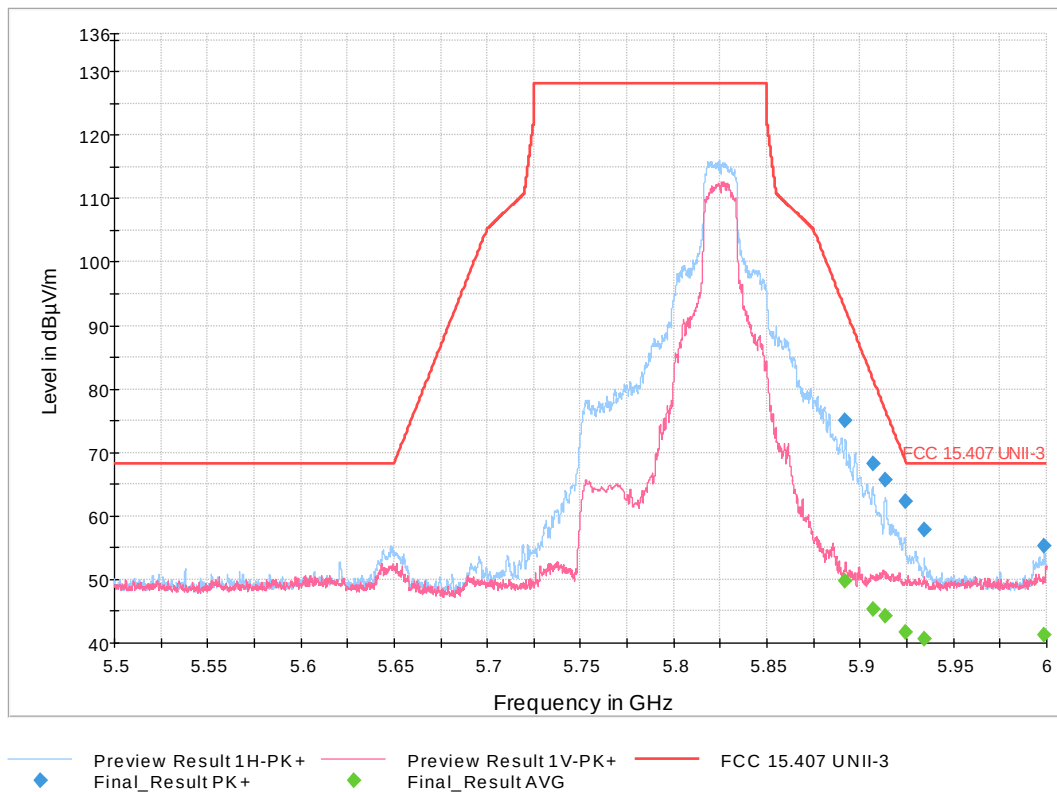
Figure 26: High Band Edge 802.11ac VHT Mode 20 MHz, High Channel
