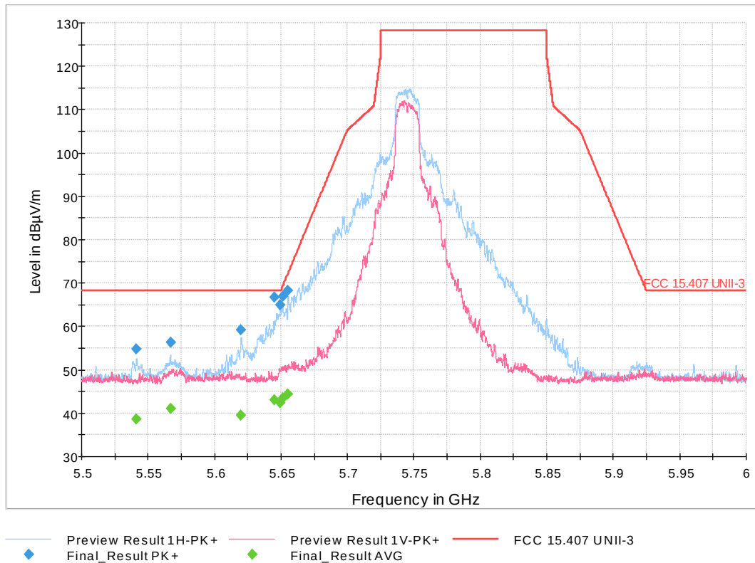
Figure 15: Low Band Edge 802.11n HT Mode 20 MHz, Low Channel
