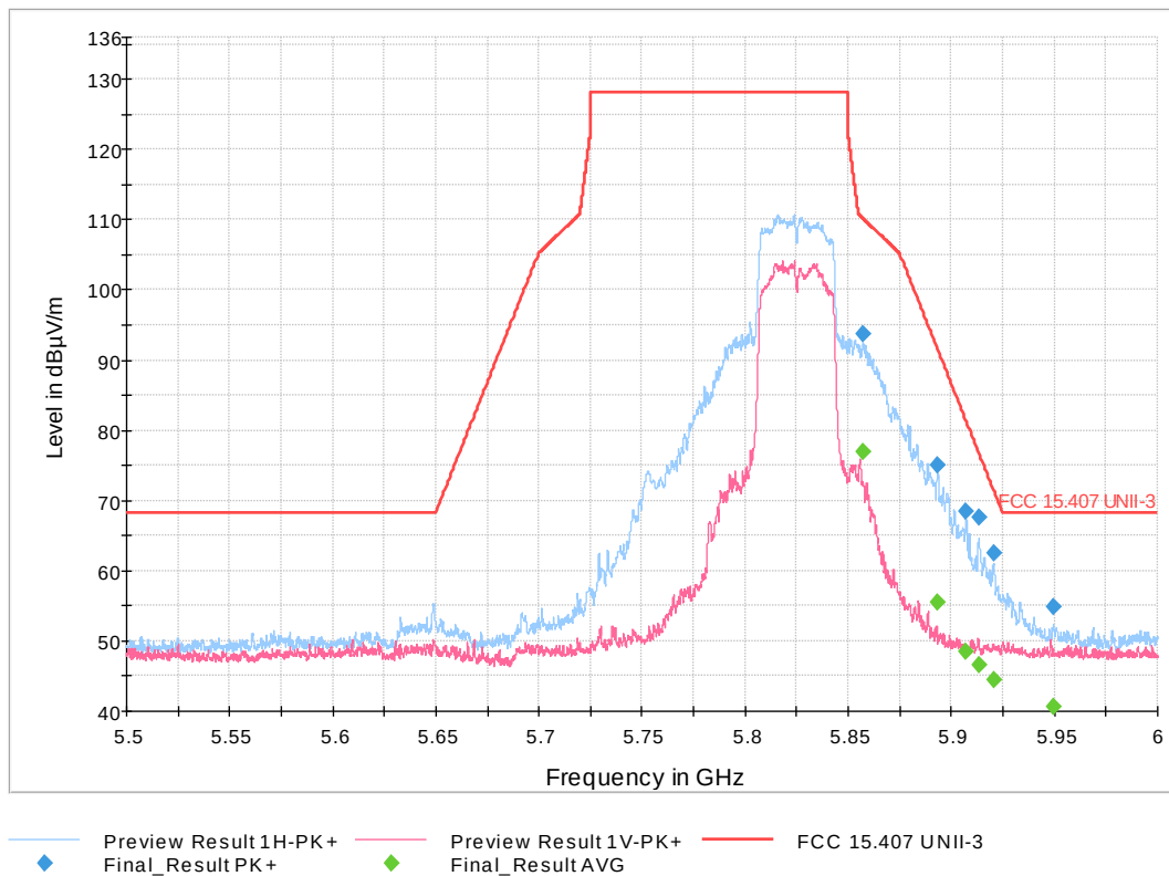
Figure 25: High Band Edge 802.11n HT Mode 40 MHz, High Channel
