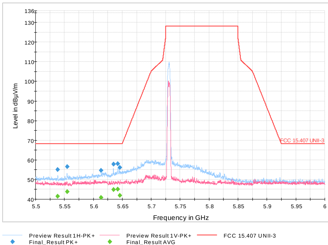
Figure 13: Low Band Edge 802.11n HT Mode 5 MHz, Low Channel
