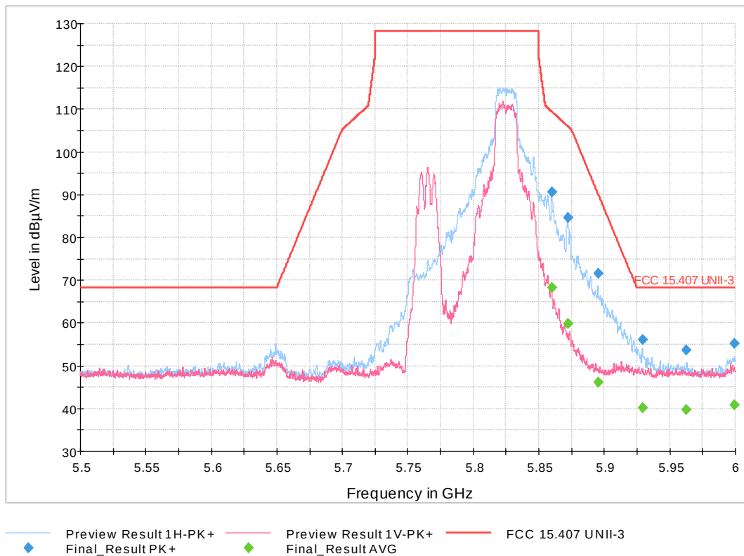
Figure 21: High Band Edge 802.11a Mode 20 MHz, High Channel
