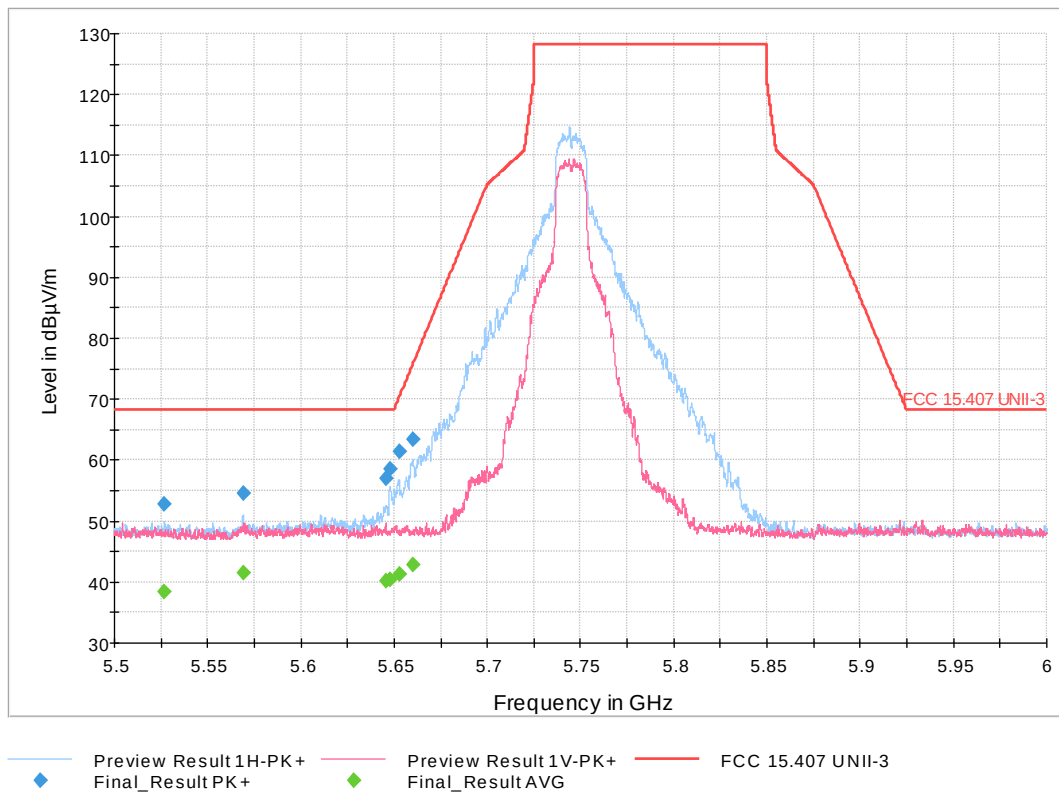
Figure 12: Low Band Edge 802.11a Mode 20 MHz, Low Channel
