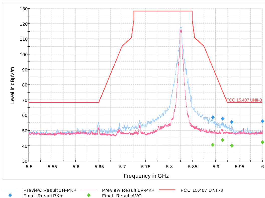
Figure 19: High Band Edge 802.11a Mode 5 MHz, High Channel
