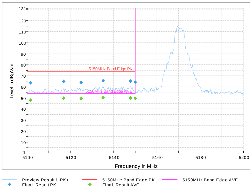
Figure 1: Low Band Edge 802.11a Mode 5 MHz, Low Channel
