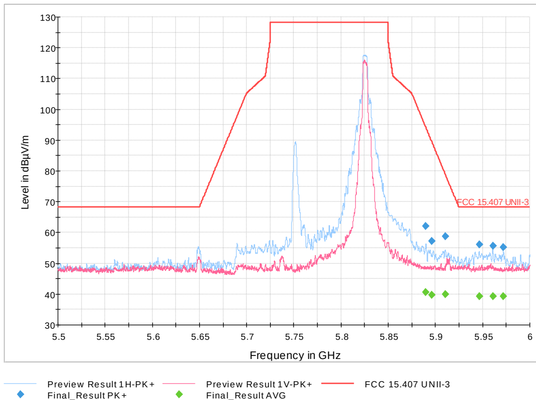
Figure 22: High Band Edge 802.11n HT Mode 5 MHz, High Channel
