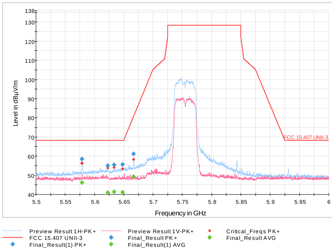
Figure 16: Low Band Edge 802.11n HT Mode 40 MHz, Low Channel
