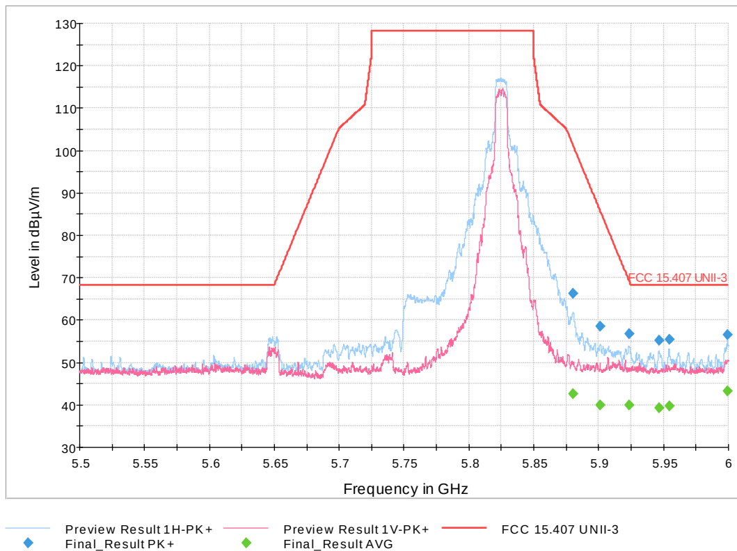
Figure 23: High Band Edge 802.11n HT Mode 10 MHz, High Channel
