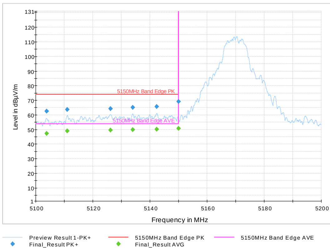
Figure 2: Low Band Edge 802.11a Mode 10 MHz, Low Channel
