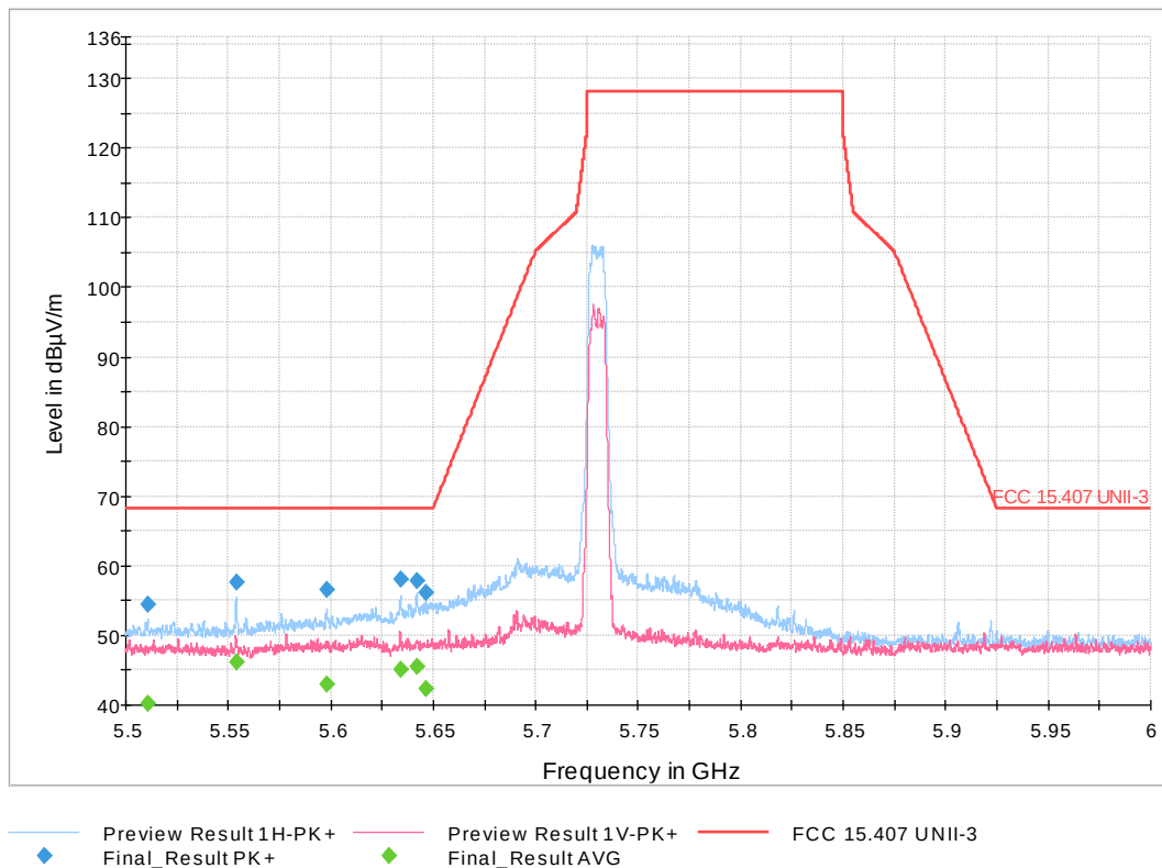
Figure 11: Low Band Edge 802.11a Mode 10 MHz, Low Channel
