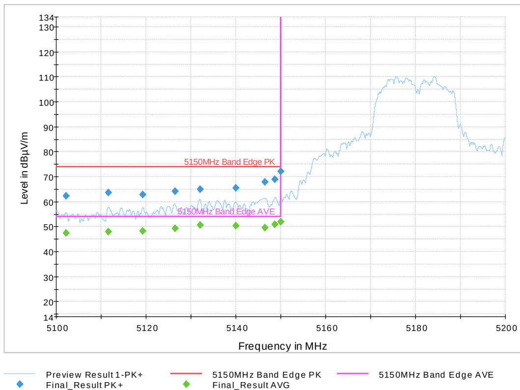
Figure 6: Low Band Edge 802.11n HT Mode 20 MHz, Low Channel
