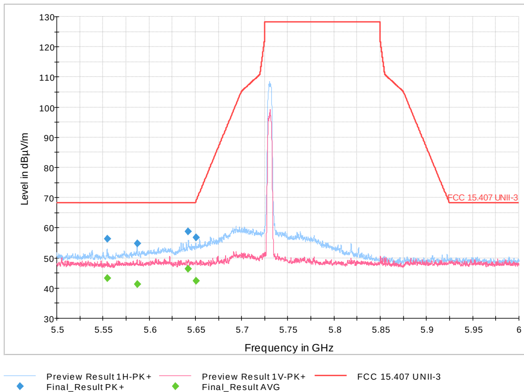
Figure 10: Low Band Edge 802.11a Mode 5 MHz, Low Channel
