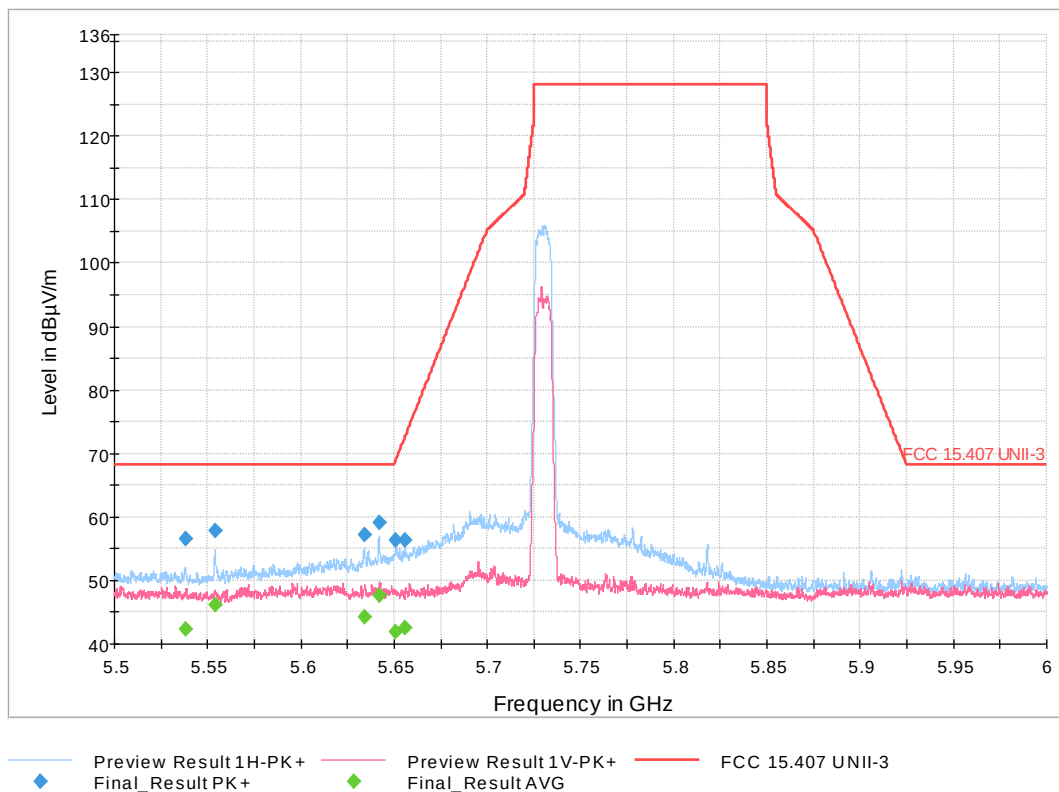
Figure 14: Low Band Edge 802.11n HT Mode 10 MHz, Low Channel
