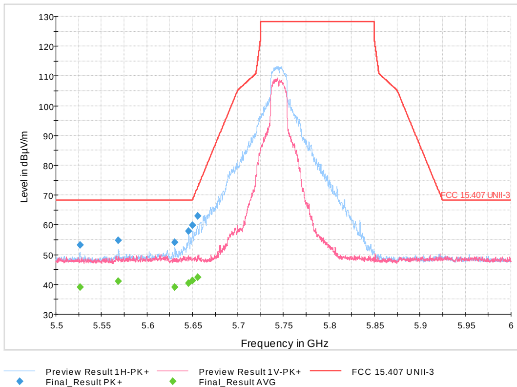
Figure 17: Low Band Edge 802.11ac VHT Mode 20 MHz, Low Channel
