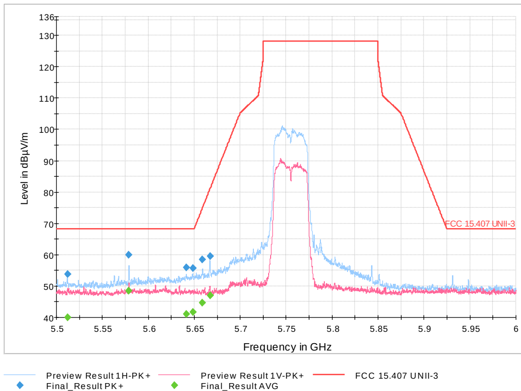
Figure 18: Low Band Edge 802.11ac VHT Mode 40 MHz, Low Channel
