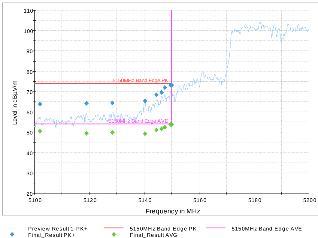
Figure 9: Low Band Edge 802.11ac VHT Mode 40 MHz, Low Channel
