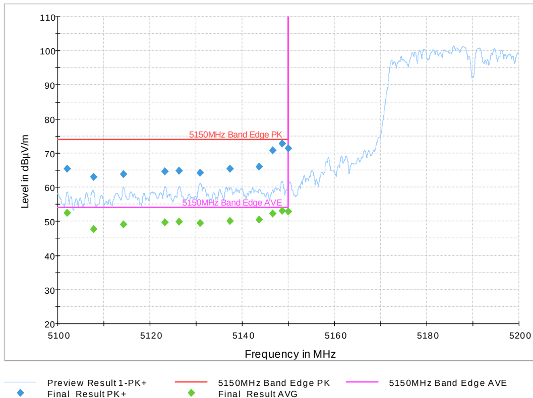
Figure 7: Low Band Edge 802.11n HT Mode 40 MHz, Low Channel
