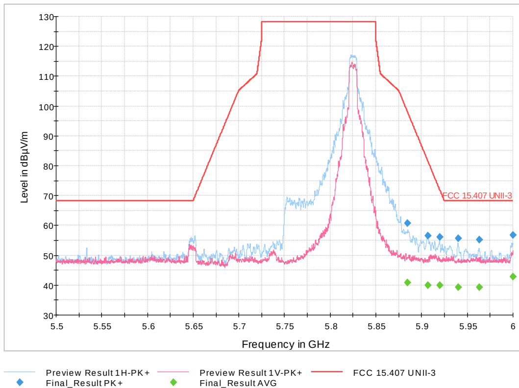
Figure 20: High Band Edge 802.11a Mode 10 MHz, High Channel
