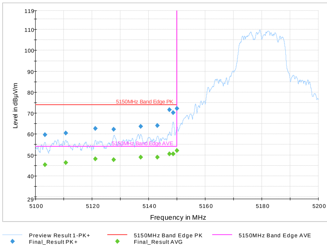
Figure 3: Low Band Edge 802.11a Mode 20 MHz, Low Channel
