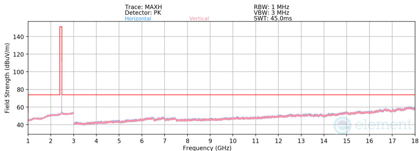
Plot 7-114. Radiated Spurious Emissions 1-18GHz TxBF (4Mbps, HDR4, ePA – Ch. 73)
