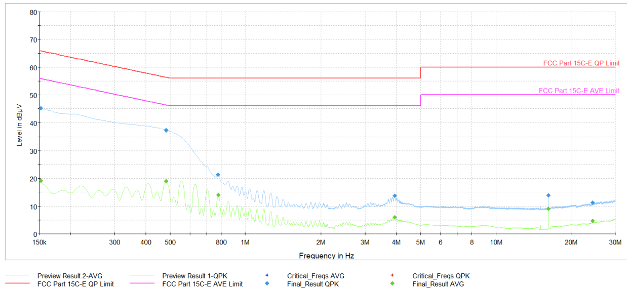
Plot 7-134. AC Line Conducted Plot with Bluetooth HDR Ant2 (L1, 4Mbps ePA - Ch.38 with AC/DC Adapter)
