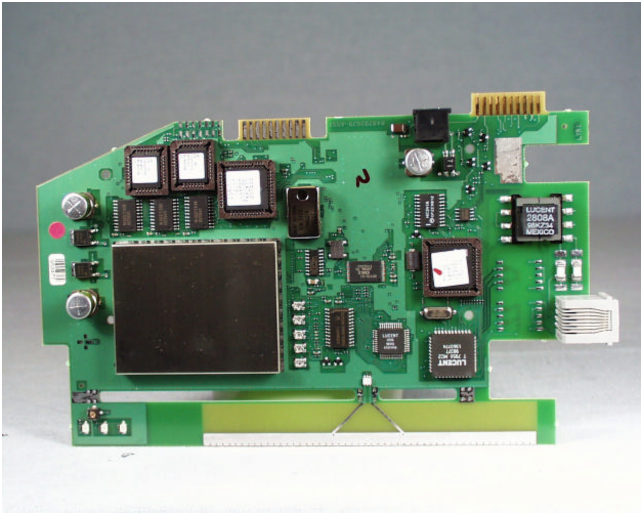
Component Side of PCB with RF cans installed (Base)
