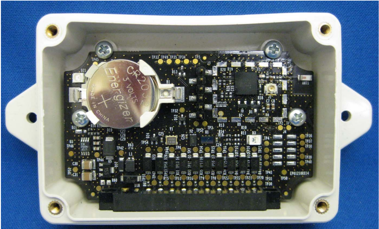
Shield Off - plastic cover removed, board screwed to enclosure
