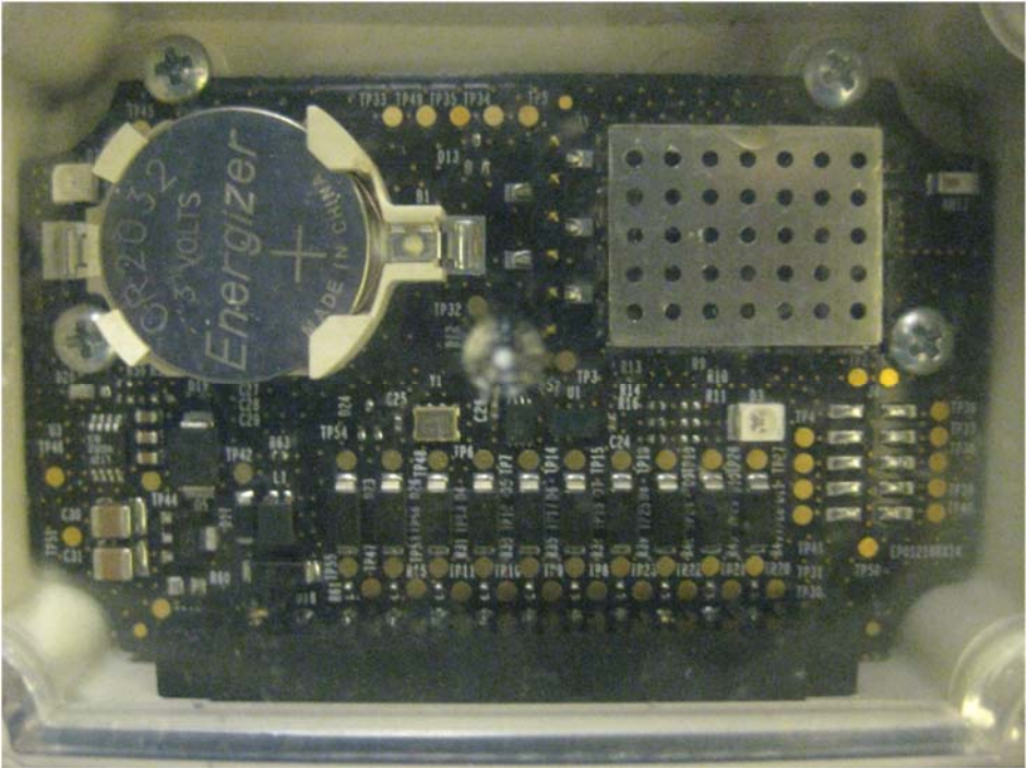
Shield On looking thru clear plastic cover
