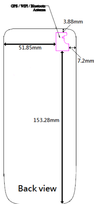
Fig.17 Antenna position of EUT
