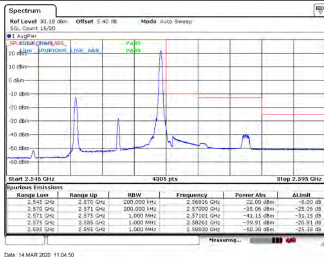
Band7_15MHz_16QAM_21375_75RB#0
