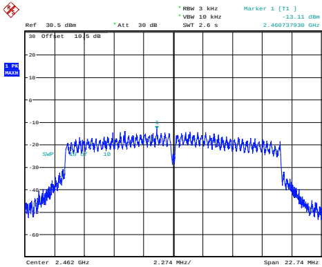
g_2462MHz_Chain 0 -13.11dBm/3kHz
