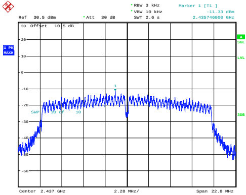
n20_2437MHz_Chain 0 -11.33dBm/3kHz
