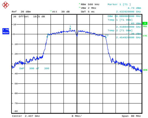
n40_2437MHz_Chain 0 36.080MHz
