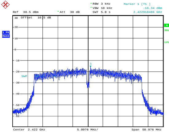
n40_2422MHz_Chain 1 -16.34dBm/3kHz
