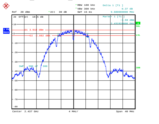
b_2437MHz_Chain 0 9.680MHz
