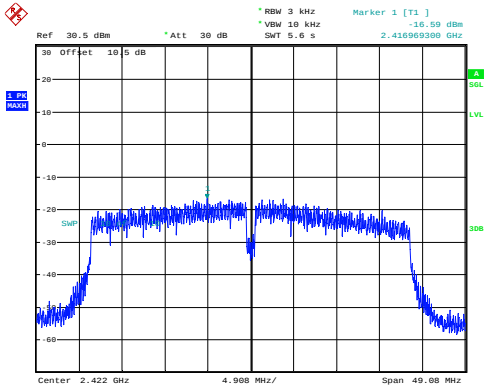
n40_2422MHz_Chain 0 -16.59dBm/3kHz
