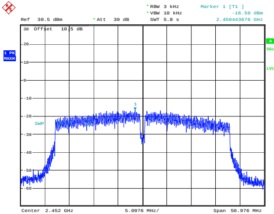
n40_2452MHz_Chain 1 -16.59dBm/3kHz
