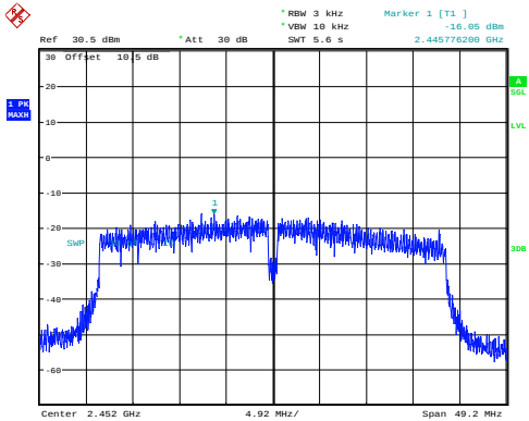
n40_2452MHz_Chain 0 -16.05dBm/3kHz
