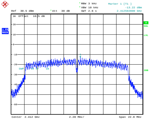
n20_2412MHz_Chain 0 -13.22dBm/3kHz
