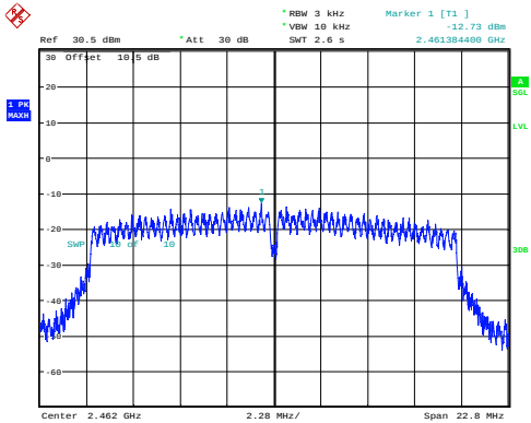
n20_2462MHz_Chain 0 -12.73dBm/3kHz
