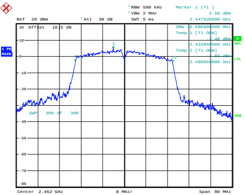
n40_2452MHz_Chain 0 36.080MHz
