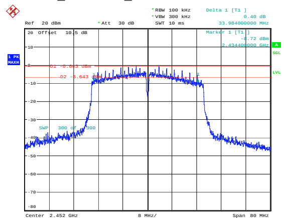
n40_2452MHz_Chain 1 33.984MHz
