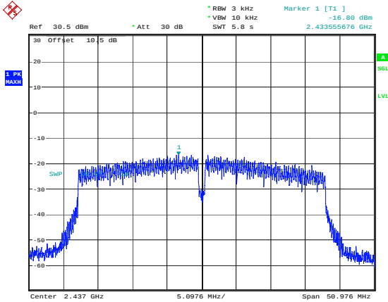
n40_2437MHz_Chain 1 -16.80dBm/3kHz
