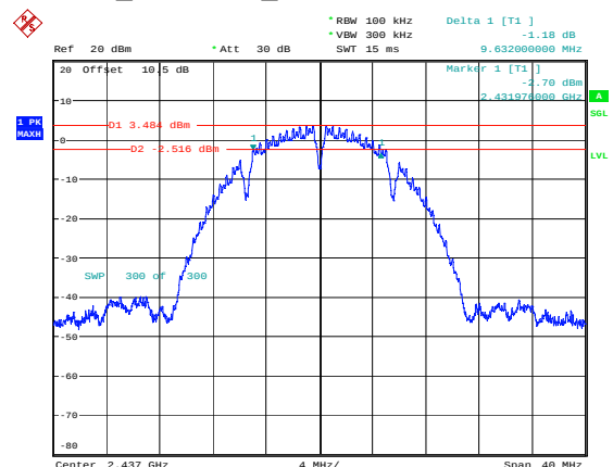
b_2437MHz_Chain 1 9.632MHz
