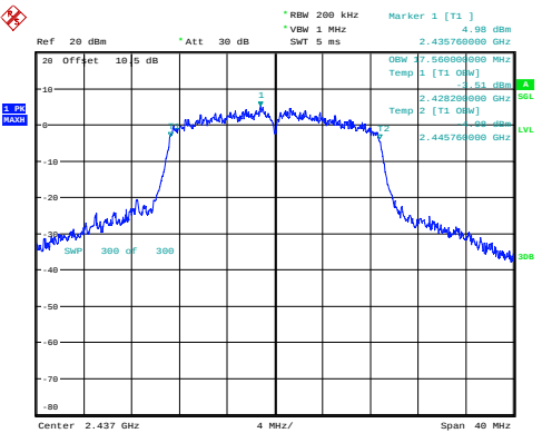
n20_2437MHz_Chain 0 17.560MHz
