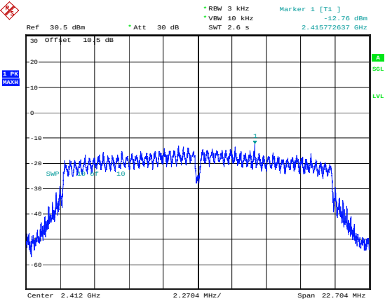
n20_2412MHz_Chain 1 -12.76dBm/3kHz
