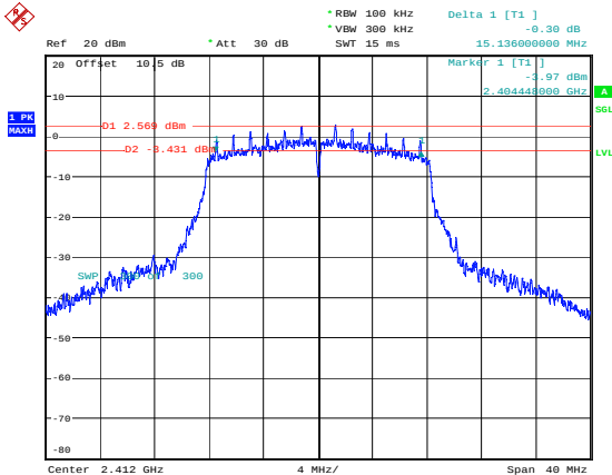
g_2412MHz_Chain 1 15.136MHz
