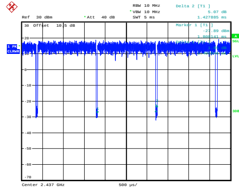
g_2437MHz_Chain 0 1.404ms,1.428ms
