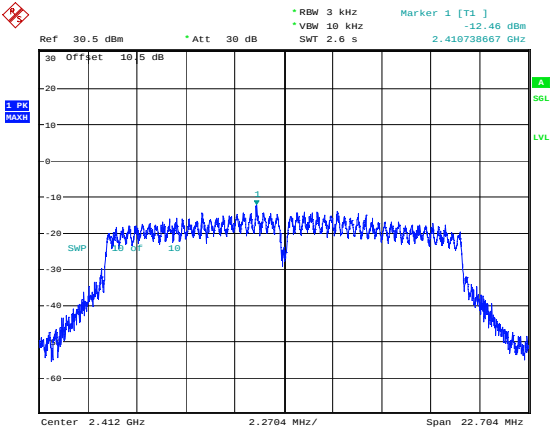
g_2412MHz_Chain 1 -12.46dBm/3kHz
