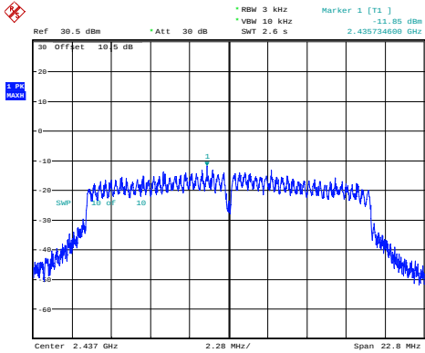
g_2437MHz_Chain 0 -11.85dBm/3kHz
