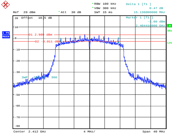
n20_2412MHz_Chain 1 15.136MHz
