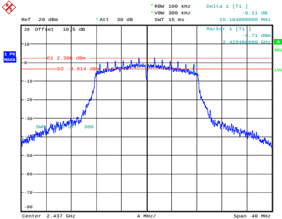
g_2437MHz_Chain 1 15.104MHz
