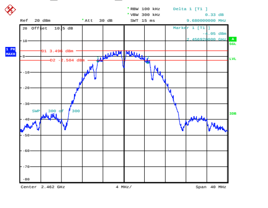
b_2462MHz_Chain 0 9.680MHz
