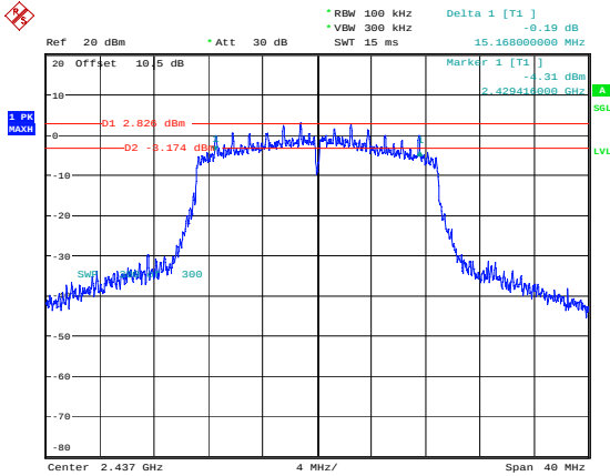
n20_2437MHz_Chain 1 15.168MHz
