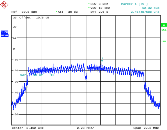
n20_2462MHz_Chain 1 -12.32dBm/3kHz
