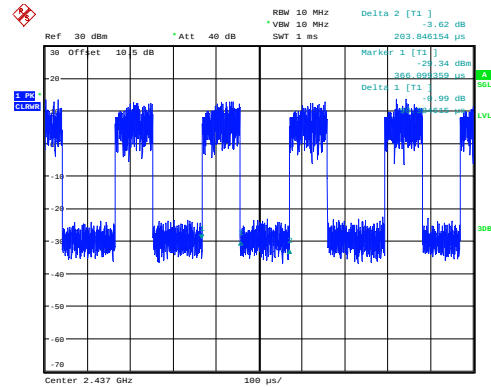
n40_2437MHz_Chain 0 0.090ms,0.204ms
