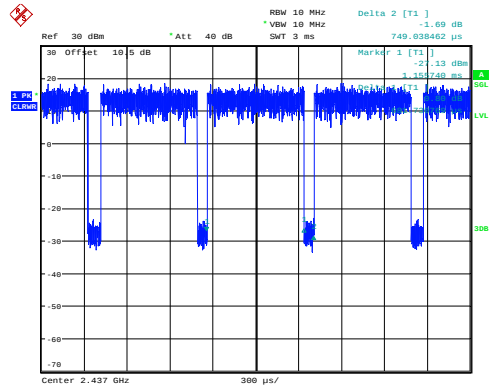
n20_2437MHz_Chain 0 0.682ms,0.749ms
