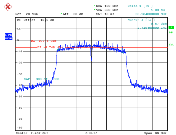
n40_2437MHz_Chain 1 33.984MHz
