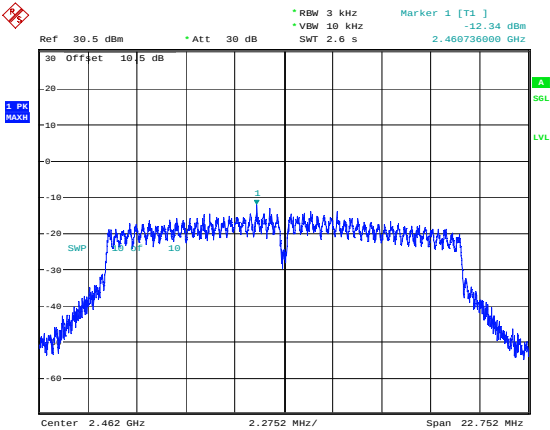
g_2462MHz_Chain 1 -12.34dBm/3kHz
