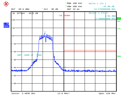
g_2462MHz_Chain 1 43.89dB
