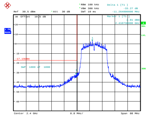
n20_2412MHz_Chain 1 33.27dB
