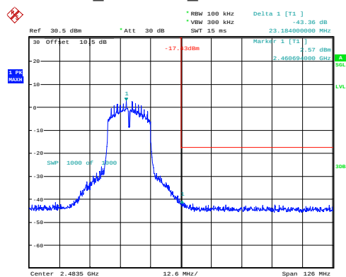
n20_2462MHz_Chain 0 43.36dB
