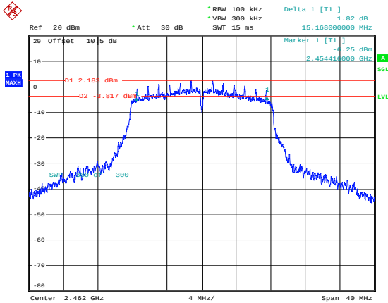
g_2462MHz_Chain 1 15.168MHz
