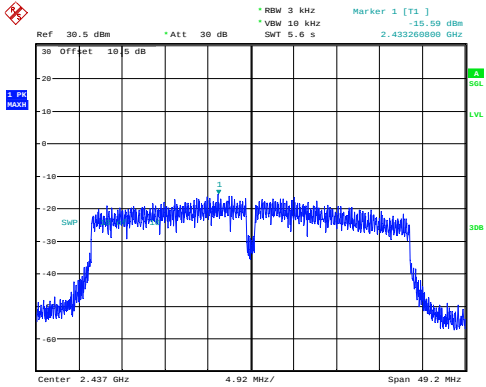
n40_2437MHz_Chain 0 -15.59dBm/3kHz
