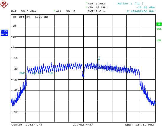
n20_2437MHz_Chain 1 -12.38dBm/3kHz
