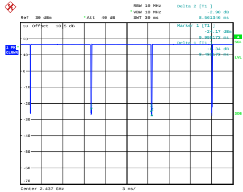
b_2437MHz_Chain 0 8.483ms,8.561ms
