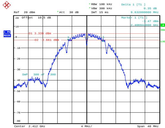
b_2412MHz_Chain 0 9.632MHz
