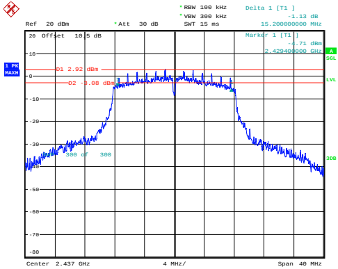
g_2437MHz_Chain 0 15.200MHz
