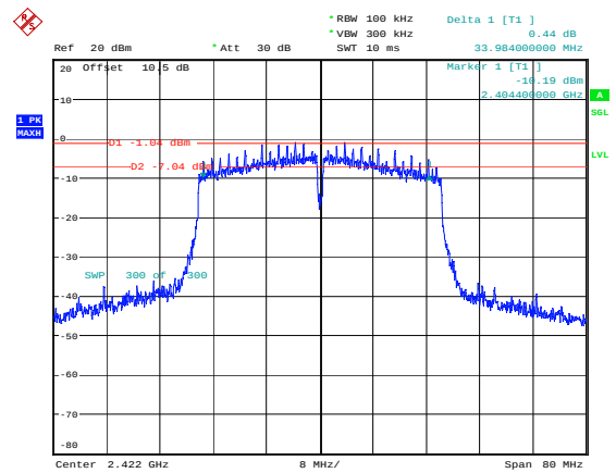
n40_2422MHz_Chain 1 33.984MHz
