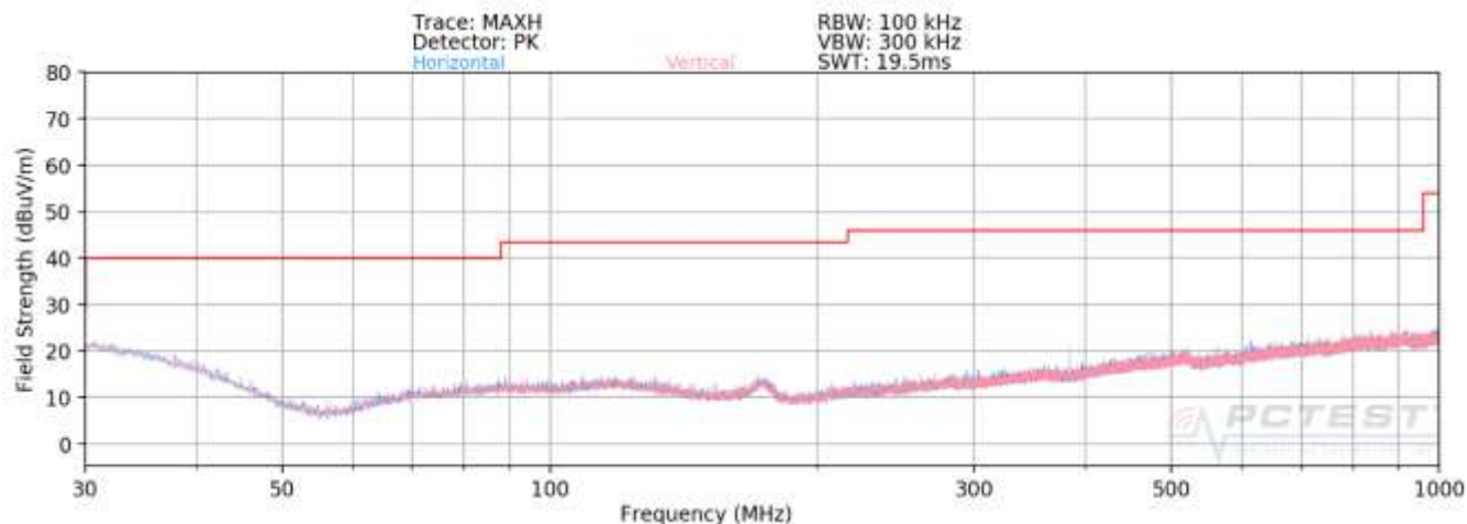
Plot 7-118. Radiated Spurious Plot below 1GHz (802.11a – U3 Ch. 157)
