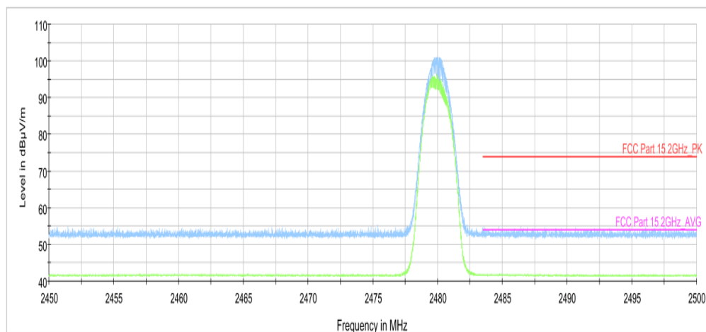
Fig.18. Frequency Band Edges: 8DPSK, Channel 78, 2.45 GHz - 2.50GHz
