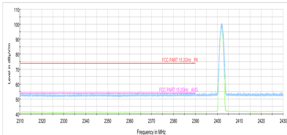
Fig.15. Frequency Band Edges: \pi/4 DQPSK, Channel 0, 2.31 GHz - 2.43GHz
