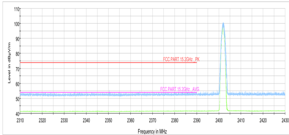
Fig.13. Frequency Band Edges: GFSK, Channel 0, 2.31 GHz – 2.43GHz
