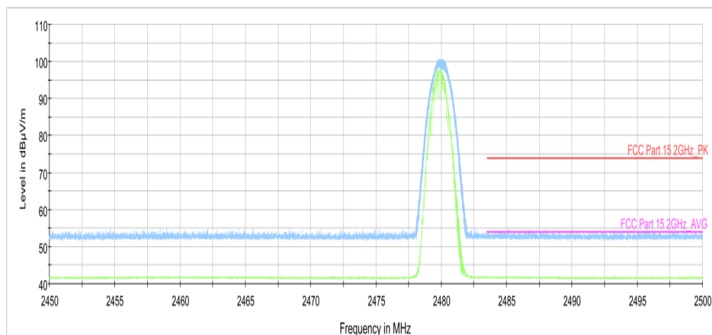
Fig.16. Frequency Band Edges: \pi/4 DQPSK, Channel 78, 2.45 GHz - 2.50GHz
