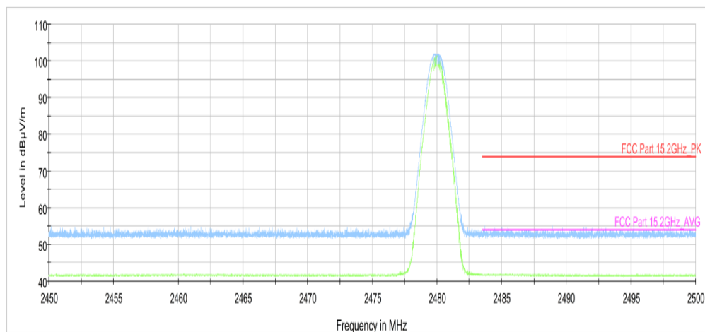
Fig.14. Frequency Band Edges: GFSK, Channel 78, 2.45 GHz - 2.50GHz
