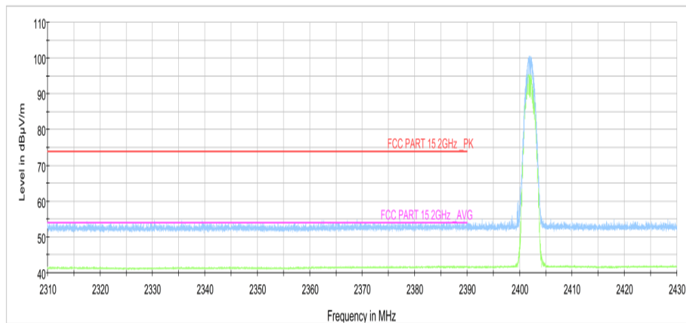
Fig.17. Frequency Band Edges: 8DPSK, Channel 0, 2.31 GHz - 2.43GHz
