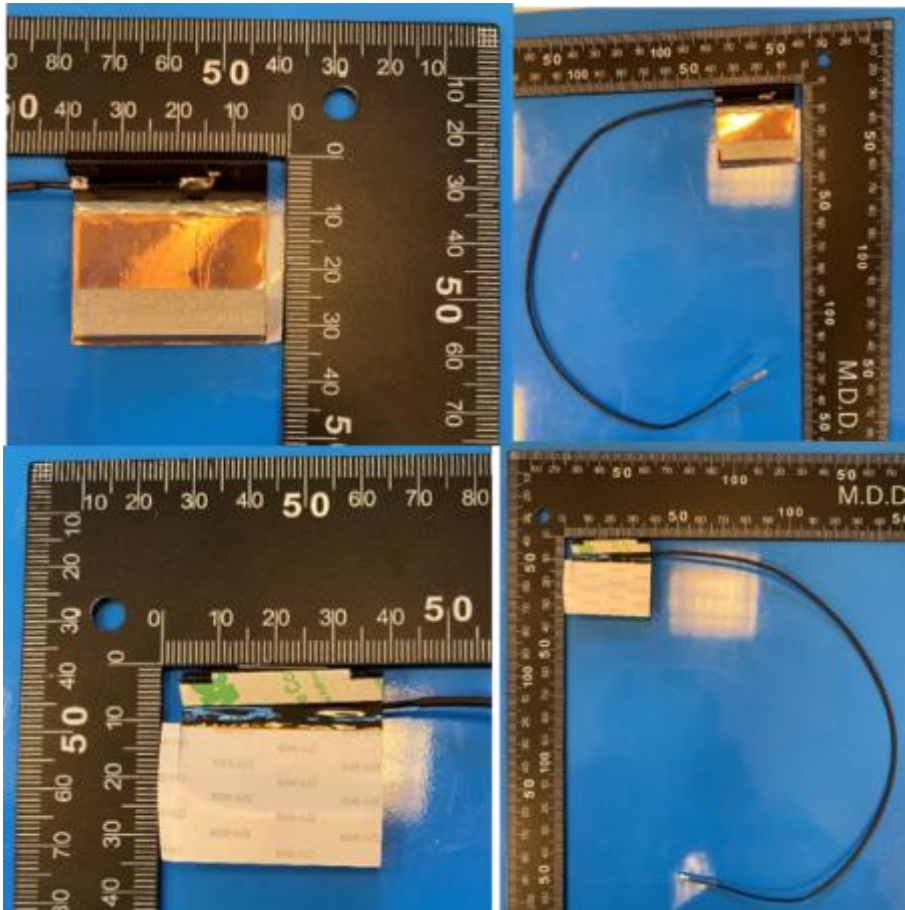
Main Antenna Photo (Front/Back): DC33002Q900((TZ2283D)
