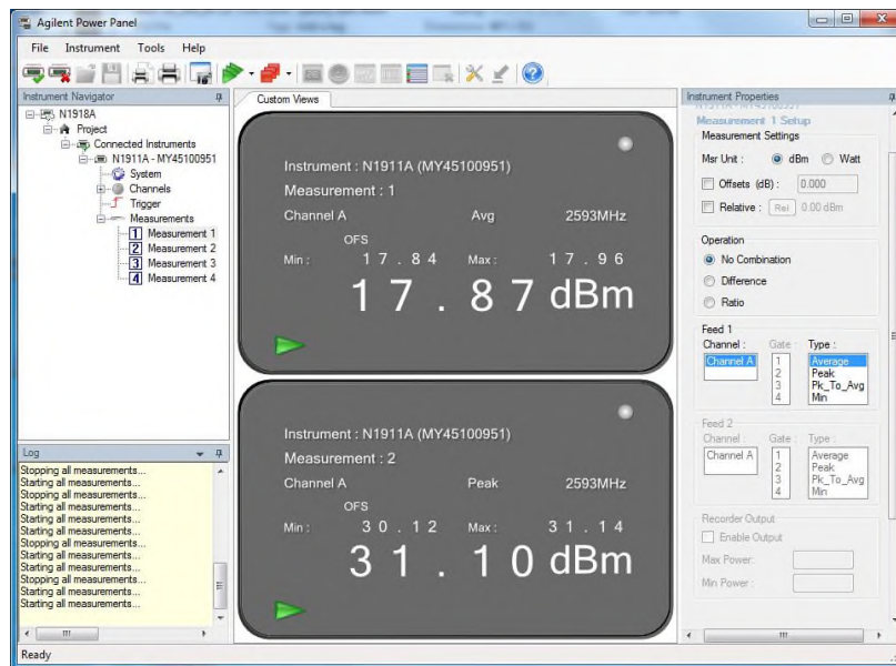
LTE Band 41 UL 10MHz Bandwidth Middle Channel
