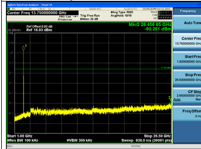
OQPSK on Channel 25
