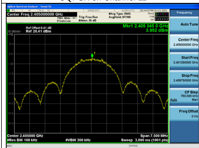
OQPSK on Channel 11
