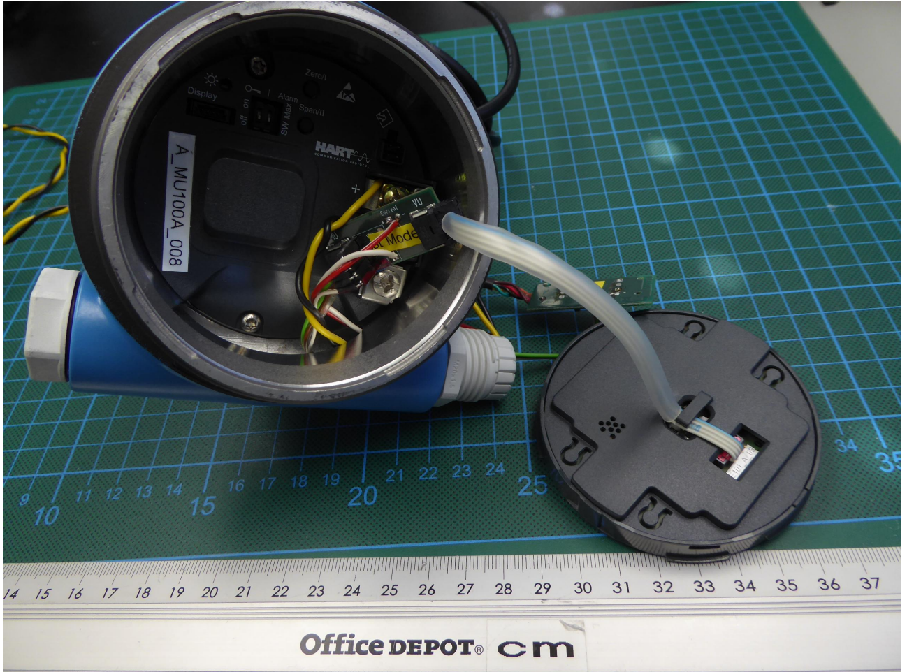
Housing open 1
