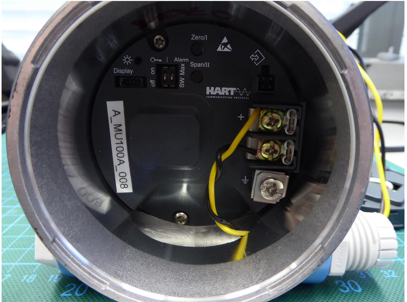
Housing open 2
