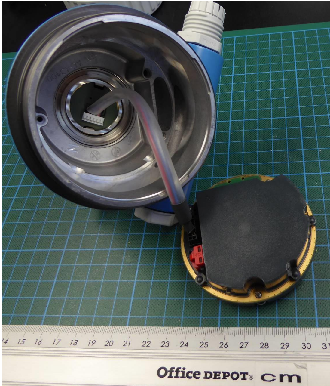
Housing open 4
