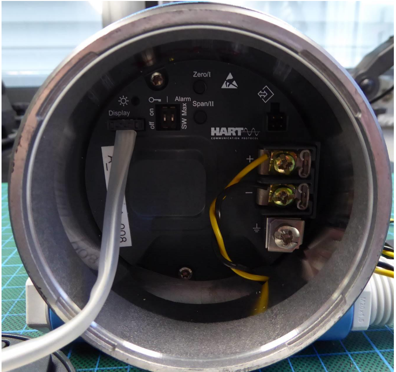
Housing open 3
