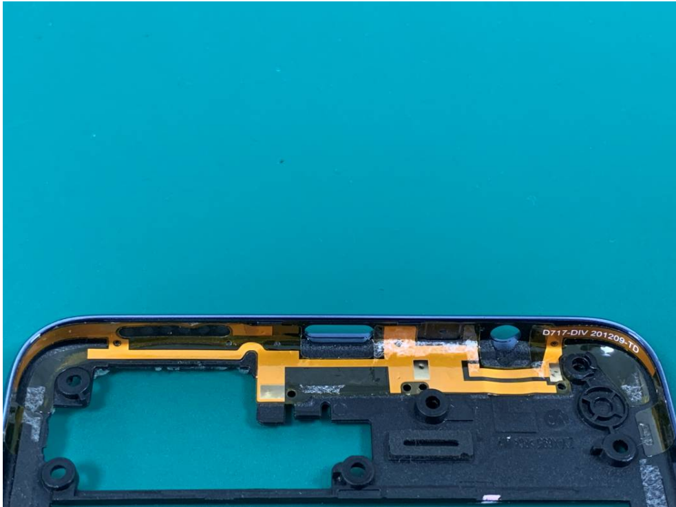
LTE Aux Antenna
