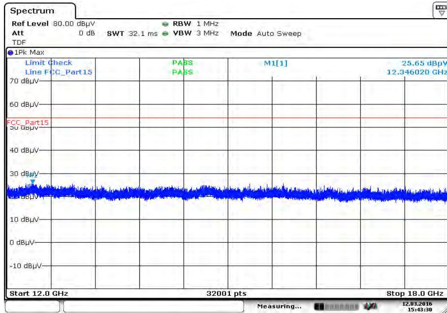
Plot 22: 12 GHz to 18 GHz, 5320 MHz, vertical & horizontal polarization
