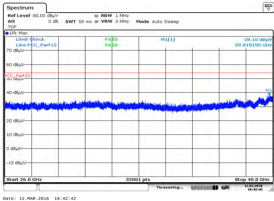
Plot 30: 26 GHz to 40 GHz, 5510 MHz, vertical & horizontal polarization
