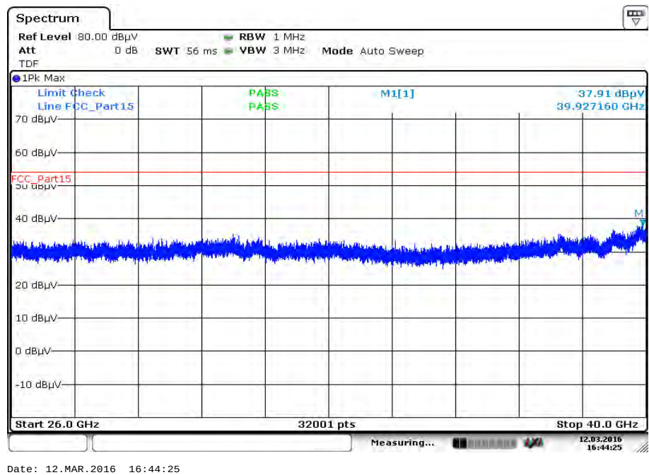
Plot 42: 26 GHz to 40 GHz, 5755 MHz, vertical & horizontal polarization
