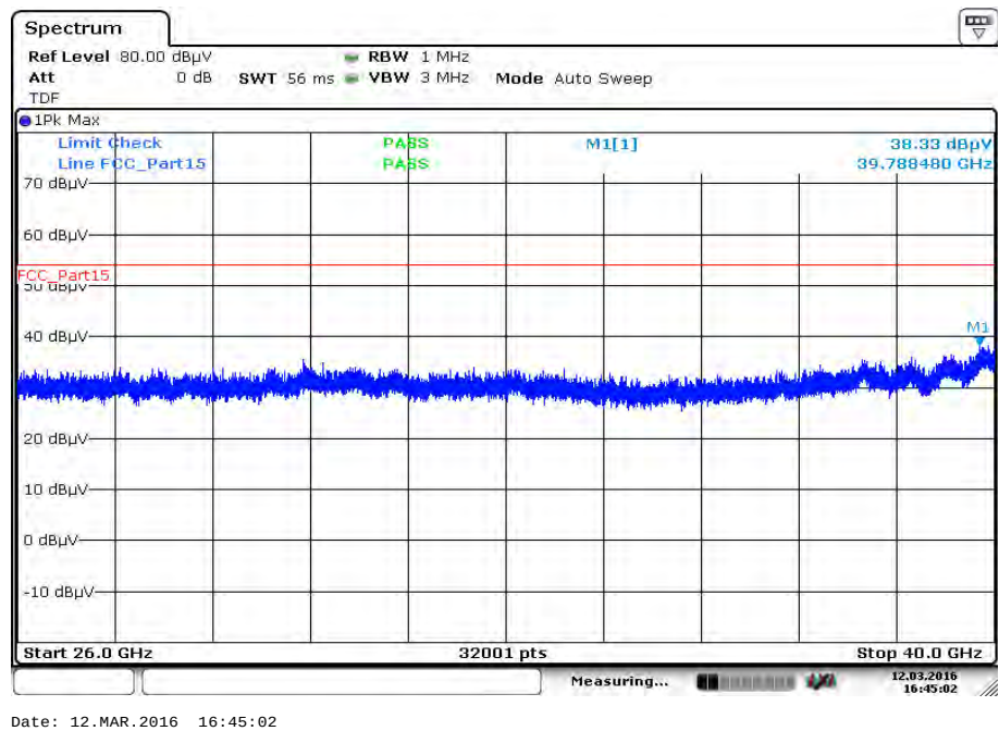
Plot 48: 26 GHz to 40 GHz, 5795 MHz, vertical & horizontal polarization
