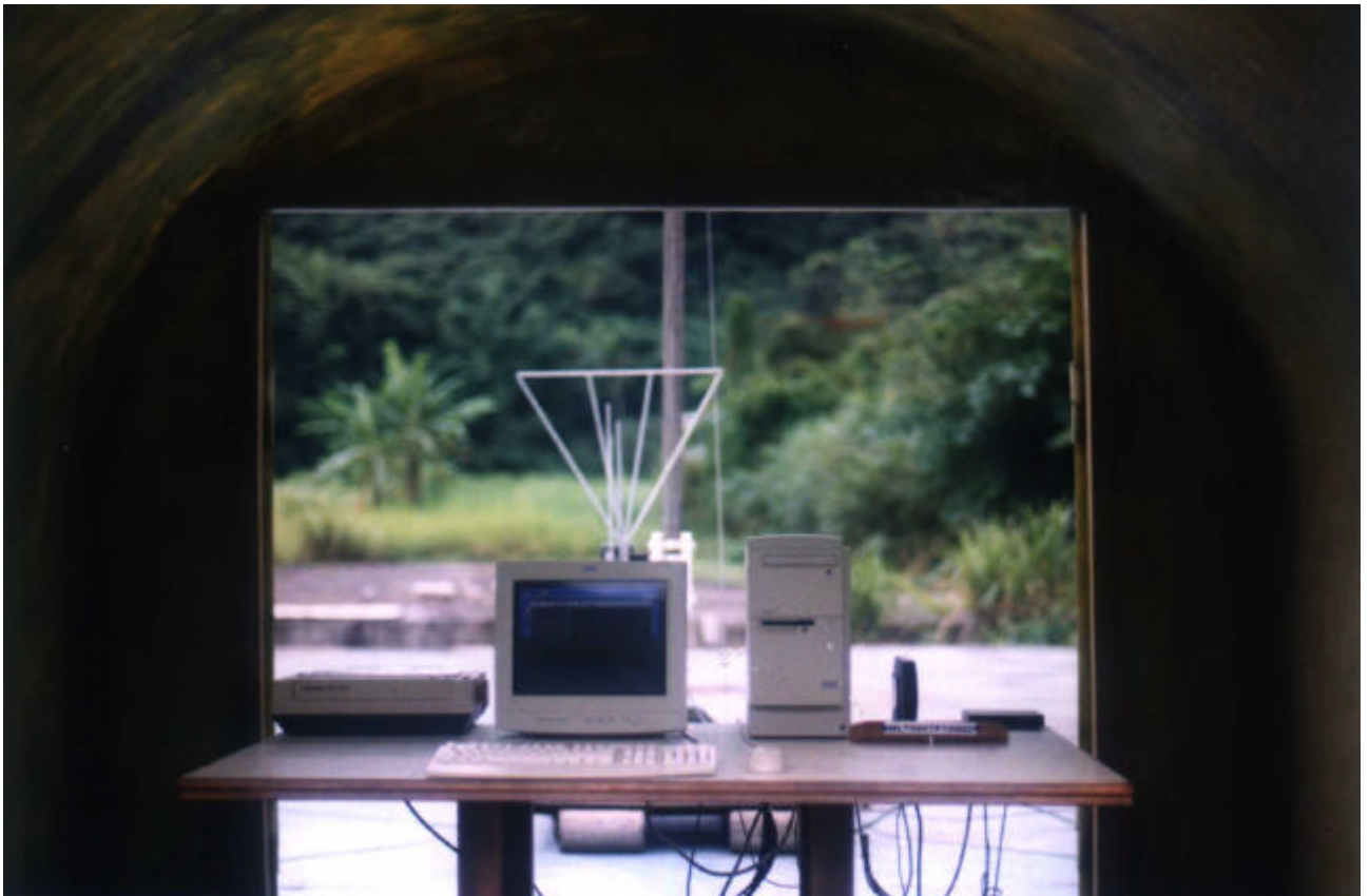
Front View of The Test Configuration
