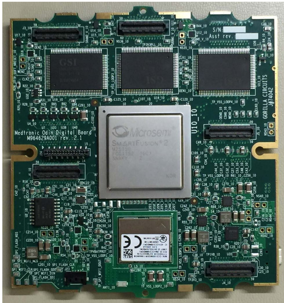
Figure 1: External Neurostimulator, Model: 4NR003, Digital Board Top View
