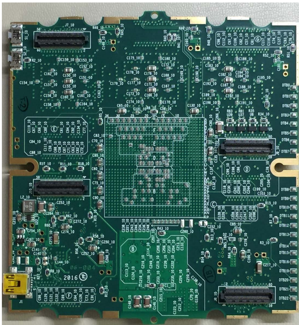
Figure 2: External Neurostimulator, Model: 4NR003, Digital Board Back View
