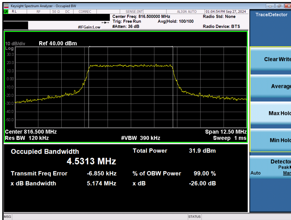
Plot 7-23. Occupied Bandwidth Plot (LTE Band 26 - 5MHz QPSK Low Channel- Full RB)
