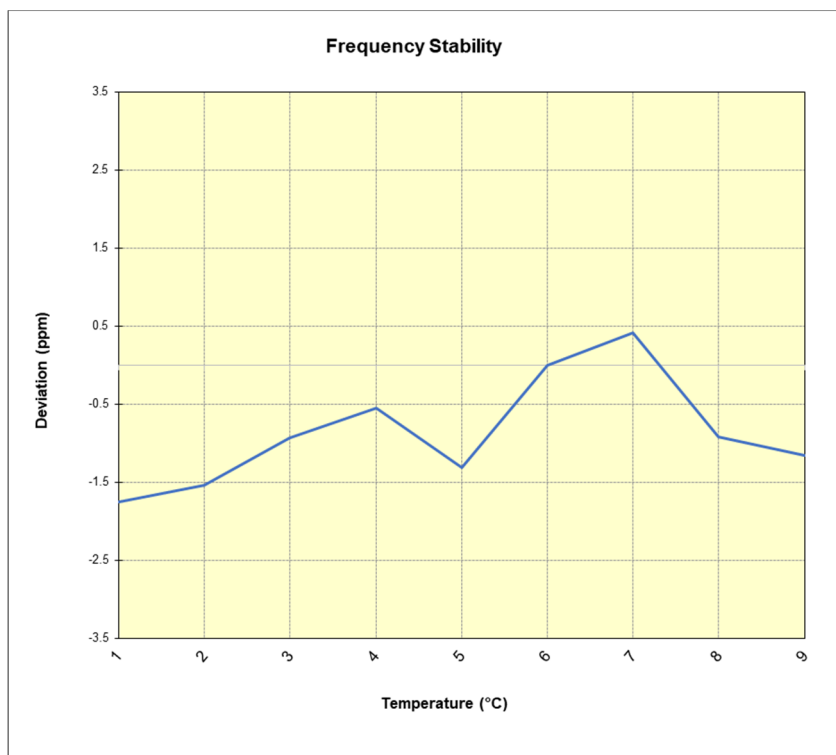
Plot 7-51. LTE Band 26 Frequency Stability Chart
