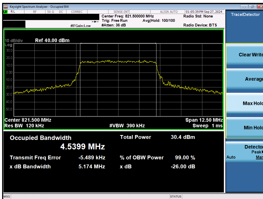
Plot 7-26. Occupied Bandwidth Plot (LTE Band 26 - 5MHz 16-QAM High Channel - Full RB)
