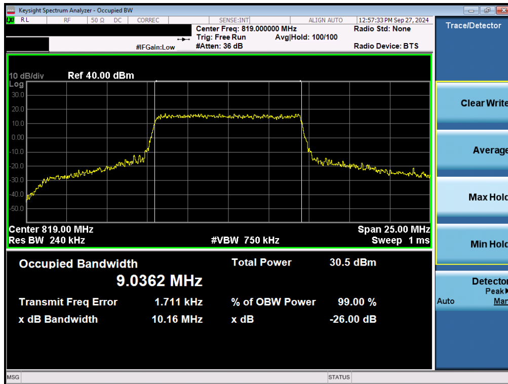
Plot 7-22. Occupied Bandwidth Plot (LTE Band 26 - 10MHz 16-QAM - Full RB)
