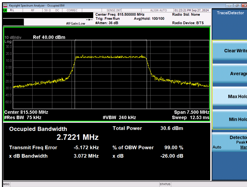
Plot 7-29. Occupied Bandwidth Plot (LTE Band 26 - 3MHz 16-QAM Low Channel - Full RB)
