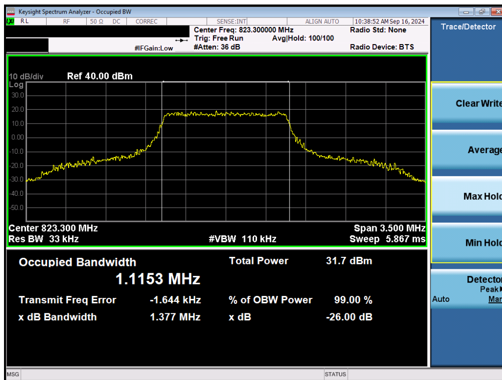
Plot 7-14. Occupied Bandwidth Plot (LTE Band 26 – 1.4MHz 16-QAM High Channel - Full RB)
