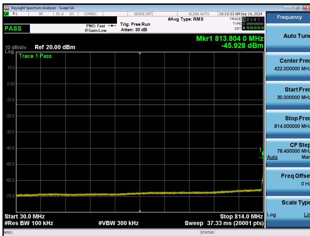
Plot 7-37. Conducted Spurious Plot (LTE Band 26 - 15MHz QPSK - RB Size 1, RB Offset 37)
