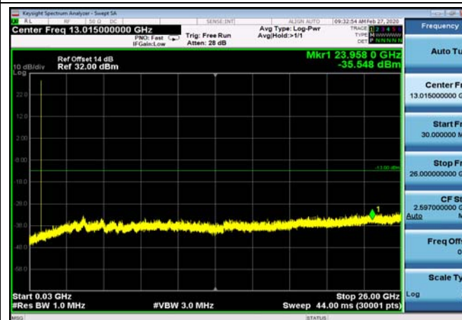
FDD05_LowRange_1.4MHz_30MHz~26GHz
