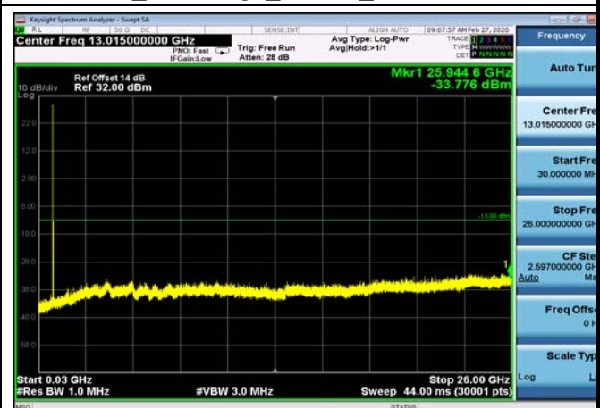
FDD05_LowRange_10MHz_30MHz~26GHz
