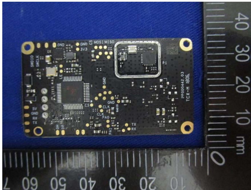
EUT –Wireless Module RF Board Bottom Uncover View
