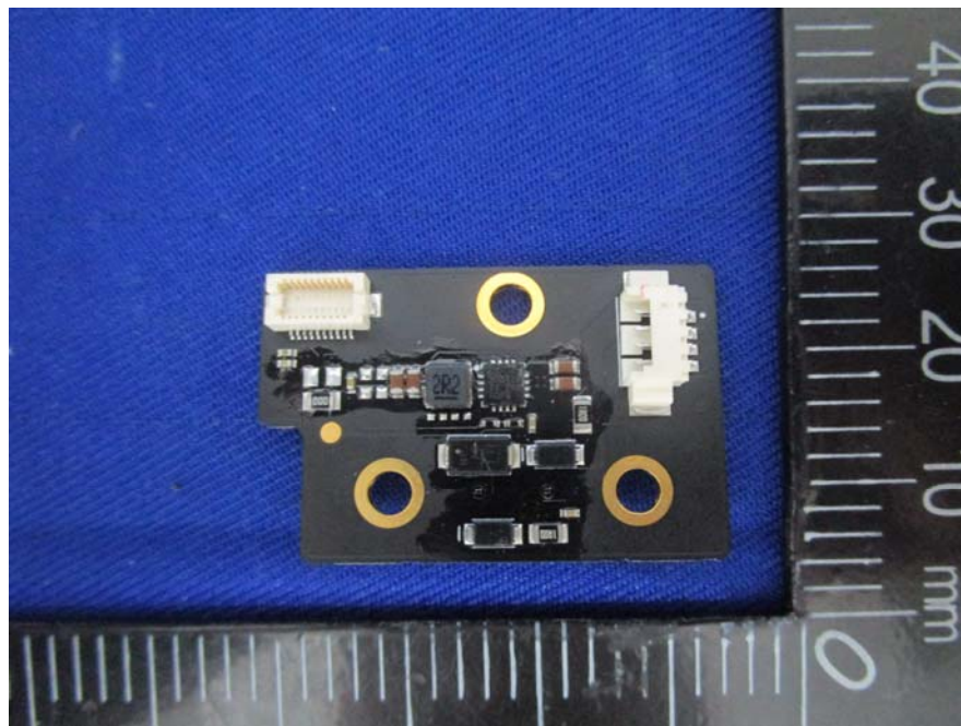
EUT –Wireless Module Sub-Board Top View
