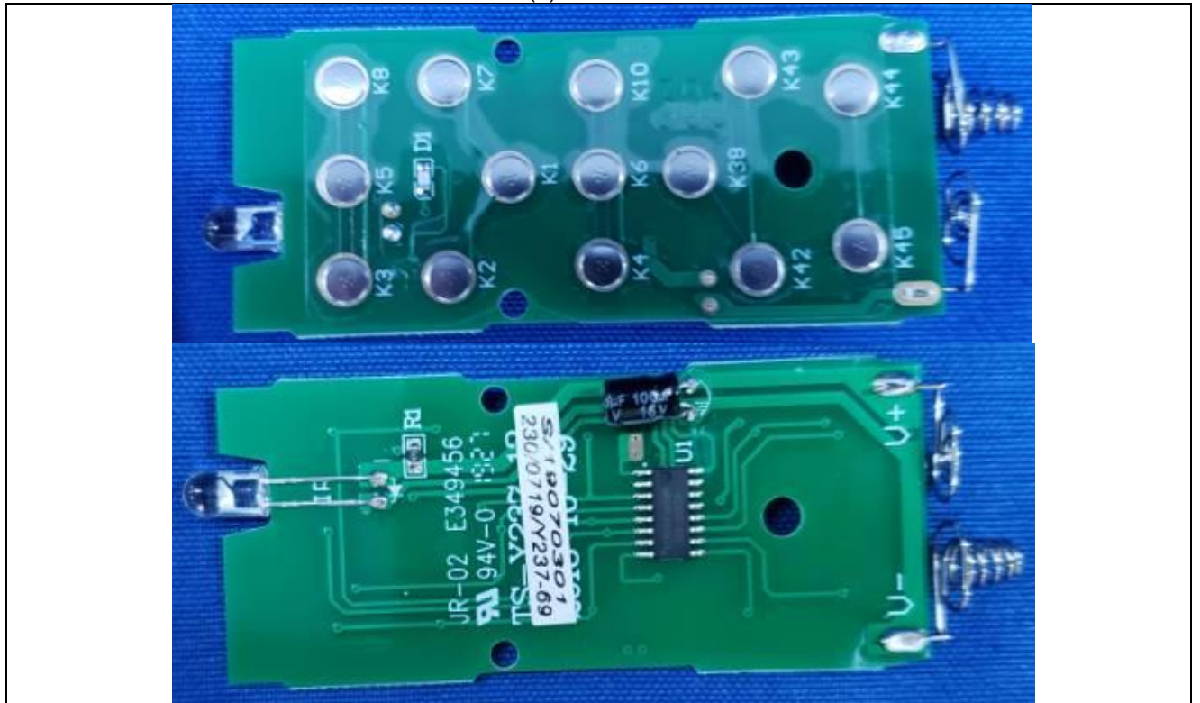
Details of: Accessory Internal view of remote controller (2)
