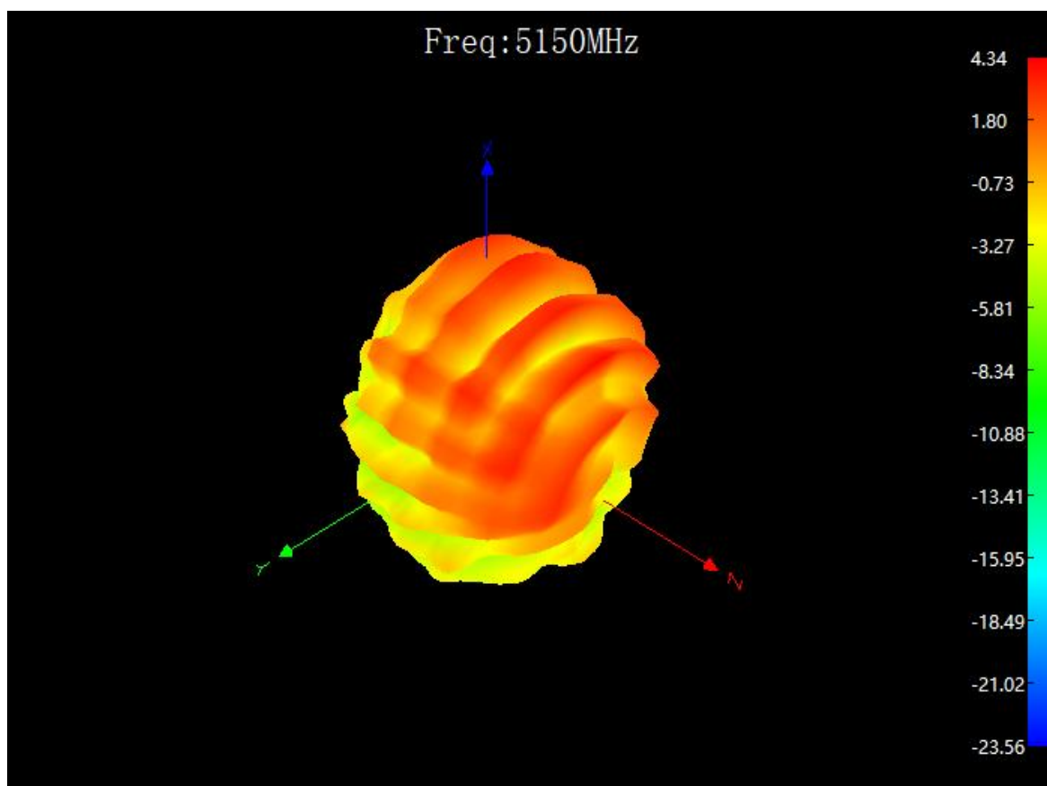
Wifi antenna 3D diagram
