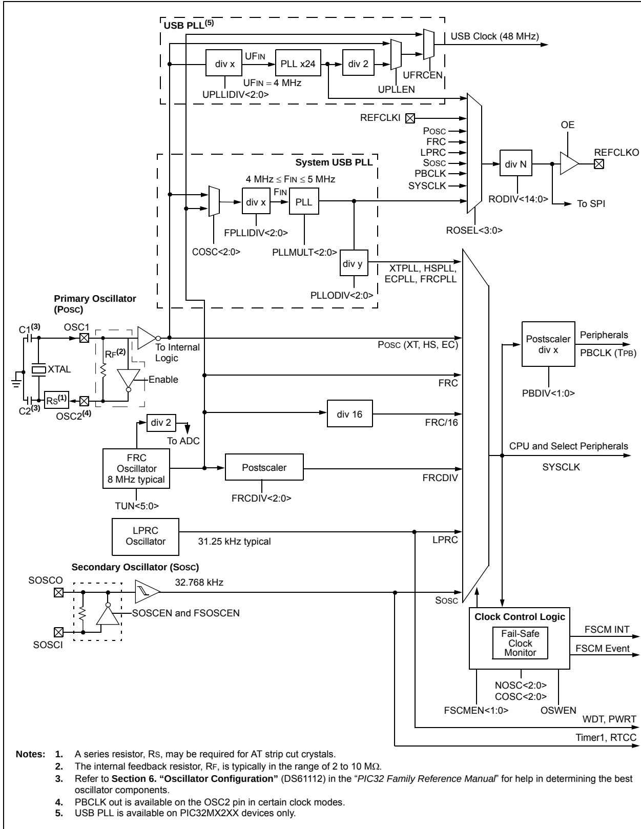
FIGURE 8-1: PIC32MX1XX/2XX FAMILY CLOCK DIAGRAM
