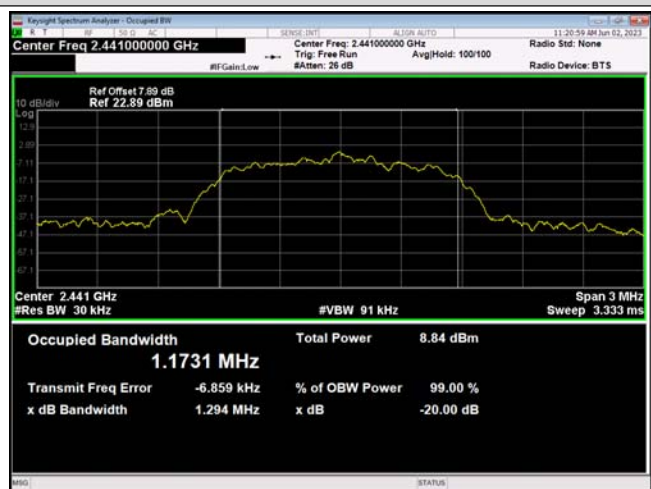
8DPSK_3-DH1_Channel 39
