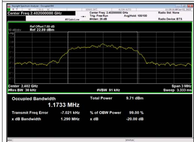
8DPSK_3-DH1_Channel 0
