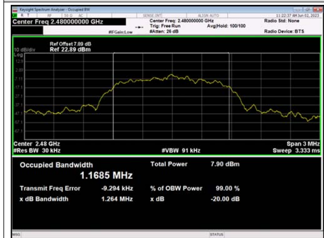
8DPSK_3-DH1_Channel 78
