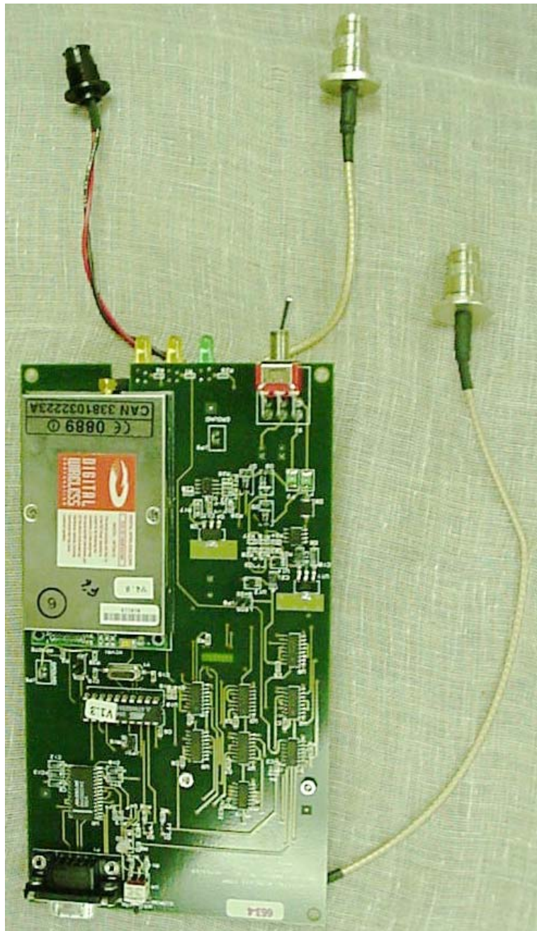
Photo 4. EUT, Top View of PCB
