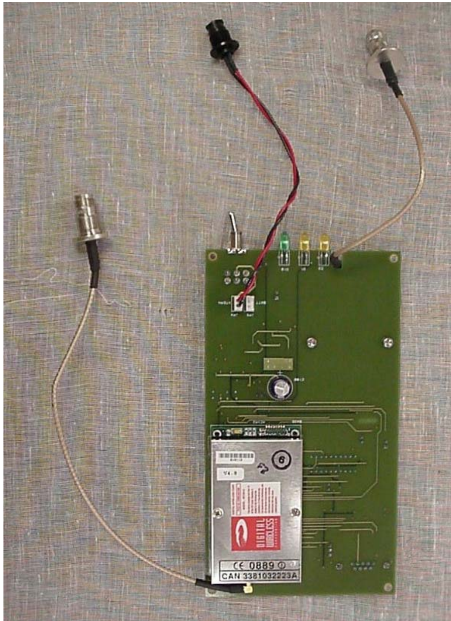
Photo 5. EUT, Bottom View of PCB
