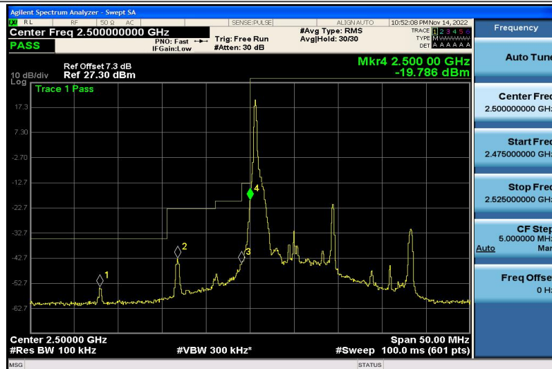
Band7-10MHz-16QAM-20800-1RB#0
