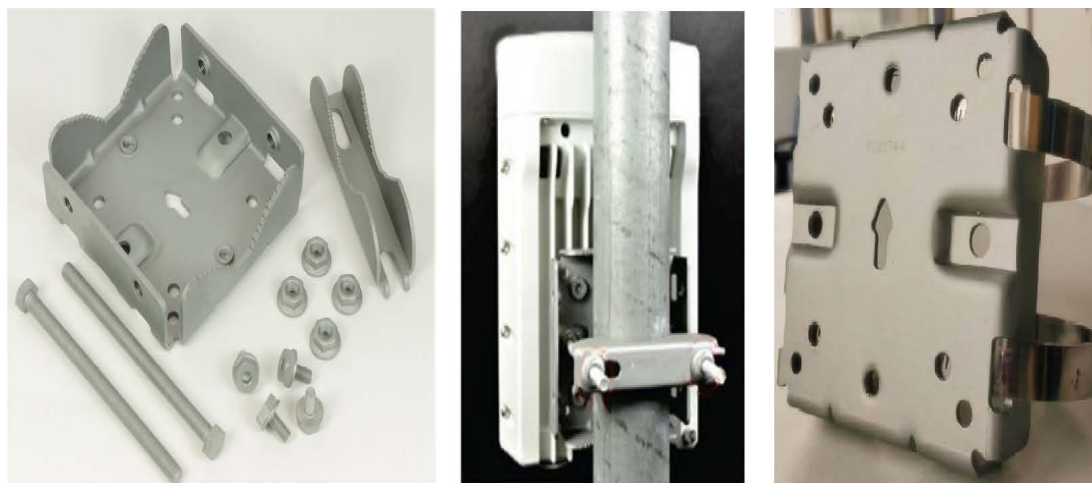
Figure 24: Pole mount
