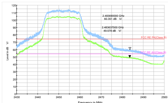
802.11g-Channel 9 Peak+ Average
