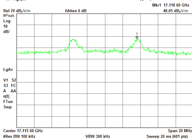
Plot 7.3.98 Radiated emission measurements at the seventh harmonic of high carrier frequency, Antenna 2
