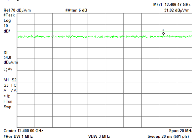
Plot 7.3.56 Radiated emission measurements at the sixth harmonic of low carrier frequency, Antenna 1
