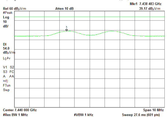
Plot 7.3.84 Radiated emission measurements at the fourth harmonic of low carrier frequency, Antenna 2
