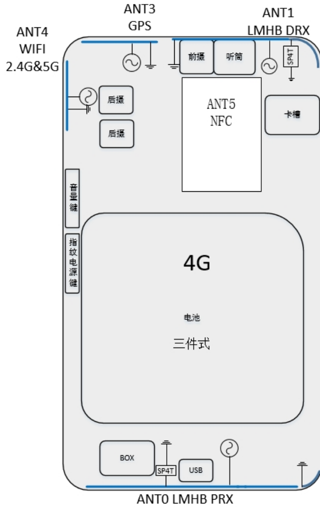
Fig 1 Antenna location &amp; dimension
