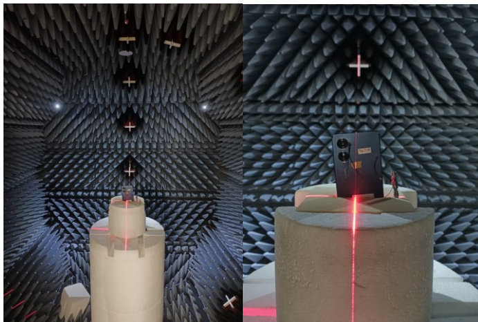
Fig.5. The DUT in the fully anechoic chamber
