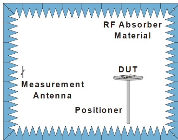
Fig. 4. The fully anechoic chamber
