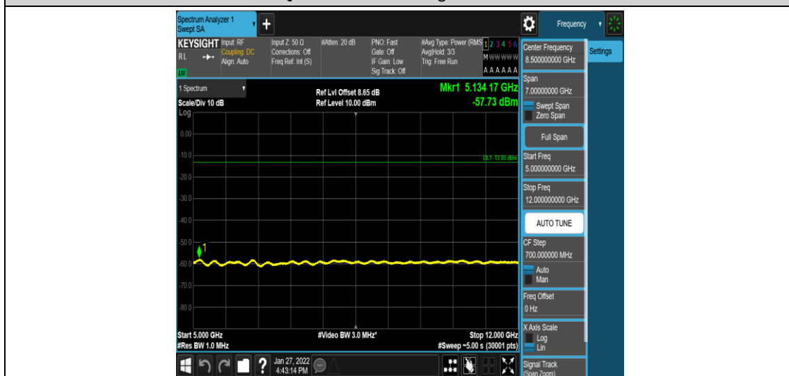
Band4-15MHz-16QAM-20325-1-0-High-5000-12000--57.73-PASS
