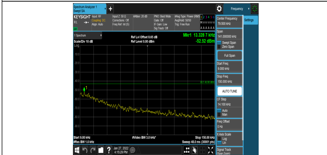
Band4-10MHz-16QAM-20350-1-0-High-0.009-0.15--52.52-PASS
