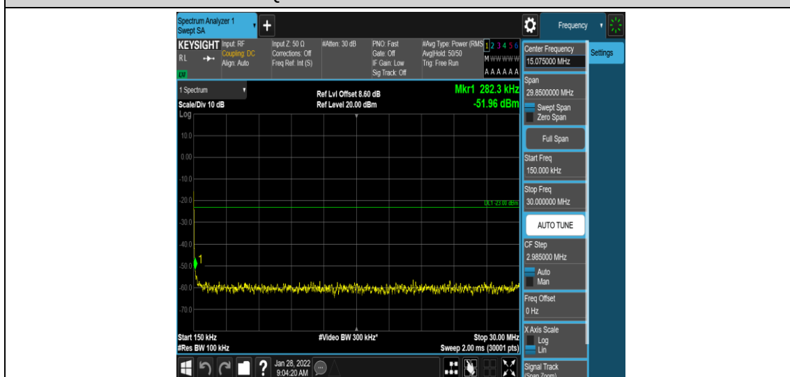
Band4-20MHz-QPSK-20175-1-0-Low-0.15-30--51.96-PASS
