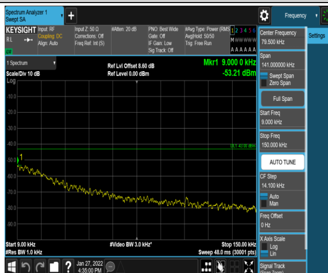
Band4-15MHz-QPSK-20025-1-0-Low-0.009-0.15--53.21-PASS
