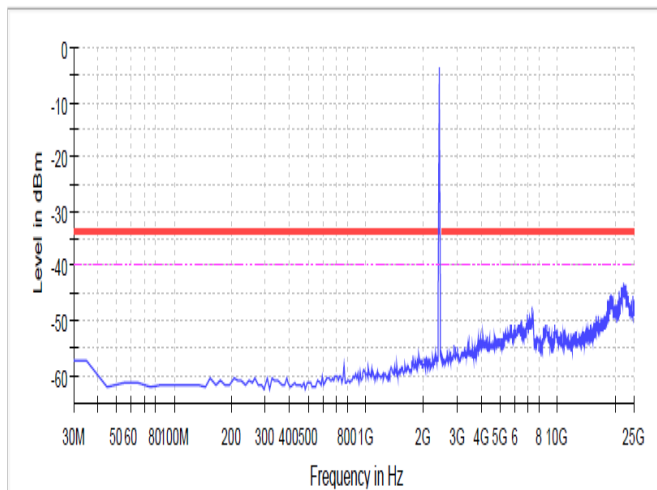
Spurious
