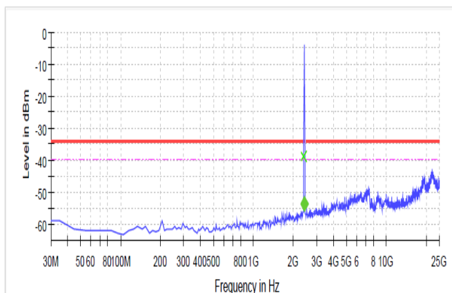
Spurious
