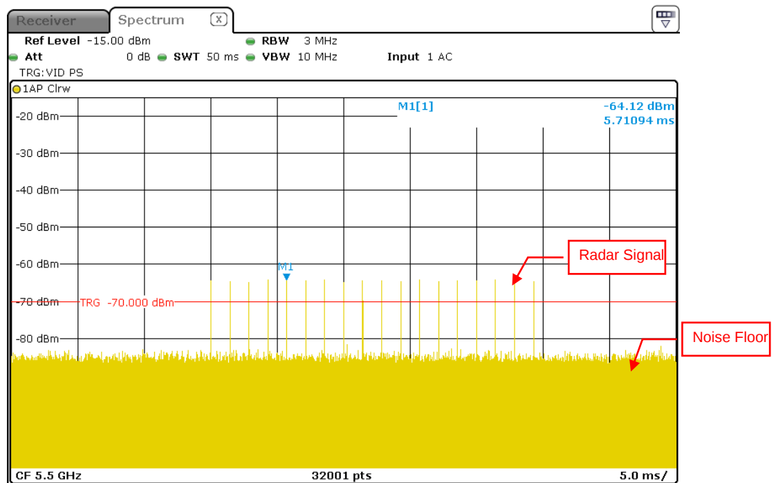
Radar Signal 0
