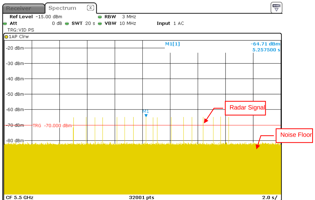
Radar Signal 5
