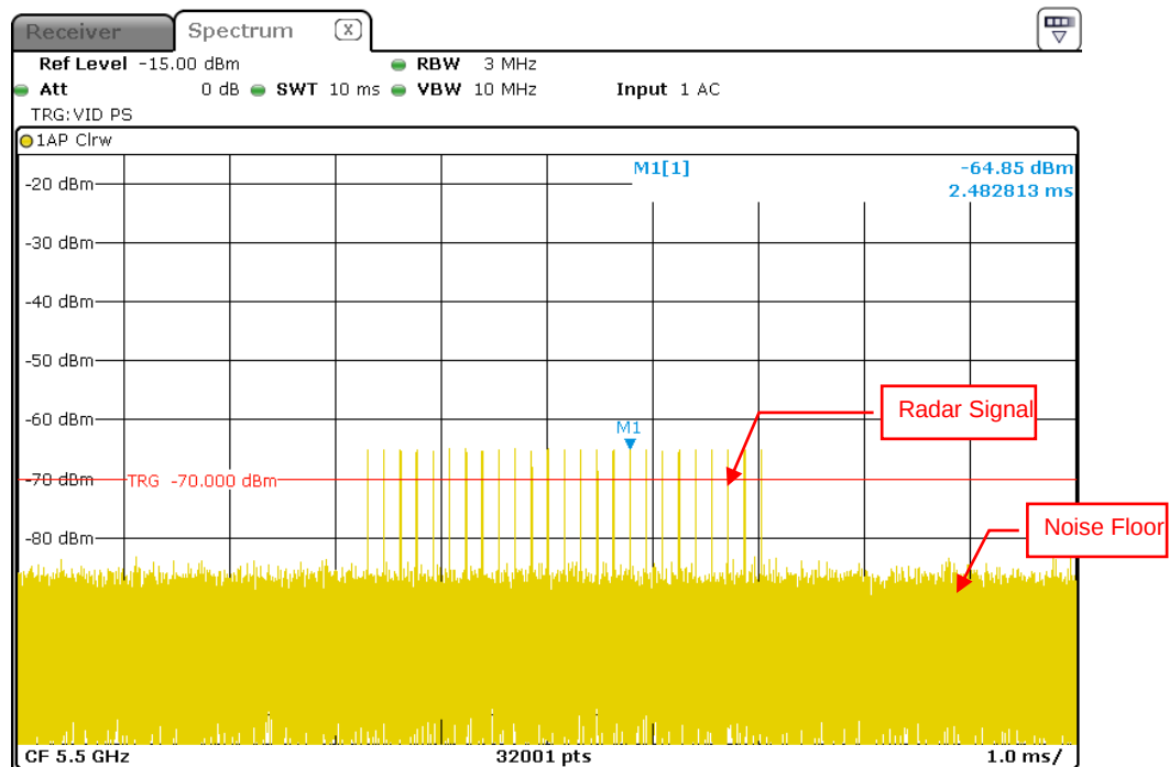
Radar Signal 2
