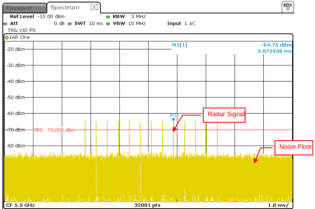
Radar Signal 4
